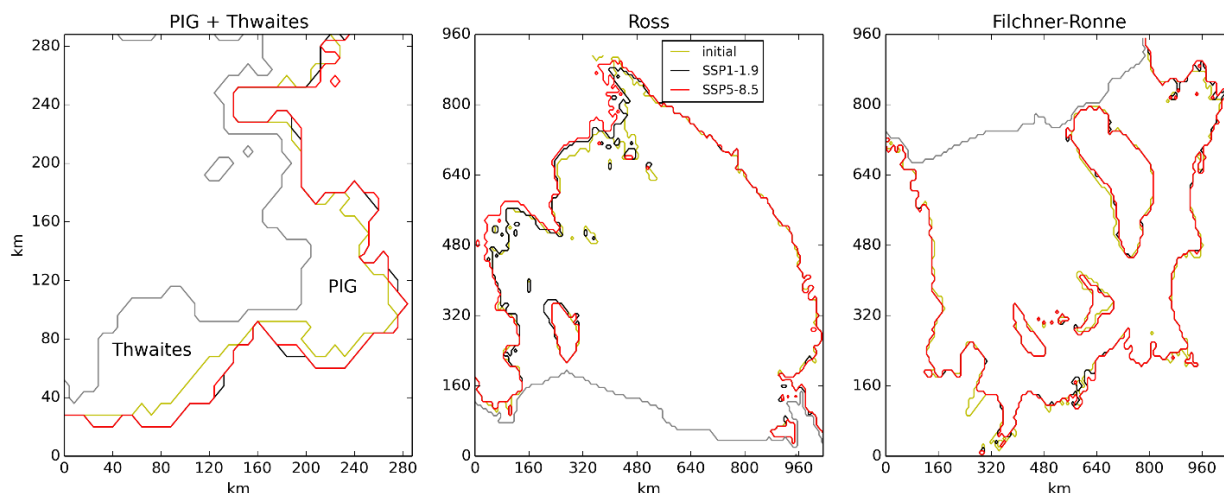
755 Figure 17: Grounding line change in (Left) Pine Island & Thwaites Glaciers (Middle) Ross and (Right) Filchner-Ronne ice shelves. Gray=ice front, yellow=initial grounding line, black=grounding line for SSP1-1.9 in 2100, red=grounding line for SSP5-8.5 in 2100.
