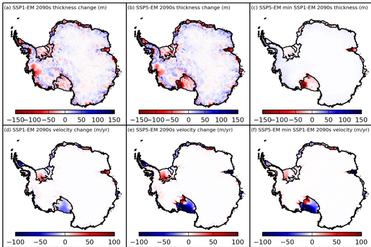
Figure 15: Change of (top) ice thickness and (bottom) surface velocity magnitude between (Left) 2015 and 2100 in SSP1-1.9 (Middle) 2015 and 2100 in SSP5-8.5. (Right) Difference of (top) ice thickness and (bottom) surface velocity magnitude in the final period between SSP5-8.5 and SSP1-1.9.
