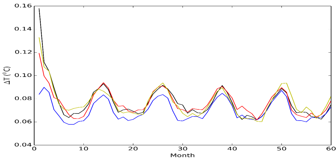
295 Figure 2: Monthly time-series of temperature difference across ice fronts averaged over depth and along the entire Antarctic coast in the first 5 years of ocean stand-alone integration (Stage C) for all (four) members. The blue line is the member that was not initialised with the global ocean from the UKESM1.0 CMIP6 historical ensemble.
