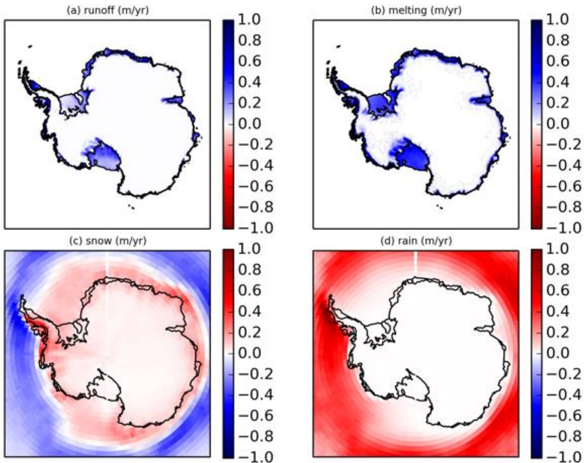
675 Figure 14: The difference between average 2090-2100 and average 2020-2030 of SMB components in SSP5-8.5: (a) surface runoff (b) surface melting (c) snowfall and (d) rainfall, all in m/yr. Black lines indicate the grounding lines of the ice sheet.
