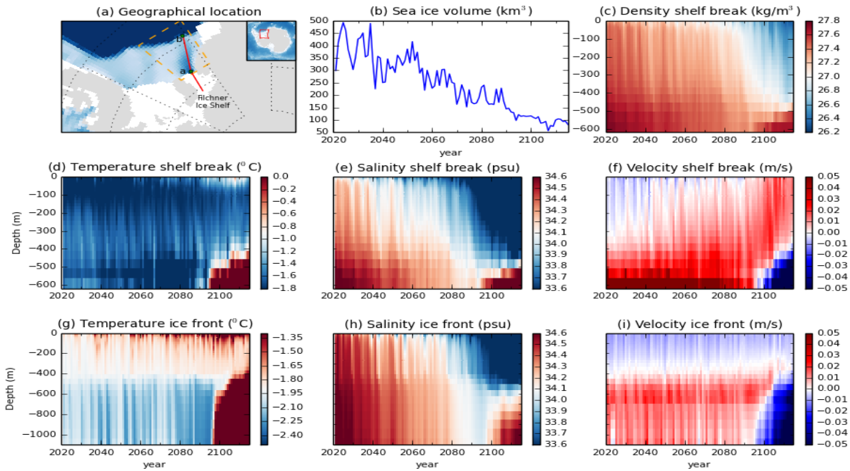
Figure 8: Filchner Trough profiles in the SSP5-8.5 scenario. (a) The chosen section on the Filchner Trough is indicated by the red line segment between the green dots a and b. The entire red line denotes the meridional section used in Figure 9. The dark and light blue colours represent the deep ocean and the continental shelf in the Weddell Sea, respectively, whereas the grey and white colours represent the grounded ice sheet and the Filchner-Ronne Ice Shelf, respectively. (b) sea ice volume on the area enclosed by the orange dashed lines in (a). (c-f) The timeseries of potential density, temperature, salinity and meridional velocity, respectively at the shelf break indicated by the green dot b in (a). (g-i) The timeseries of temperature, salinity and meridional velocity at the ice front indicated by the green dot a in (a).
