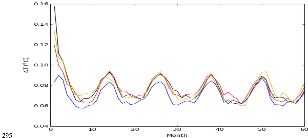
295 Figure 2: Monthly time-series of temperature difference across ice fronts averaged over depth and along the entire Antarctic coast in the first 5 years of ocean stand-alone integration (Stage C) for all (four) members. The blue line is the member that was not initialised with the global ocean from the UKESM1.0 CMIP6 historical ensemble.
