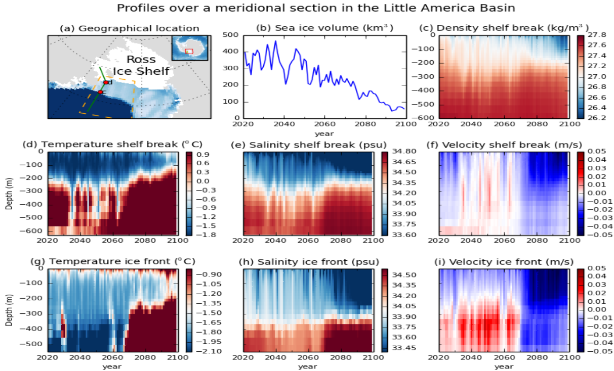
555 Figure 10: Little America Basin profile in the SSP5-8.5 scenario. (a) The chosen section on the Little America Basin is indicated by the green line segment between the red dots c and d. The entire green line denotes the meridional section used in Figure 11. The dark and light blue colours represent the deep ocean and the continental shelf in the Ross Sea, respectively, whereas the grey and white colours represent the grounded ice sheet and the Ross Ice Shelf, respectively. (b) Sea ice volume on the area enclosed by the 560 orange dashed lines in (a). (c-f) The timeseries of potential density, temperature, salinity and meridional velocity, respectively at the shelf break indicated by the red dot c in (a). (g-i) The timeseries of temperature, salinity and meridional velocity at the ice front indicated by the red dot d in (a).
