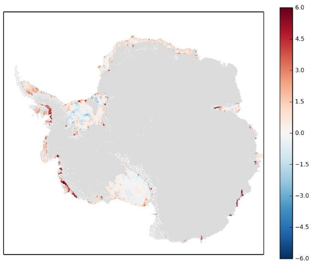
960 Figure A1. Ice shelf basal melt rate observation (m/yr) around Antarctica (Adusumilli et al., 2020).
