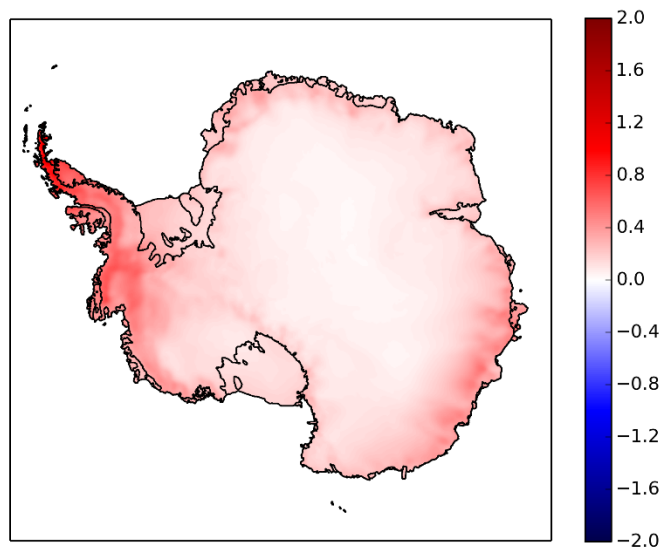
Figure A2. Surface Mass Balance interpolated from observation (m/yr) around Antarctica (Arthern et al.,2006).
