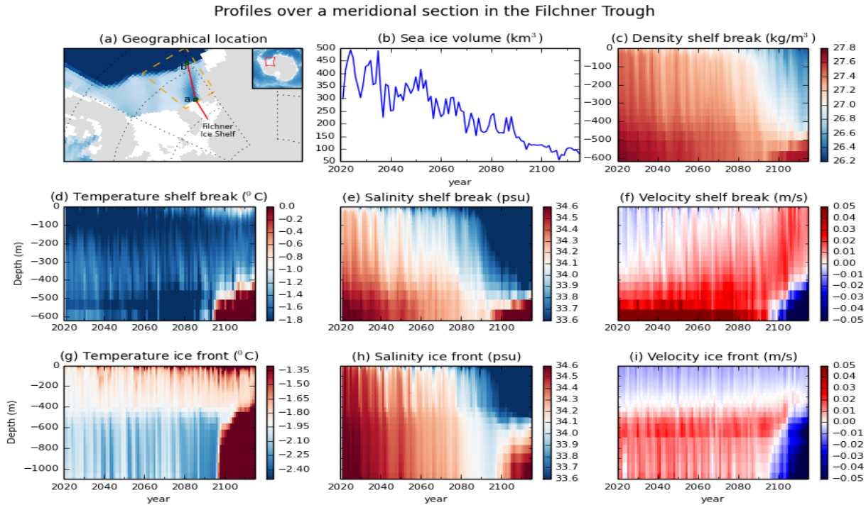
Figure 8: Filchner Trough profiles in the SSP5-8.5 scenario. (a) The chosen section on the Filchner Trough is indicated by the red line segment between the green dots a and b. The entire red line denotes the meridional section used in Figure 9. The dark and light blue colours represent the deep ocean and the continental shelf in the Weddell Sea, respectively, whereas the grey and white colours represent the grounded ice sheet and the Filchner-Ronne Ice Shelf, respectively. (b) sea ice volume on the area enclosed by the orange dashed lines in (a). (c-f) The timeseries of potential density, temperature, salinity and meridional velocity, respectively at the shelf break indicated by the green dot b in (a). (g-i) The timeseries of temperature, salinity and meridional velocity at the ice front indicated by the green dot a in (a).
