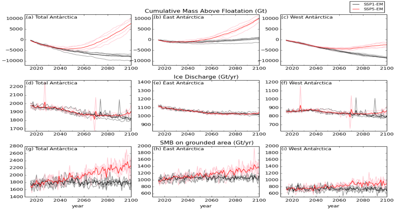
Figure 16: Time-series of ice mass budget. Top row: cumulative anomaly of ice mass above flotation relative to the initial condition; middle: rate of discharge across grounding lines; bottom row: SMB rate on the grounded ice. The grey, black, pink and red lines represent the SSP1-1.9 ensemble members, SSP1-1.9 ensemble mean, SSP5-8.5 ensemble members and SSP5-8.5 ensemble mean respectively. The Antarctic Peninsula region is considered part of West Antarctica. In each row (budget), the axis range is set the same for all columns (regions).
