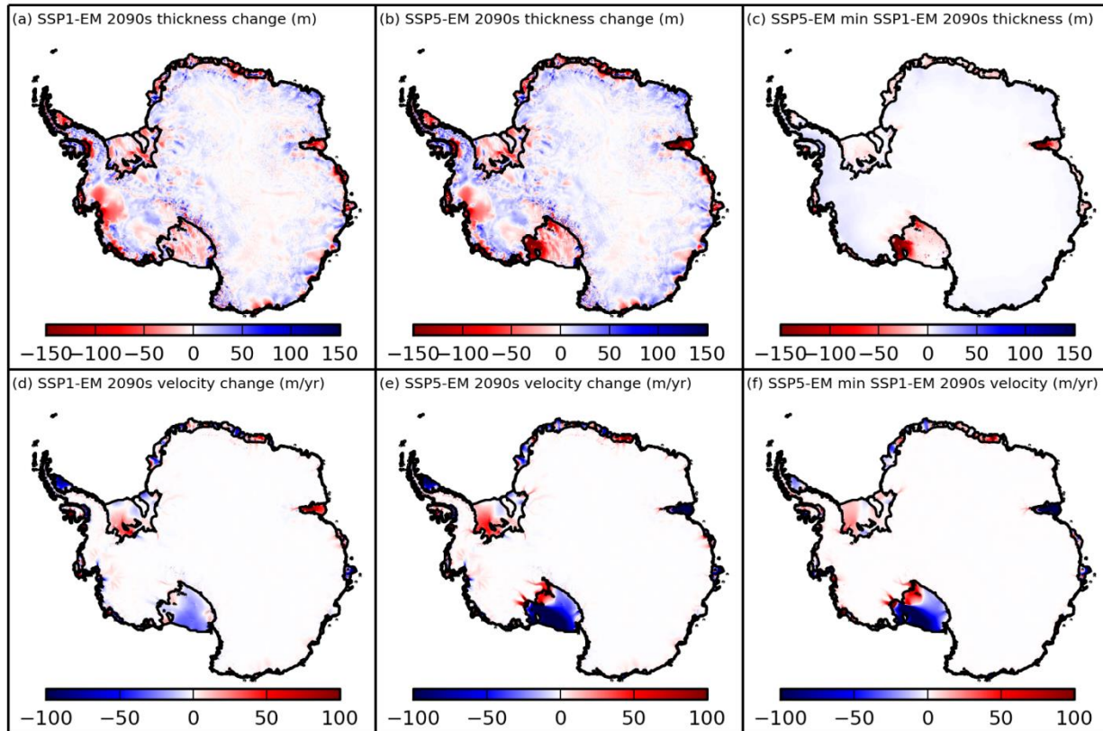
690 Figure 15: Change of (top) ice thickness and (bottom) surface velocity magnitude between (Left) 2015 and 2100 in SSP1-1.9 (Middle) 2015 and 2100 in SSP5-8.5. (Right) Difference of (top) ice thickness and (bottom) surface velocity magnitude in the final period between SSP5-8.5 and SSP1-1.9.
