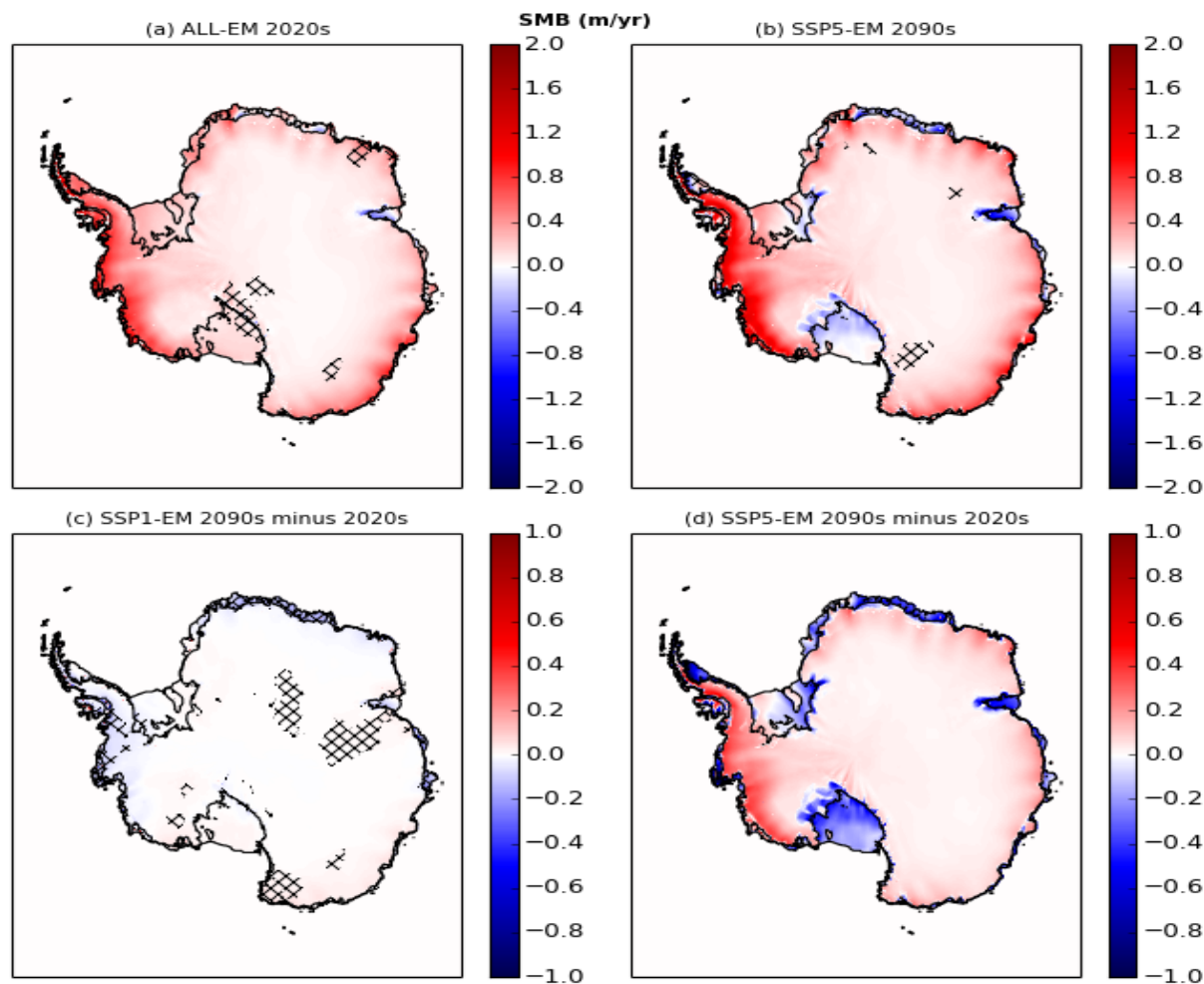
630 Figure 13: (a) ALL-EM SMB for period 2020-2030. Locations with statistically significant difference (95% Student's t -confidence interval) between SSP1-EM and SSP5-EM are hatched. (b) SSP5-EM SMB 2090-2100. Locations with statistically significant 635 difference (95% confidence interval with one-way ANOVA) among the ensemble members are hatched. (c) Difference of SSP1-EM SMB between 2090-2100 period and 2020-2030 period. Locations where the difference is statistically significant (95% Student's t -confidence interval) are hatched. (d) Difference of SSP1-EM SMB between 2090-2100 period and 2020-2030 period, almost everywhere is statistically significant. Black and grey lines indicate the ice sheet grounding lines and ice shelf fronts, respectively.
