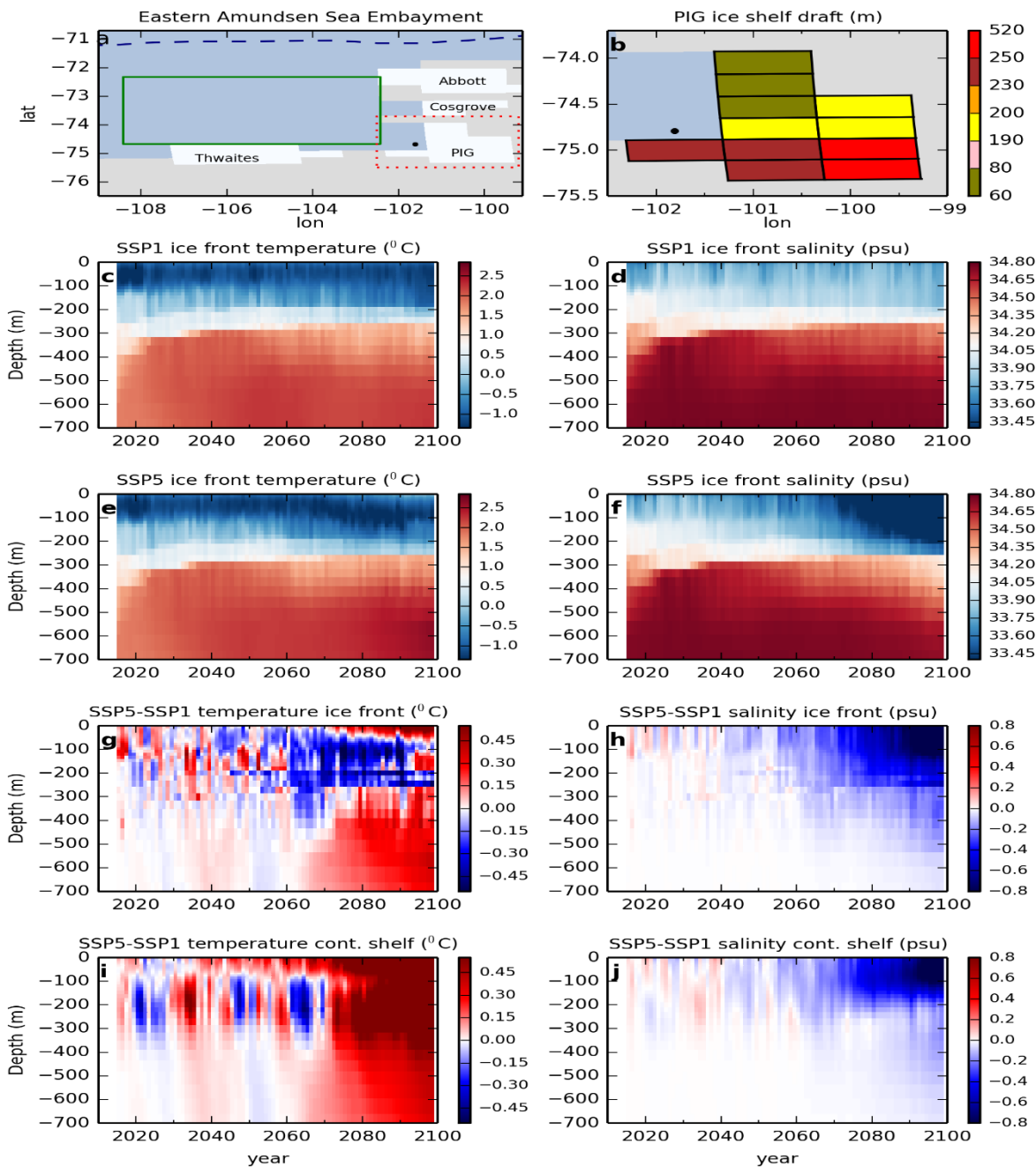
620 Figure 12: (a) The Amundsen Sea Embayment in the ORCA1 NEMO ocean model. Blue, grey, and white colour denote the ocean, grounded ice sheet, and ice shelf region. The dashed purple line marks the 700 m isobaths as the continental shelf edges. The black dot indicates the ice front where the time series profile in (c-h) is located. Enclosed by the green box is the continental shelf region where the horizontal average of time series profile in (i-j) is taken from. (b) The enlarged area surrounded by red dotted line in (a), but now with PIG Ice Shelf shaded with ice shelf draft colour scale. The draft is taken from the year 2080 of one SSP5-8.5 ensemble member. (c-h) Time-series at the PIG ice front of temperature and salinity: (c-d) SSP1-1.9 ensemble mean; (e-f) SSP5-8.5 ensemble mean; (g-h) anomaly between SSP5-8.5 and SSP1-1.9 ensemble mean. (i-j) like (g-h) but for the horizontal average over the area bounded by the green box in (a). 625
