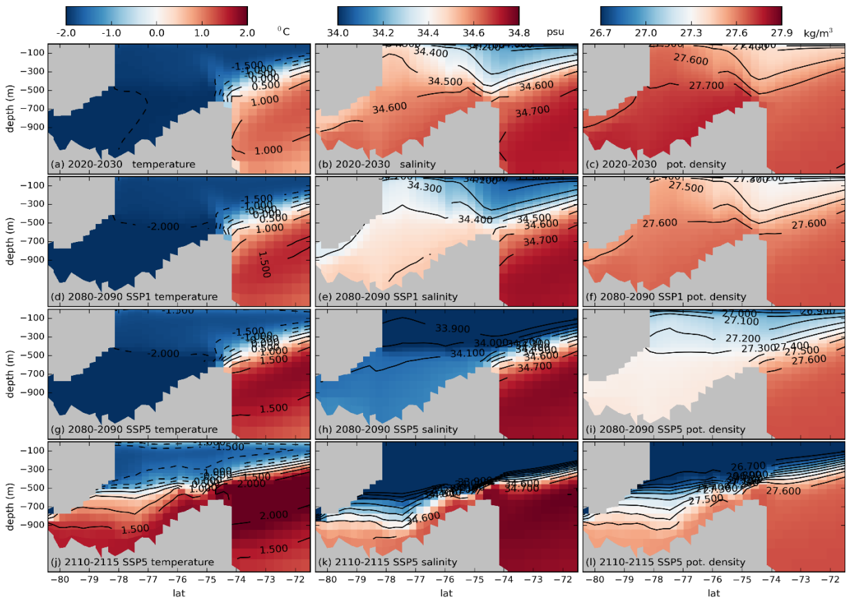
535 Figure 9: Temperature, salinity and potential density profile in a Filchner Trough section (indicated by the red line in Fig. 8a) for: (a,b,c) SSP5-8.5 year 2020-2030, (d,e,f) SSP1-1.9 year 2080-2090, (g,h,i) SSP5-8.5 year 2080-2090, (j,k,l) SSP5-8.5 year 2110-2115.
