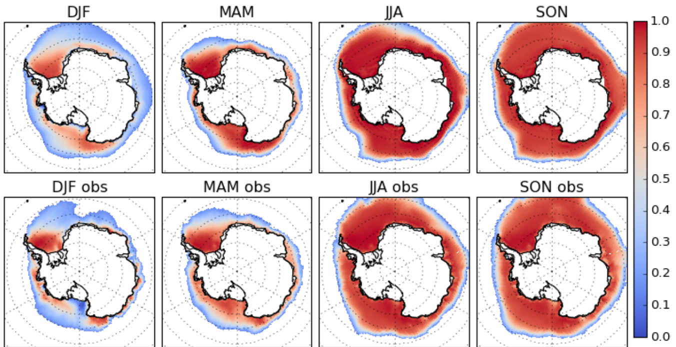
390 Figure 4: 2020-2030 ALL-EM (top) and HadISST1 (bottom) fractional sea-ice concentration in each season. The extent is defined by a threshold 0.15 concentration.
