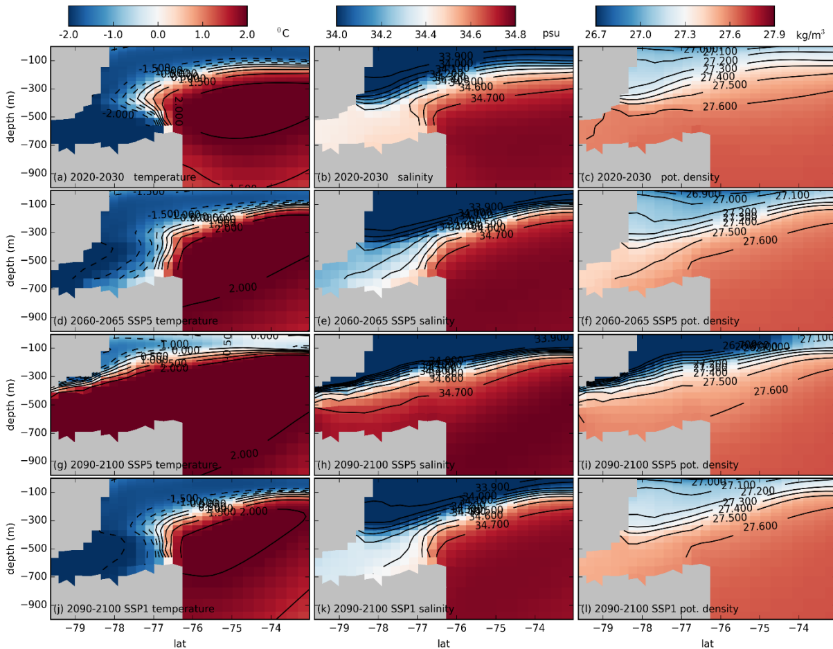
Figure 911: Temperature, salinity and potential density profile in a Little America Basin section (indicated by the green line in Fig. 8a10a) for: (a,b,c) SSP5-8.5 year 2020-2030, (d,e,f) SSP5-8.5 year 2060-2065, (g,h,i) SSP5-8.5 year 2090-2100, (j,k,l) SSP1-1.9 year 2090-2100.
