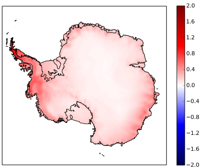
1105 Figure A2. Surface Mass Balance interpolated from observation (m/yr) around Antarctica (Arthern et al., 2006).
