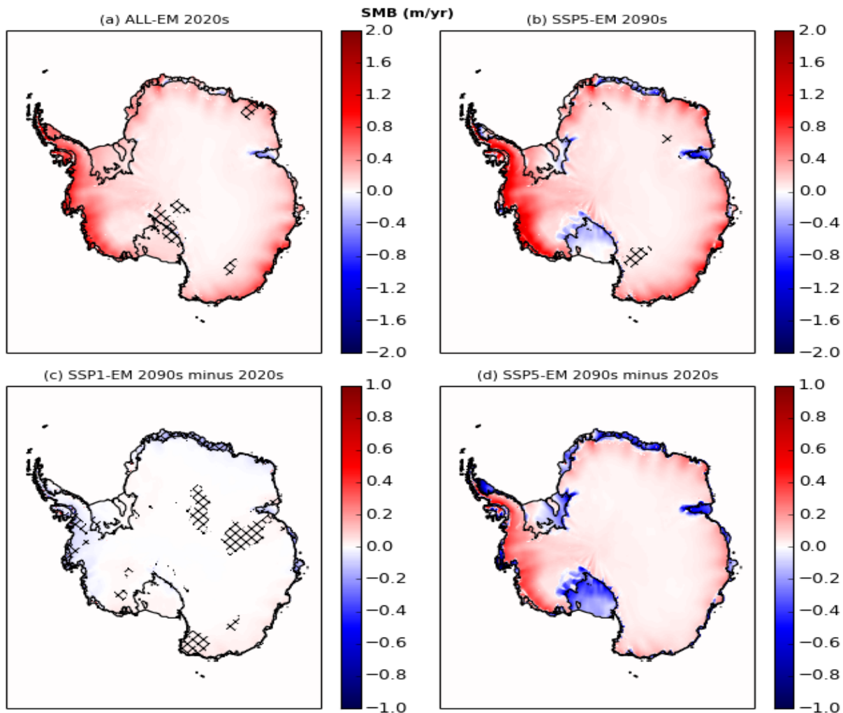
775 Figure 11: (a) ALL-EM SMB for period 2020–2030. Locations with statistically significant difference (95% Student’s t -confidence interval) between SSP1-EM and SSP5-EM are hatched. (b) SSP5-EM SMB 2090–2100. Locations with statistically significant difference (95% confidence interval with one-way ANOVA) among the ensemble members are hatched. (c) Difference of SSP1-EM SMB between 2090–2100 period and 2020–2030 period. Locations where the difference is statistically significant (95% Student’s t -confidence interval) are hatched. (d) Difference of SSP5-EM SMB between 2090–2100 period and 2020–2030 period, almost everywhere is statistically significant. Black and grey lines indicate the ice sheet grounding lines and ice shelf fronts, respectively. 780
