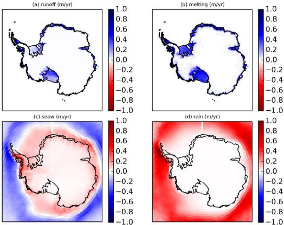
Figure 12: The difference between average 2090–2100 and average 2020–2030 of SMB components in SSP5–8.5: (a) surface runoff (b) surface melting (c) snowfall and (d) rainfall, all in m/yr. Black lines indicate the grounding lines of the ice sheet.
