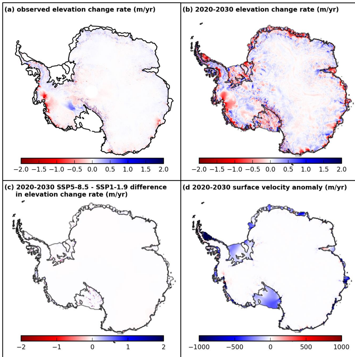
Figure 3:5: (a) IMBIE 1992-2017 mean observed elevation change rate (m/yr). Ice shelves and some grounded regions in the Antarctic Peninsula are not covered by the data. (b) 2020-2030 mean modelled elevation change rate (m/yr). (c) 2020-2030 difference of mean elevation change rate (m/yr) between the SSP5-8.5 and SSP1-1.9 scenario. (d) 2020-2030 mean surface velocity anomaly (m/yr) and (d) 2020-2030 mean ice thickness anomaly (m) with respect to the reference ice state (MartinCornford et al., 20192016). The black and grey lines in (b), (c) and (d) are the ice sheet grounding lines and ice shelf fronts respectively.
