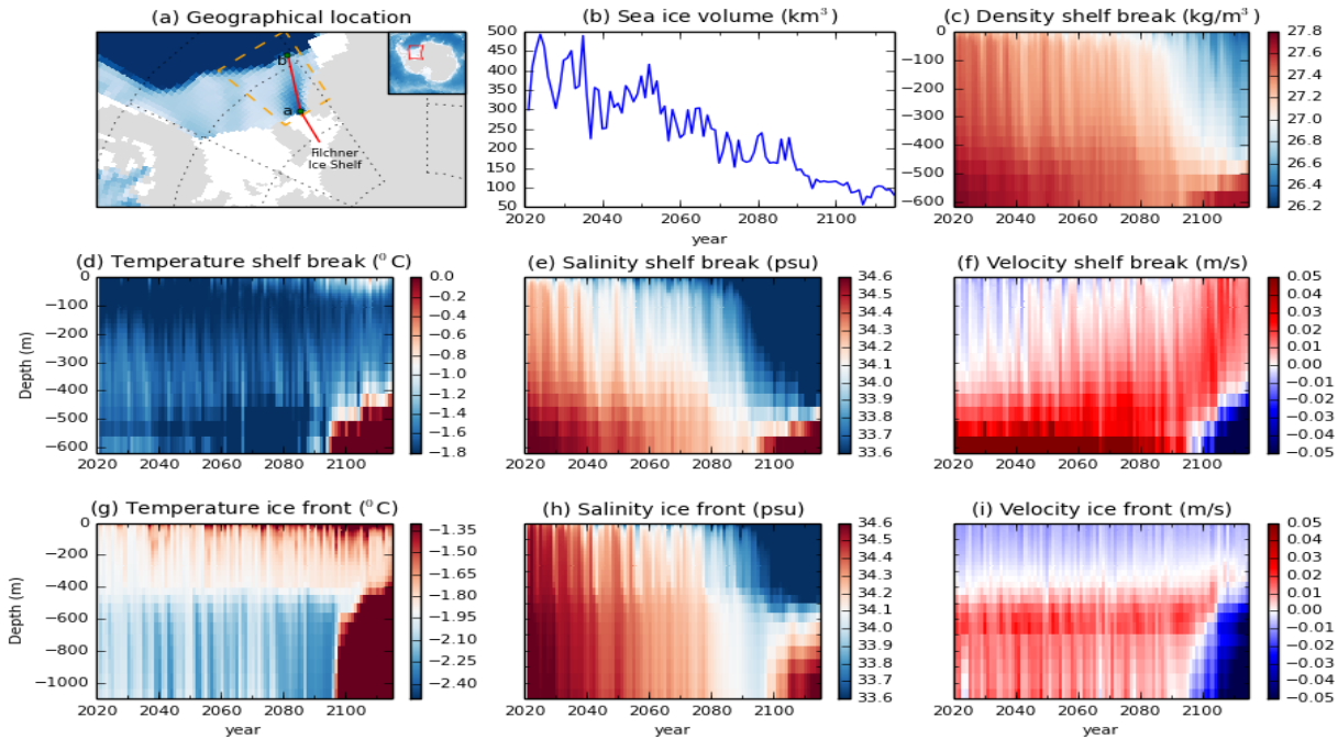
560 Figure 8: Filchner Trough profiles in the SSP5-8.5 scenario. (a) The chosen section on the Filchner Trough is indicated by the red line segment between the green dots a and b. The entire red line denotes the meridional section used in Figure 9. The dark and light blue colours represent the deep ocean and the continental shelf in the Weddell Sea, respectively, whereas the grey and white colours represent the grounded ice sheet and the Filchner-Ronne Ice Shelf, respectively. (b) sea ice volume on the area enclosed by the orange dashed lines in (a). (c-f) The timeseries of potential density, temperature, salinity and meridional velocity, respectively at the shelf break indicated by the green dot b in (a). (g-i) The timeseries of temperature, salinity and meridional velocity at the ice front indicated by the green dot a in (a). 565
