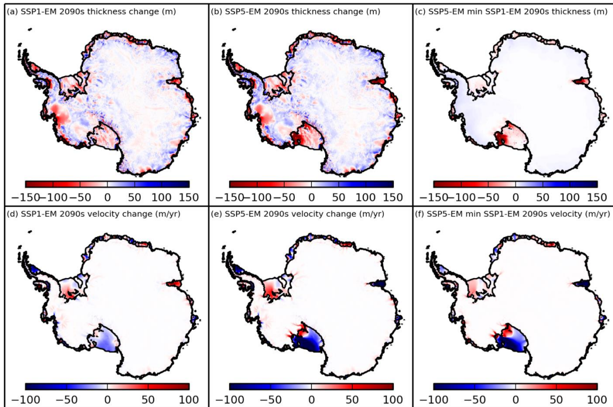
Figure 1315: Change of (top) ice thickness and (bottom) surface velocity magnitude between (Left) 2015 and 2100 in SSP1-1.9 (Middle) 2015 and 2100 in SSP5-8.5. (Right) Difference of (top) ice thickness and (bottom) surface velocity magnitude in the final period between SSP5-8.5 and SSP1-1.9 in the final period.
