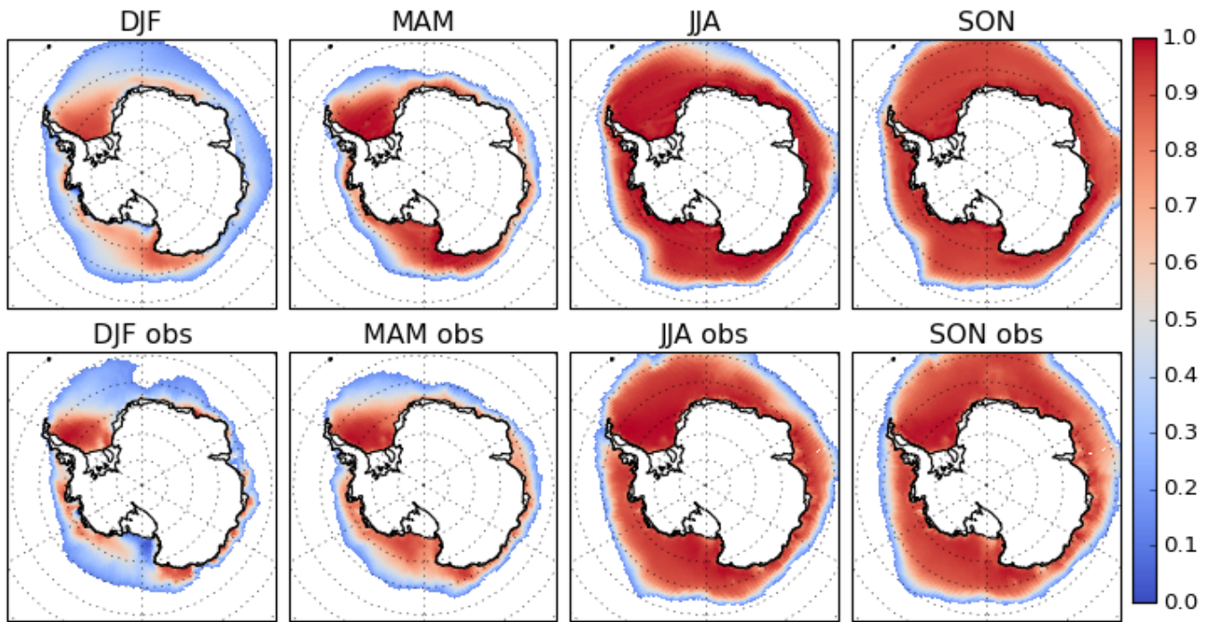
Figure 4: 2020-2030 ALL-EM (top) and HadISST1 (bottom) fractional sea-ice concentration in each season. The extent is defined by a threshold 0.15 concentration.
