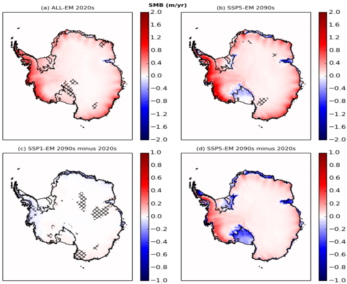
745 Figure 13: (a) ALL-EM SMB for period 2020-2030. Locations with statistically significant difference (95% Student's t -confidence interval) between SSP1-EM and SSP5-EM are hatched. (b) SSP5-EM SMB 2090-2100. Locations with statistically significant difference (95% confidence interval with one-way ANOVA) among the ensemble members are hatched. (c) Difference of SSP1-EM SMB between 2090-2100 period and 2020-2030 period. Locations where the difference is statistically significant (95% Student's t -confidence interval) are hatched. (d) Difference of SSP1-EM SMB between 2090-2100 period and 2020-2030 period, almost everywhere is statistically significant. Black and grey lines indicate the ice sheet grounding lines and ice shelf fronts, respectively.
