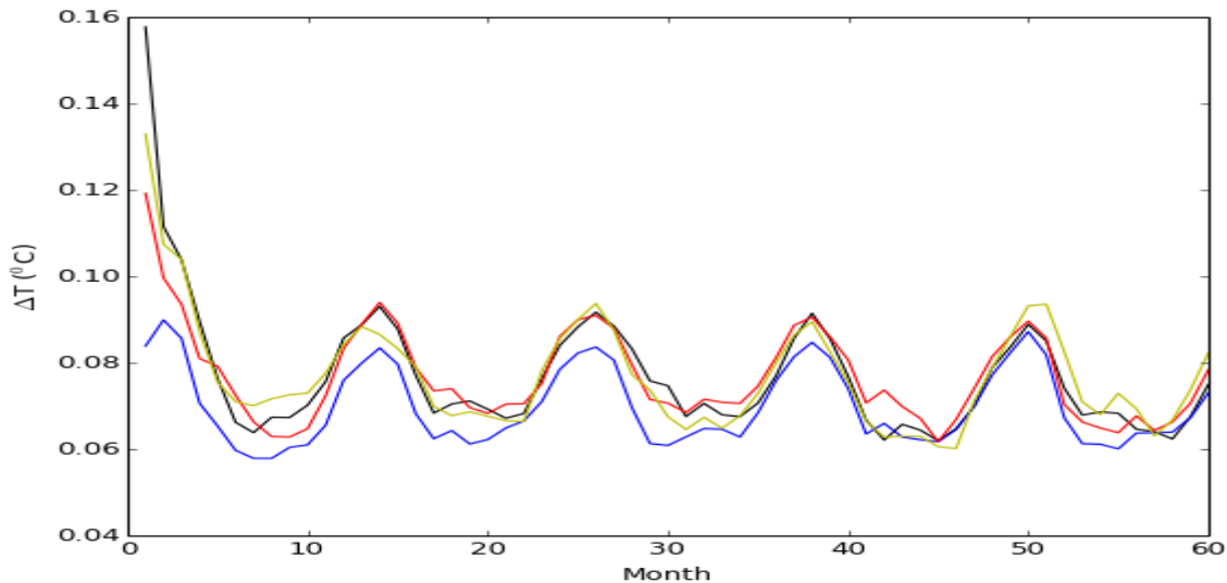
Figure 2: Monthly time-series of temperature difference across ice fronts averaged over depth and along the entire Antarctic coast in the first 5 years of ocean stand-alone integration (Stage C) for all (four) members. The blue line is the member that was not initialised with the global ocean from the UKESM1.0 CMIP6 historical ensemble.
