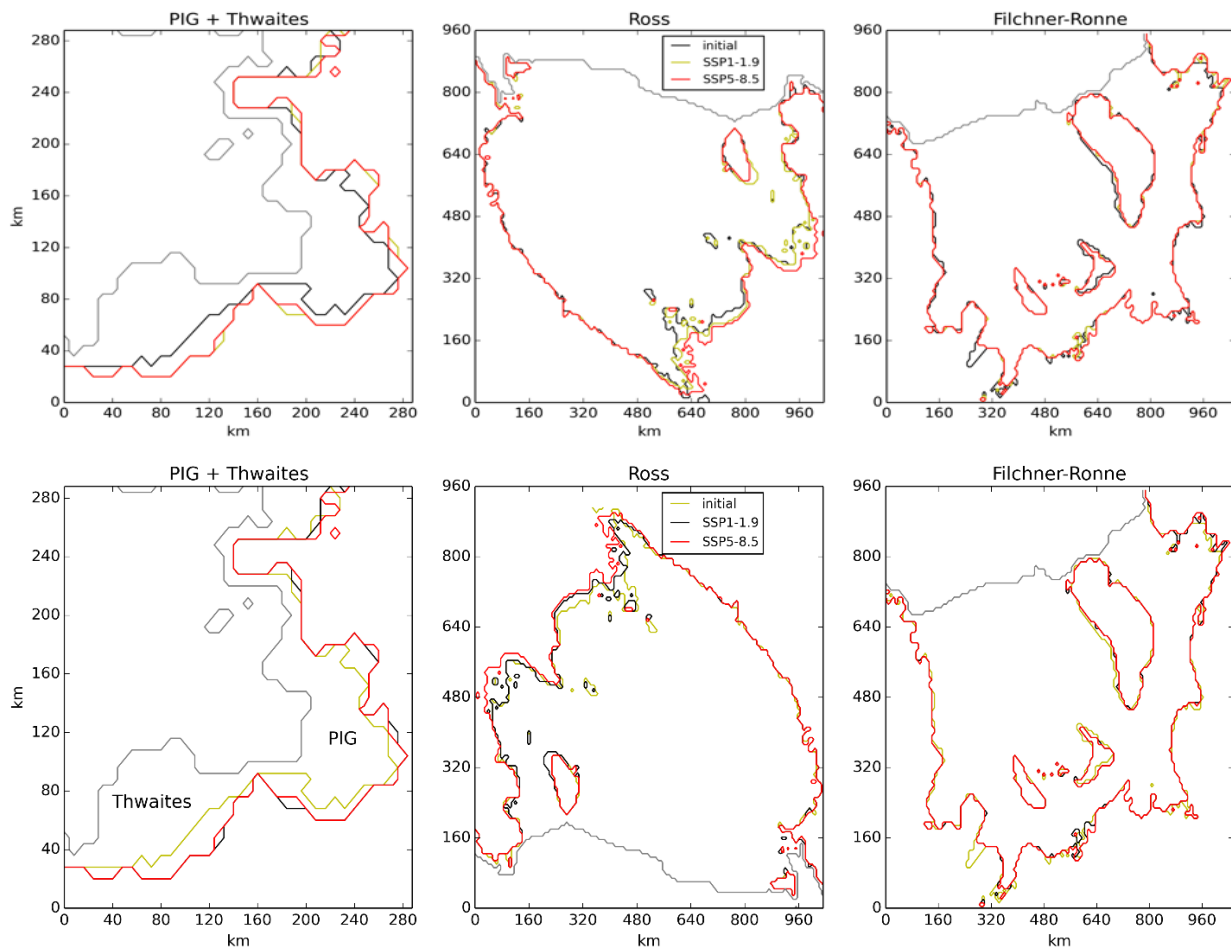
890 Figure 4517: Grounding line change in (Left) Pine Island & Thwaites Glaciers (Middle) Ross and (Right) Filchner-Ronne ice shelves. Gray=ice front, blackyellow =initial grounding line, yellowblack =grounding line for SSP1-1.9 in 2100, red=grounding line for SSP5-8.5 in 2100.
