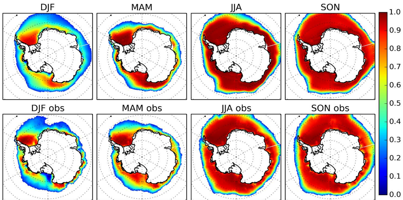
Figure 2: 2020-2030 ALL-EM (top) and HadISST1 (bottom) fractional sea ice concentration in each season. The extent is defined by a threshold 0.15 concentration.
