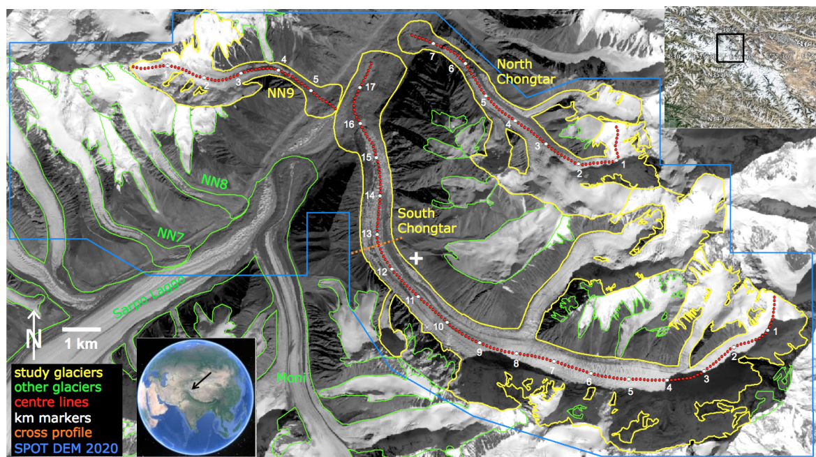
Fig. 1: Overview of the study region showing the location of the Karakoram Mountains (inset, lower left) and of the study region (inset upper right), outlines of the investigated glaciers (yellow), other glaciers (green), centre lines (red), km markers (white) cross-profile line (orange) and extent of the SPOT 2020 DEM perimeter (blue). The white + near the centre marks the coordinates 35.9^{\circ}\text{N} and 76.34^{\circ}\text{E} . The satellite image in the background is the Landsat 8 panchromatic band acquired on 21 Oct 2020. Credits: Landsat: earthexplorer.usgs.gov , the two insets are screenshots from Google Earth, © Google Earth).
