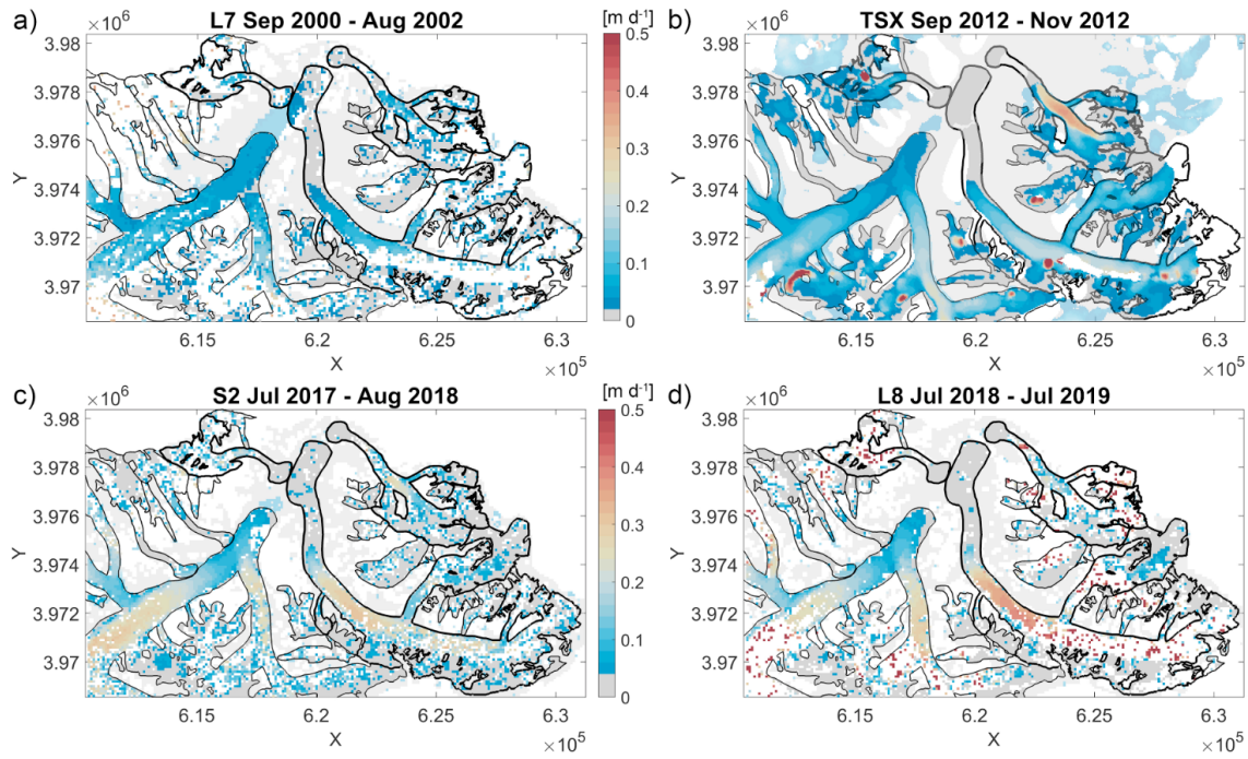
Fig. 5: Temporal evolution of 2D surface flow velocities for the three glaciers before 2020 derived from a) Landsat 7, b) TerraSAR-X, c) Sentinel-2, and d) Landsat 8. The dates of the compared images are given at the top of each panel. Grey values refer to velocities smaller than the uncertainty (see Table S2), i.e. <0.01 \text{ m d}^{-1} for panels a) and b) and <0.02 \text{ m d}^{-1} for c) and d).
