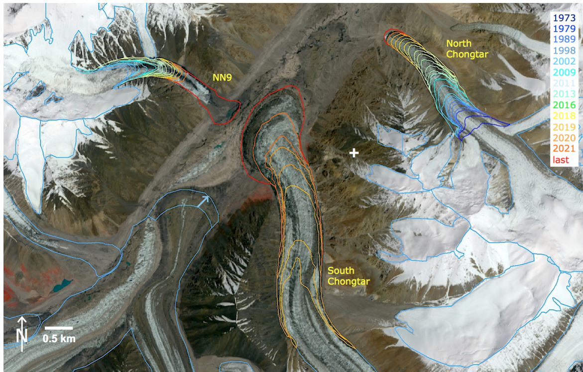
Fig. 3: Temporal evolution (colour-coded dates) of glacier extent for the three glaciers (NN9, North Chongtar, South Chongtar) investigated here. For comparison, the displacement of the terminal lobe of Moni Glacier from 2000 to 2020 is also shown (blue arrow). ‘Last’ is referring to 30 September 2021, the + sign near the centre marks the coordinates 35.93°N and 76.34°E. Background: Sentinel-2 image acquired on 16 July 2021 with bands 8/4/3 as RGB (Copernicus Sentinel data 2021).
