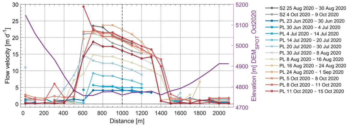
Fig. 9: South-west to north-east cross-profile surface flow velocities for South Chongtar Glacier derived from Planet and comparison with Sentinel-2. The vertical dash line indicates the location of the centerline. See Fig. 1 for location of the cross profile.
