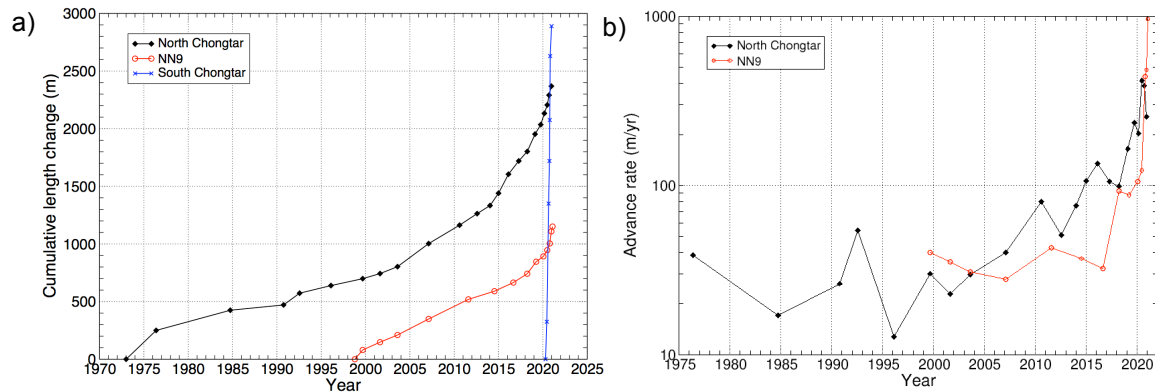
Fig. 4: Terminus changes for the investigated glaciers. a) Cumulative length changes (the retreat phase of South Chongtar before 2020 is not shown), b) advance rates.
