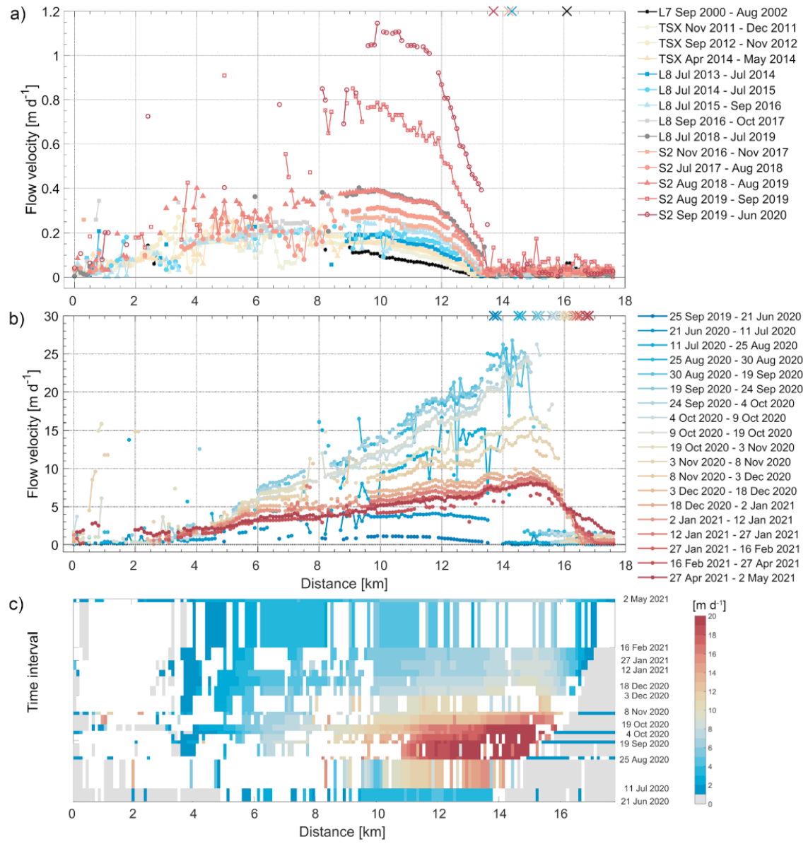
Fig. 7: Temporal evolution of flow velocities for South Chongtar Glacier from its highest point to its terminus, its location is indicated by an 'x' at the top of panels a) and b). a) Pre-surge values along the centre-line as derived from different satellites (names see Fig. 6). b) As a) but during the surge and derived from Sentinel-2 only, c) Hovmöller diagram of the surge phase. In this plot grey values are below 1 \text{ m d}^{-1} , white indicates no data.
