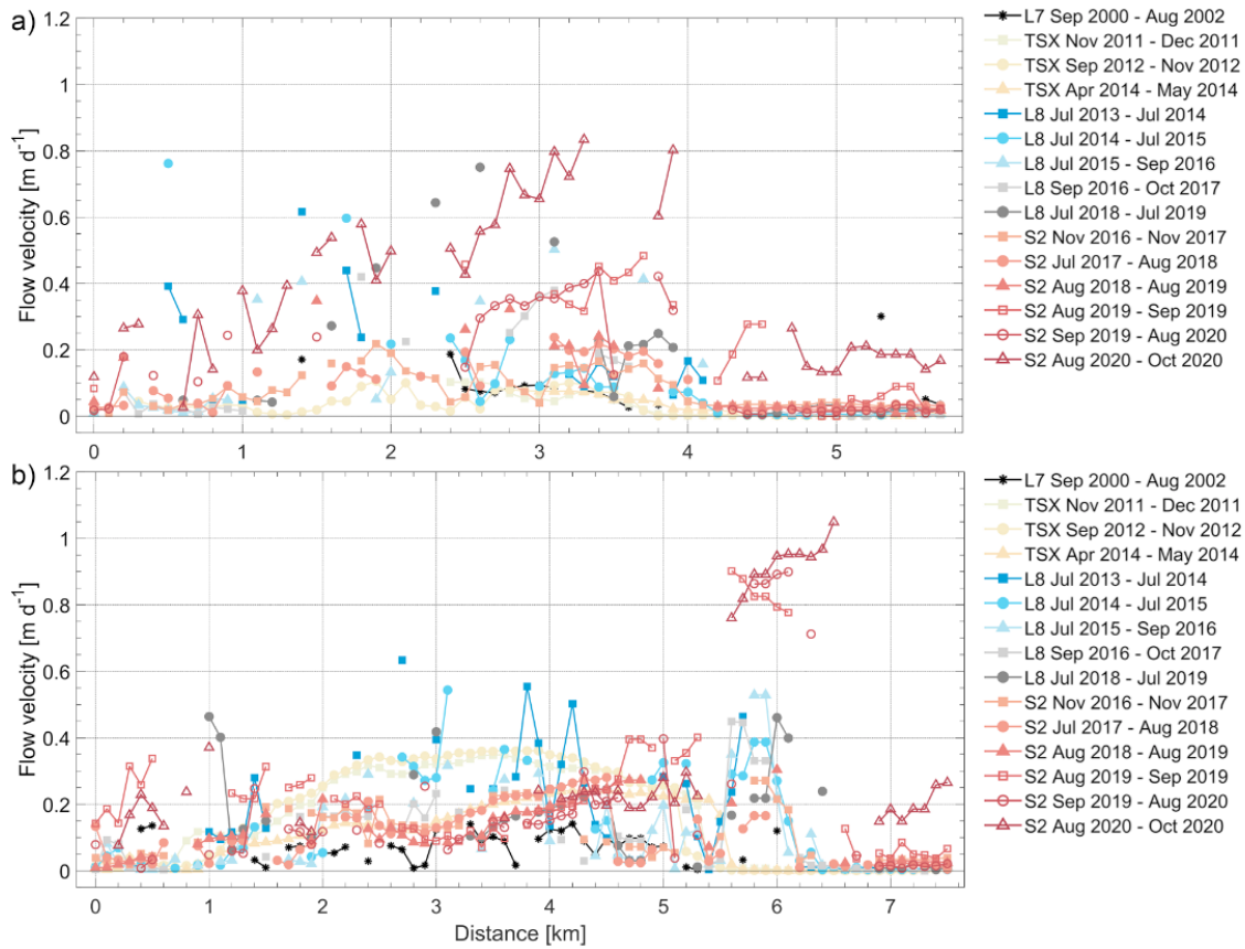
Fig. 6: Temporal evolution of 1D flow velocities along a centre-line starting at the highest point of each glacier for a) glacier NN9 and b) North Chongtar. Satellite names: L7/L8: Landsat 7/8, TSX: Terra-SAR-X, S2: Sentinel-2.
