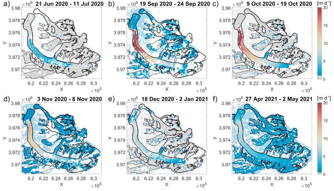
Fig. 8: Temporal evolution of 2D flow velocities for South Chongtar Glacier during its surge as derived from Sentinel-2. The dates of the respective Sentinel-2 pairs are given at the top of each panel. Grey values refer to velocities smaller than one standard deviation (see Table S2), i.e. <1 \text{ m d}^{-1} for panels a) to c) and <0.5 \text{ m d}^{-1} for d) to f).
