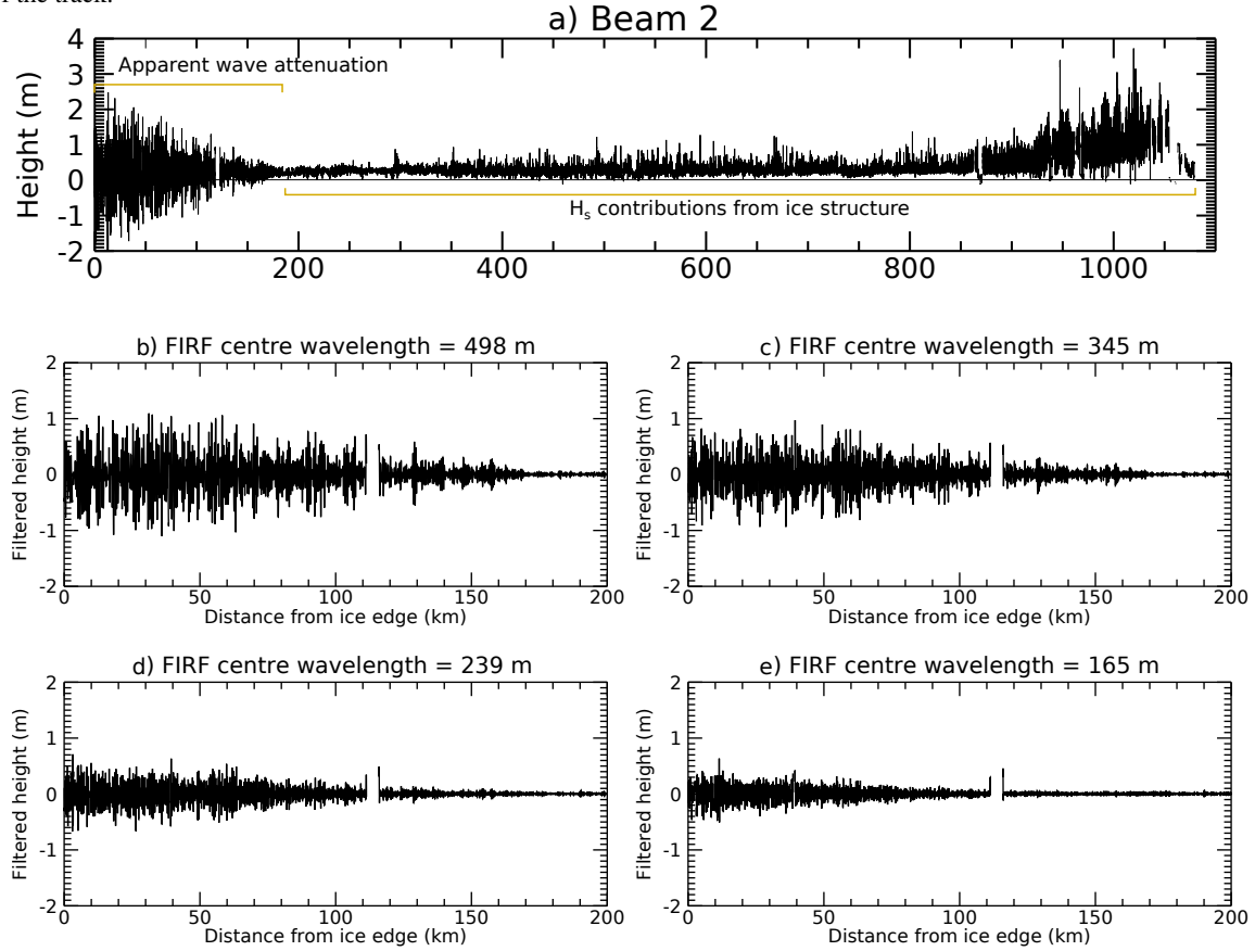
Figure 2. Panel a: Resampled segment heights from the central strong beam, for case study 1. Data acquisition start time 2019-09-09T19:15:19Z. Panels b-e: SDF-filtered heights for each of the four FIRF filters used in wave penetration width estimation, for the first 200 km of the track.
