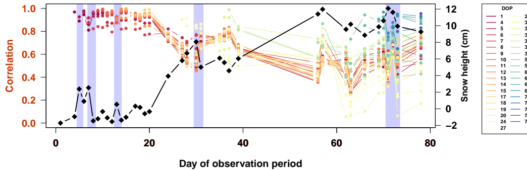
Figure 7. Correlation between the DEM-derived surface structures of a particular day and the surface structure on every following day (coloured points) as well as the overall snow height evolution (black diamonds). The colour-code indicates the DOP of the surface structure to which all subsequent structures are correlated to. The entire DEM area is considered for the correlation calculation. Vertical blue bars indicate an increase in the correlation and a decrease in the snow height. The second blue bar to the left shows the decrease in snow height from DOP 7 to DOP 8 which is illustrated in Fig. 6.
