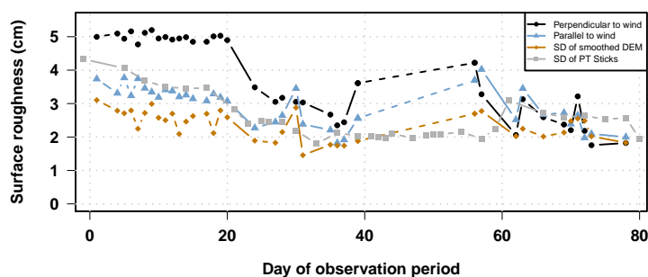
Figure 10. Temporal evolution of the surface roughness estimates throughout the observation period as described in section 2.4. The estimates parallel (blue) and perpendicular (black) to the main wind direction show an overall similar behaviour with the latter estimate suggesting higher roughness estimates at the beginning of the observation period. In addition, larger-scale undulations (gold) follow the overall pattern as well with an overall lower roughness estimate. The standard deviation across all PT stick measurements (grey) is used to fill the DEM data gap between DOP 40 and DOP 56 and follows the other estimates.
