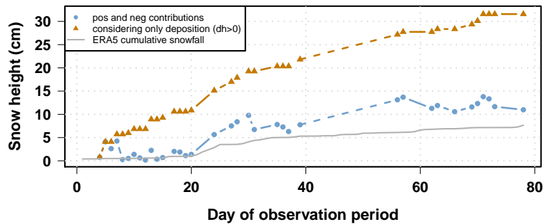
Figure 12. Cumulative snow height over the observation period from DEM-derived data and from the ERA5 reanalysis snowfall product. The DEM-derived snow height is shown for the two possibilities of i) counting both positive and negative contributions from one day to the next (blue), and ii) counting only the positive contributions (gold). The ERA5 snowfall (grey) is converted from mm w.e.q. to cm assuming a mean snow density of 290 \text{ kg m}^{-3} which was obtained from daily density measurements of the top 2.5 cm at the stick positions of the SSA transect. Considering only the positive changes in the DEM-derived data accounts for deposition by snowfall or drift, but not for snow removal (e.g., erosion). This indicates that more than half of the snow that arrived at the study site was eroded and redistributed, and was thus transported out of our study area.
