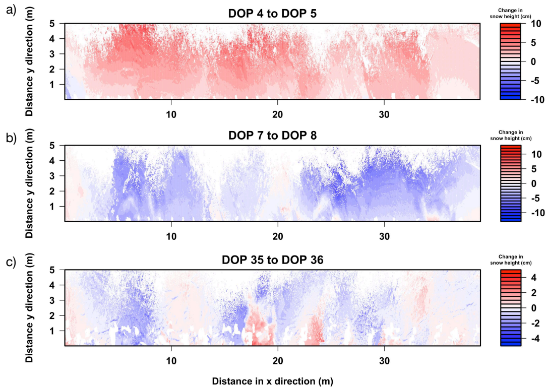
Figure 5. Day-to-day variations shown as the change in snow height (in cm) of the entire DEM-area for three periods: a) DOP 4 to DOP 5 shows an increase in the snow height for 78 % of all pixel, b) the change from DOP 7 to DOP 8 is dominated by snow erosion for 65 % of all pixel, and c) the snow height evolution from DOP 35 to DOP 36 is characterised by a spatially patchy pattern with positive and negative changes. For each panel, the zero-line indicates areas without changes in the snow height.
