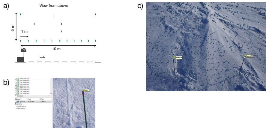
Figure B2. Validation area and possible error sources during the processing workflow. a) Schematic illustration of the validation area which was set up according to the same procedure as the main study area. 13 glass fibre sticks were distributed around the validation area (green): eleven sticks were aligned at the downwind side in a straight line with 1 m-spacing and two sticks at the upwind corners at 5 m distance from the main line. Four additional sticks ( validation sticks , black) were distributed inside the area. b) Allocation of GCPs (ground control points) during the process of DEM (digital elevation model) generation. The top of the glass fibre sticks were used as GCPs and manually checked for correct alignment (c).
