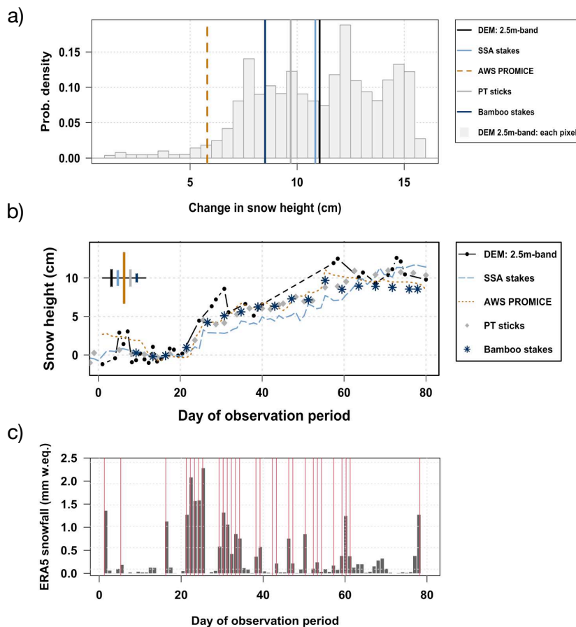
Figure 4. Evolution and changes of different snow height estimates throughout the observation period. a) Histogram of the DEM-derived change in snow height (grey bars) for every single pixel of the 2.5 m-band from DOP 1 to DOP 78 (Fig. 3 fourth panel) together with the mean snow height change (black vertical line) in the 2.5 m-band, as well as the mean snow height changes from other methods (vertical lines; Tables 1 and 2). Note that the latter estimates cover different spatial extents. b) Mean temporal evolution of snow height estimates throughout the observation period from the DEMs (2.5 m-band; black), the SSA stakes (light blue), the AWS PROMICE (gold), the PT Sticks (grey), and the Bamboo stakes (dark blue). For a direct comparison, each estimate is referred to its mean value from DOP 10 to DOP 20, which is defined as the zero level. Vertical bars include the uncertainty in cm ( \pm one standard error) due to the limited spatial resolution of each method assuming a spatial decorrelation length of 5 m for our study site. The AWS PROMICE has the largest uncertainty because it is a single point measurement. c) The ERA5 snowfall product (grey bars) and manually documented snowfall during the observation period (red lines, see Appendix Table A1).
