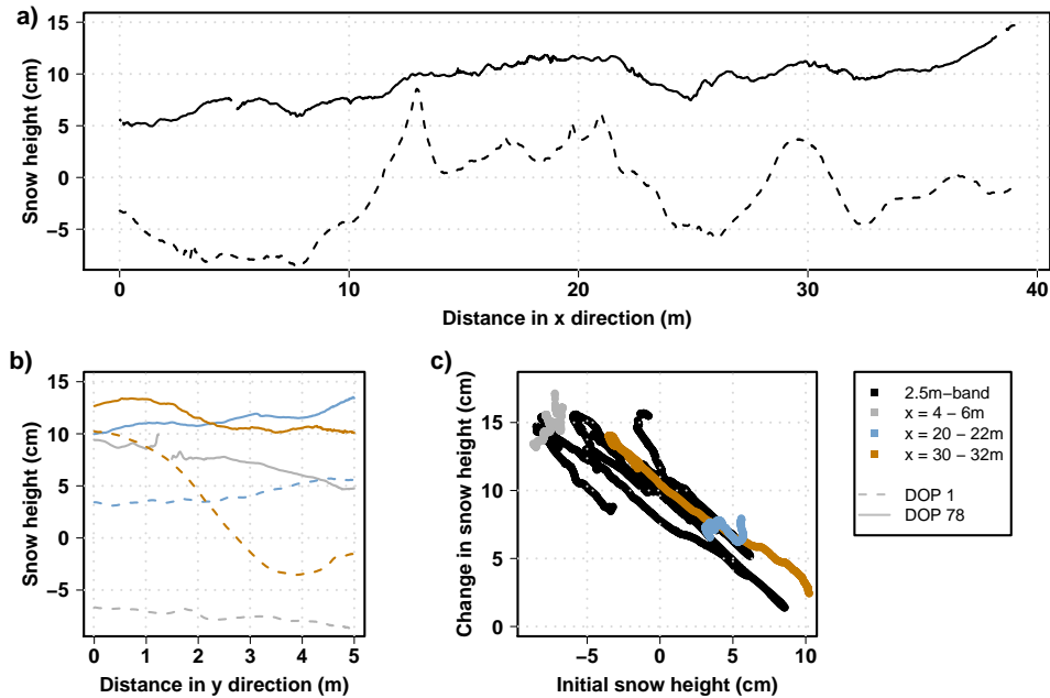
Figure 9. DEM-derived relative snow heights for 16 th of May (DOP 1, dotted lines) and 1 st of August, 2018 (DOP 78, solid lines) for four subareas of the study area: a) the 2.5 m-band perpendicular to the main wind direction; b) three subareas parallel to the main wind direction (grey: x = 4-6 m, blue: x = 20-22 m, and gold: x = 30-32 m) marked with grey bars in Fig. 3. c) Relationship between the initial snow height on DOP 1 and the change in snow height to DOP 78 for the subareas in a) and b). Note that the legend refers to all panels. The relation for each individual pixel in the study area is shown in the Appendix Fig. C3.
