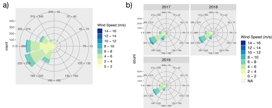
Figure A2. Wind characteristics (speed and direction) for the EGRIP camp site recorded by the PROMICE AWS for a) the observation period (16 th of May to 1 st of August 2018), and b) the years 2017, 2018 and 2019, respectively.
