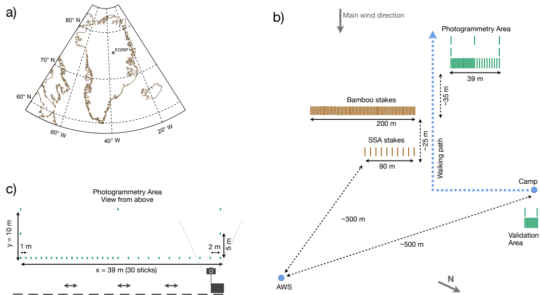
Figure 1. Overview maps for all relevant locations and transects in our study. a) Map of Greenland with the location of the EGRIP camp site in northeast Greenland. b) Schematic map of the EGRIP area including all relevant study sites. This area is approximately 200 m south of the deep drilling site at the EGRIP camp and about 300 m from the AWS. The map is not to scale. Data from the AWS, the Bamboo stakes, and the SSA transect (SSA = Specific Surface Area) are used for the comparison of snow height estimates. Data from the Validation Area are described in the Appendix B. c) Schematic illustration of the Photogrammetry area with respective distances. 30 glass fiber sticks were set along the walking line (x-axis), four sticks were positioned on the edges towards the main wind direction (y-axis), and one in the back of the study area. The sledge with the camera is located as is shown in Fig. 2. The approximate field of view of the camera is illustrated with grey lines.
