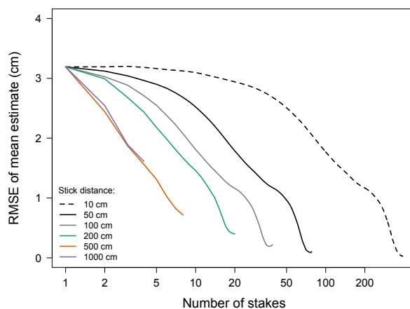
Figure 14. The uncertainty of the estimated mean snow height change as a function of the number of sampling points ("stakes") and the distance between them. The mean snow height change is calculated from the DEM data at y=2.5 m for all possible sequences along the x-direction which consist of N sampling points with a given distance from one point to the next. The figure shows the RMSE between the DEM-derived mean snow height change of the respective sequences and the mean snow height change as calculated using all available sampling points.
