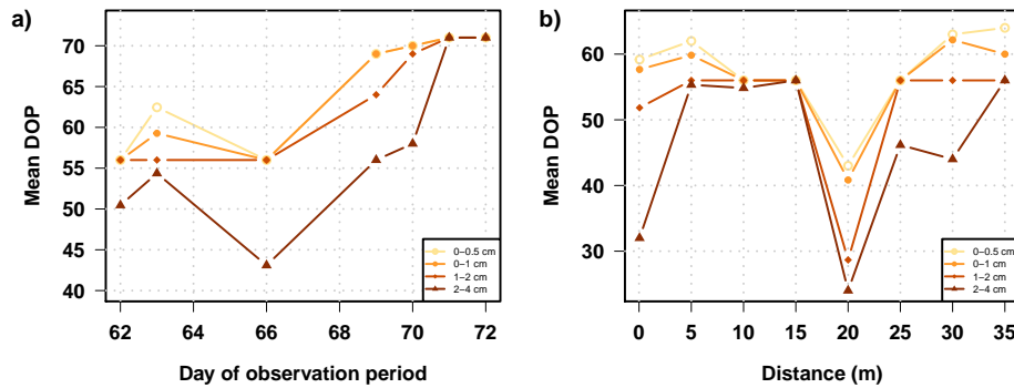
Figure 13. Theoretical temporal and spatial sampling of different depth intervals (0-0.5 cm, 0-1 cm, 1-2 cm and 2-4 cm) of the internal snow structure along the 2.5 m-band. a) Temporal sampling for ten consecutive days at x = 12 m. b) Spatial sampling at eight positions with 5 m spacing along the 2.5 m-band on DOP 69. The y-axes in a) and b) represent the average day of snow accumulation for the respective depth interval.
