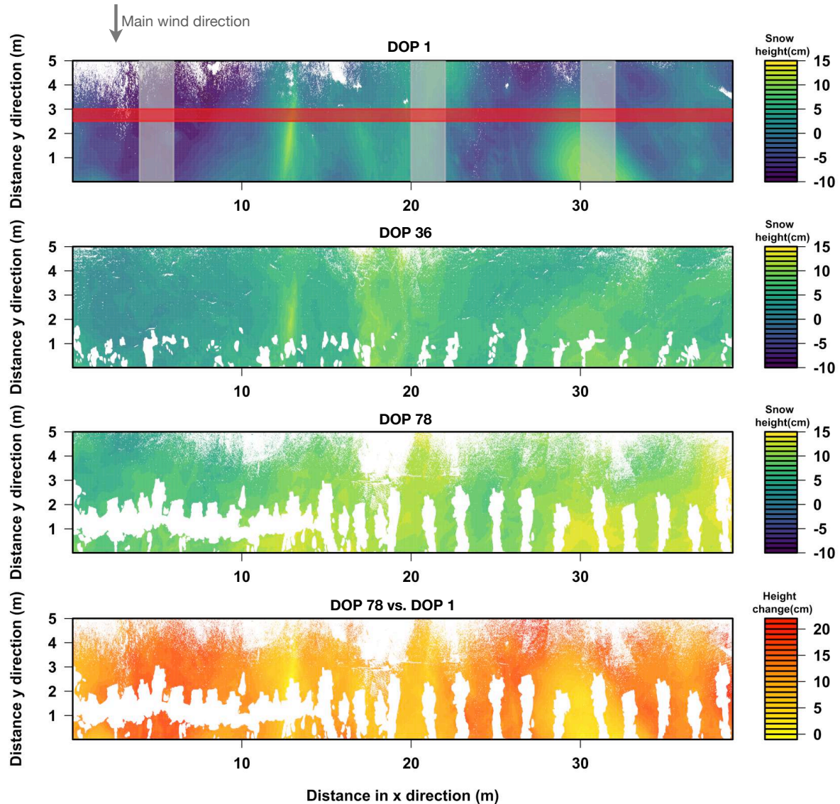
Figure 3. DEM-derived relative snow heights presented as two-dimensional maps (39 x 5 m). Shown are the snow heights for the Day of Observation Period 1 (16 th of May 2018, DOP 1, upper panel), DOP 36 (20 th of June 2018, second panel), and DOP 78 (1 st of August 2018, third panel) as well as the change in snow height between DOP 1 and DOP 78 (fourth panel). Snow height estimates are given in cm relative to the snow height at x=0 m and y=0 m on the day of installation. The y-direction points towards the main wind direction. The red bar (in the top panel) indicates the band along the x-direction from y=2.5 to y=3 m (50 cm width), which is used to obtain average snow heights for each day for further analyses. The grey bars mark three subareas for the analyses in section 3.4 and Fig. 9. Missing data are shown as white areas and are caused either by a snow sampling performed in the same area (white spots close to the lower main line) or by insufficient image quality.
