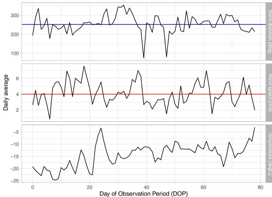
Figure A1. Daily averages of meteorological parameters, i.e., wind direction in [ ^{\circ} ], wind speed in [ \text{m s}^{-1} ] and air temperature in [ ^{\circ}\text{C} ], measured at 2 m height at the AWS PROMICE for the observation period from 16 th of May (DOP 1) to 1 st of August 2018 (DOP 78). In the first panel, the horizontal blue line indicates the average wind direction of 252^{\circ} during the observation period. The horizontal red line in the second panel marks the threshold wind speed of 4 \text{ m s}^{-1} . Snow transport is enabled when the threshold is exceeded for a 100 hour average (Groot Zwaafink et al., 2013).
