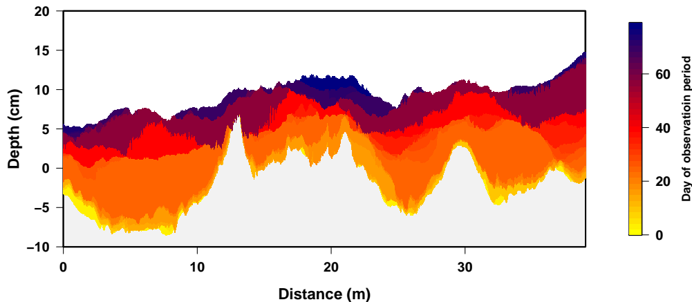
Figure 11. Two-dimensional view of the internal structure of our study area based on DEM-derived snow height variations along the 2.5 m-band for the last day of our observation period (DOP 78). Colours indicate the day of deposition during the season, namely when the DEM data recorded an increase in the snow height at the respective location. The grey background represents older snow and surface undulations prior to the first DEM on DOP 1. The long data gap between DOP 39 and DOP 56 does not cause an unrealistically thick snow layer which suggests that the temporal resolution of our data set does not affect the derived internal structure.
