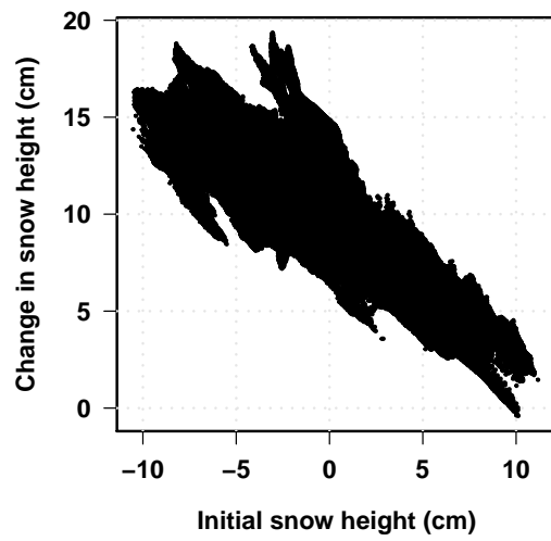
Figure C3. Relationship between the initial snow height on DOP 1 and the change in snow height on DOP 78 relative to DOP 1 for each pixel in the study area.
