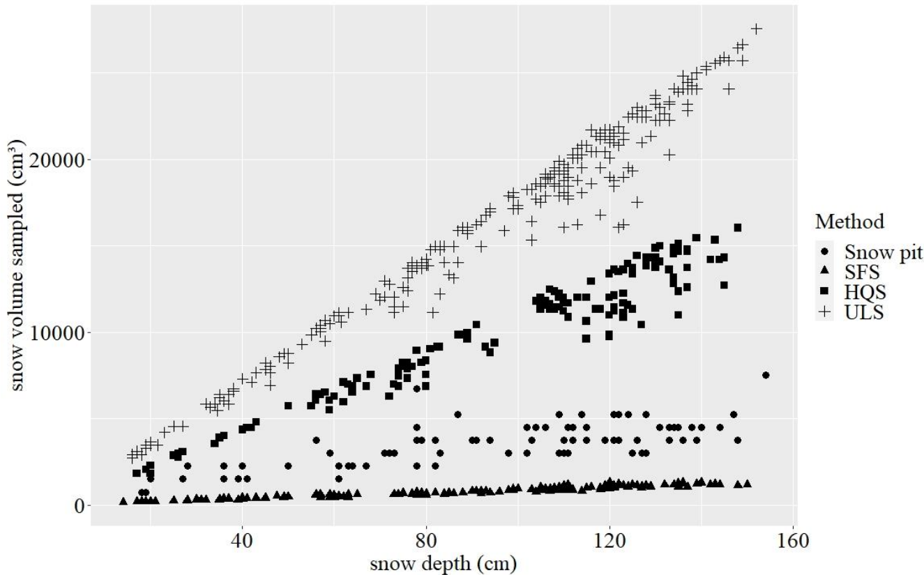
Figure 5: Volume of snow that was sampled using each SWE estimation method in relation to snow depth.
