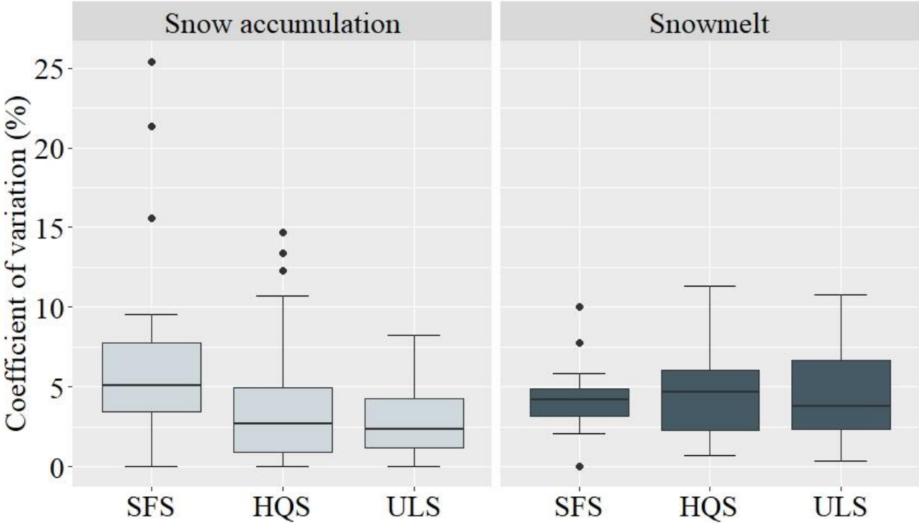
355 Figure 3: Coefficient of variation of SWE that was measured with three snow samplers according to the period of snow accumulation or melting: the Standard Federal sampler (SFS); the HQ Sampler (HQS); and the UL Sampler (ULS). Boxes represent 25th and 75th percentiles. Bars inform of the lowest and highest quartiles, excluding the outliers represented by the dots. The middle line in each box shows the median of the data.
