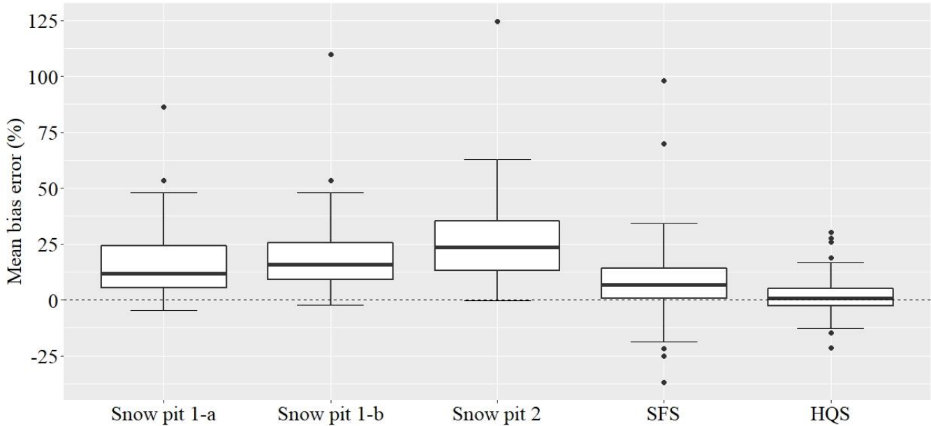
Figure 4: Mean bias error of the different SWE measurement methods relative to the UL sampler, which was used as SWE reference. The value above each boxplot is the average MBE for each method. Boxes represent 25th and 75th percentiles. Bars inform of the lowest and highest quartiles, excluding the outliers represented by the dots. The middle line in each box shows the median of the data.
