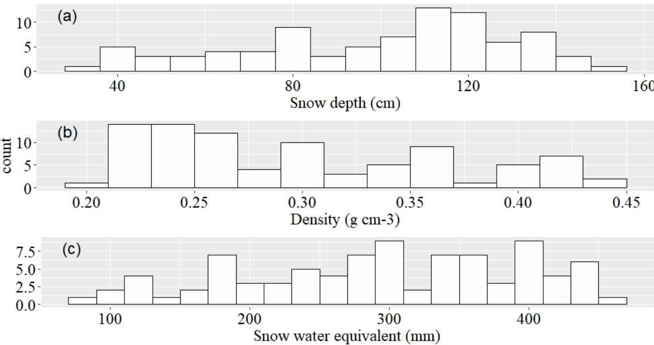
Figure 2: Distribution of (a) mean snow depth, (b) mean snow density and (c) mean snow water equivalent on the NEIGE site for 2016-2020 field measurements
