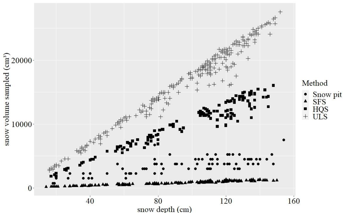
Figure 5: Volume of snow that was sampled using each SWE estimation method in relation to snow depth.
