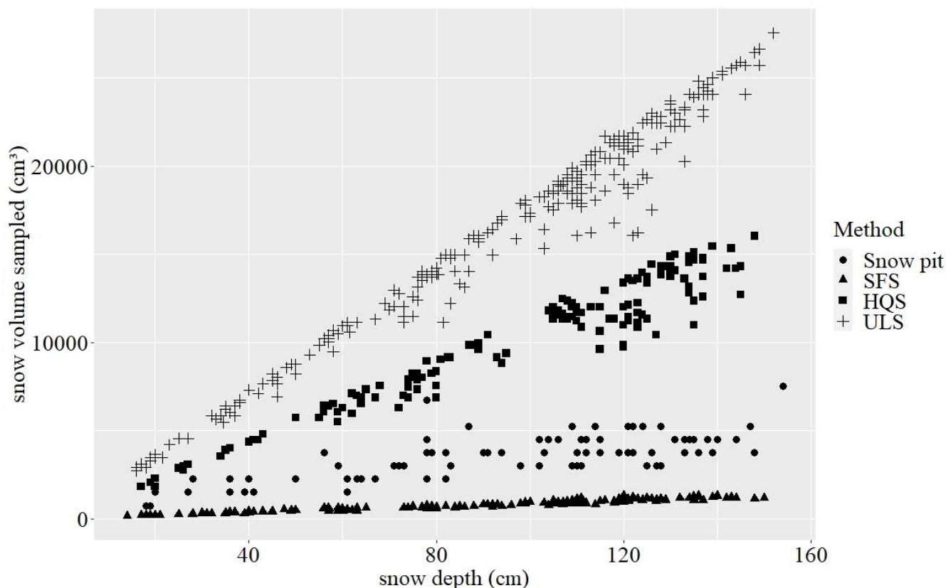
415 Figure 54: Volume of snow that was sampled using each SWE estimation method in relation to snow depth.
