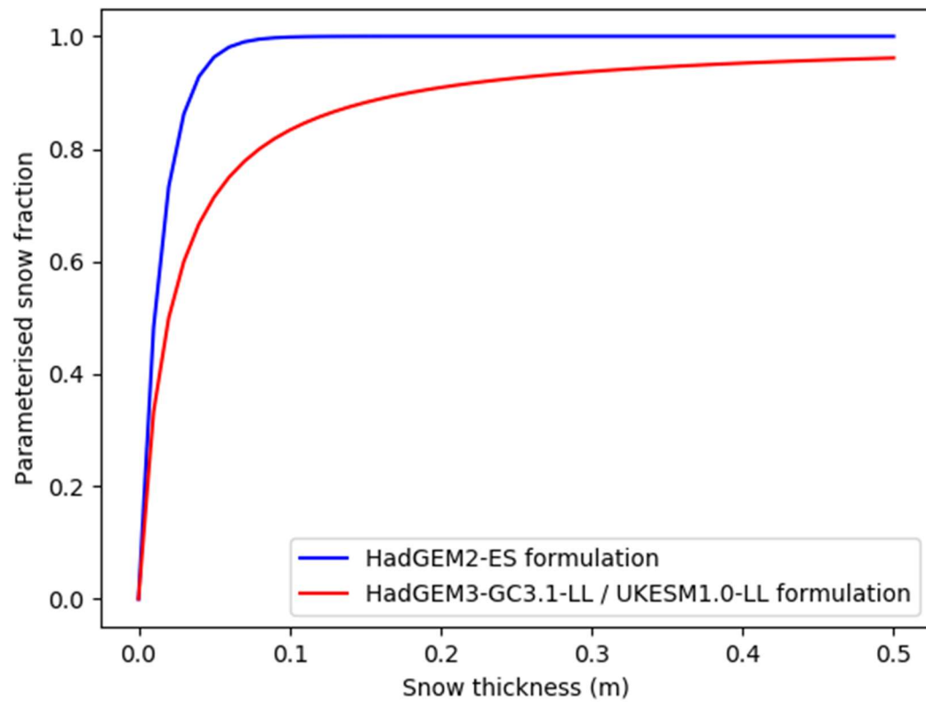
Figure S1. Snow area as a function of snow thickness in the HadGEM2-ES formulation (blue) and the HadGEM3-GC3.1-LL and UKESM1.0-LL formulations (red).
