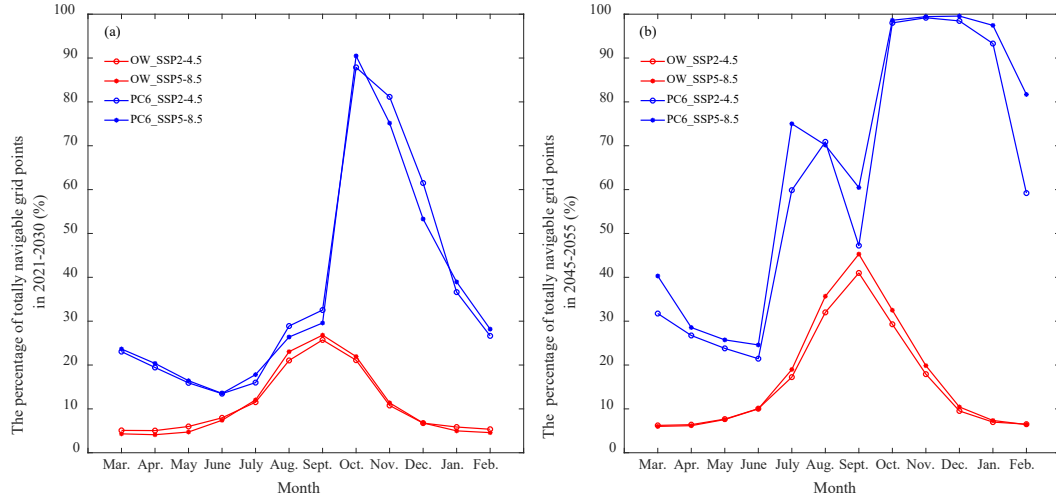
Figure. 7. The percentage of totally navigable grid cells for OW ships and PC6 ships under SSP2-4.5 and SSP5-8.5
