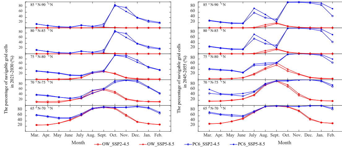
Figure. 8. The percentage of navigable grid cells for OW ships and PC6 ships under SSP2-4.5 and SSP5-8.5 within different latitudes
