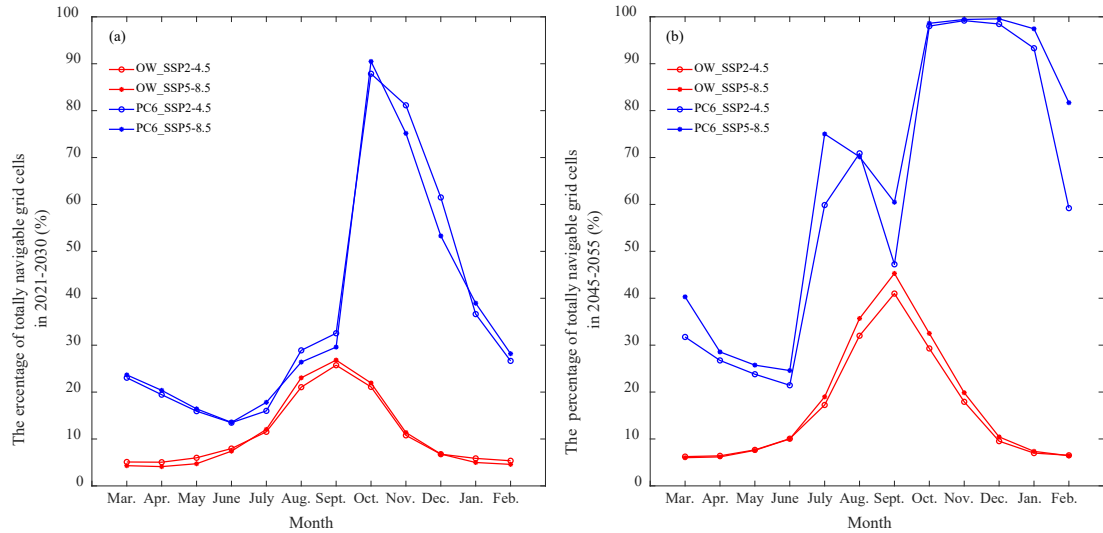
Figure 7. The percentage of totally navigable areas-grid cells for OW ships and PC6 ships under SSP2-4.5 and SSP5-8.5
