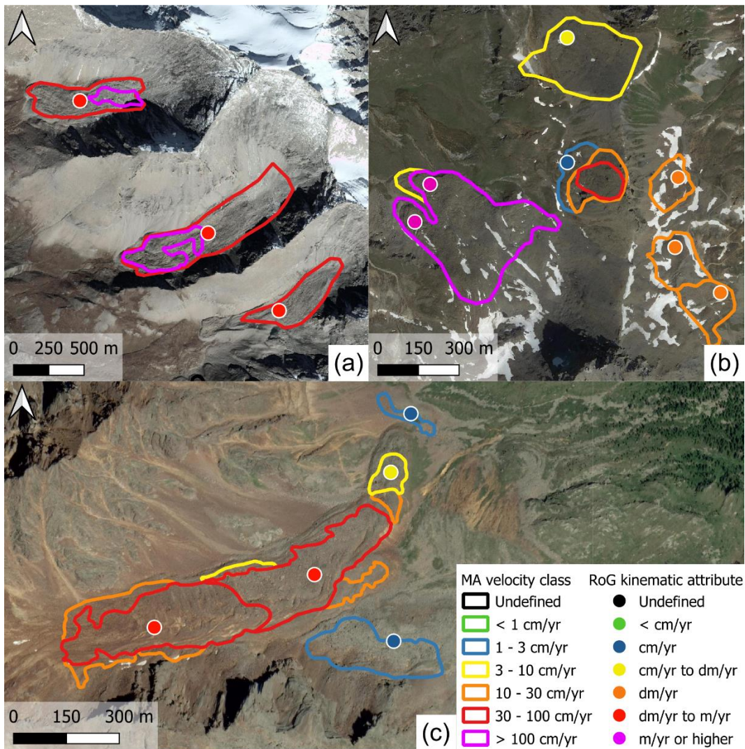
Figure 4. Examples of moving areas and rock glacier kinematic attributes produced for Vanoise (a, location: 45^{\circ}16'10''\text{N } 7^{\circ}03'00''\text{E} , 2900 m), Western Swiss Alps (b, location: 46^{\circ}10'25''\text{N } 7^{\circ}30'45''\text{E} , 2700 m), and Southern Venosta (c, location: 46^{\circ}28'20''\text{N } 10^{\circ}48'00''\text{E} , 2500 m). Orthoimages from © Google Earth 2019.
