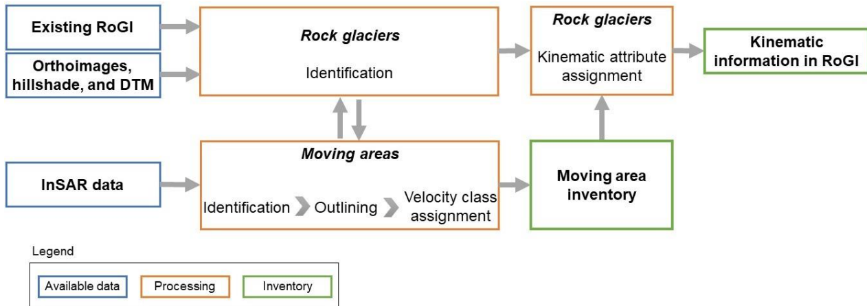
Figure 2. Conceptual diagram of the standardized method for producing a moving area inventory and a rock glacier inventory (RoGI) that includes kinematic information. The analysis is performed in a GIS environment.
