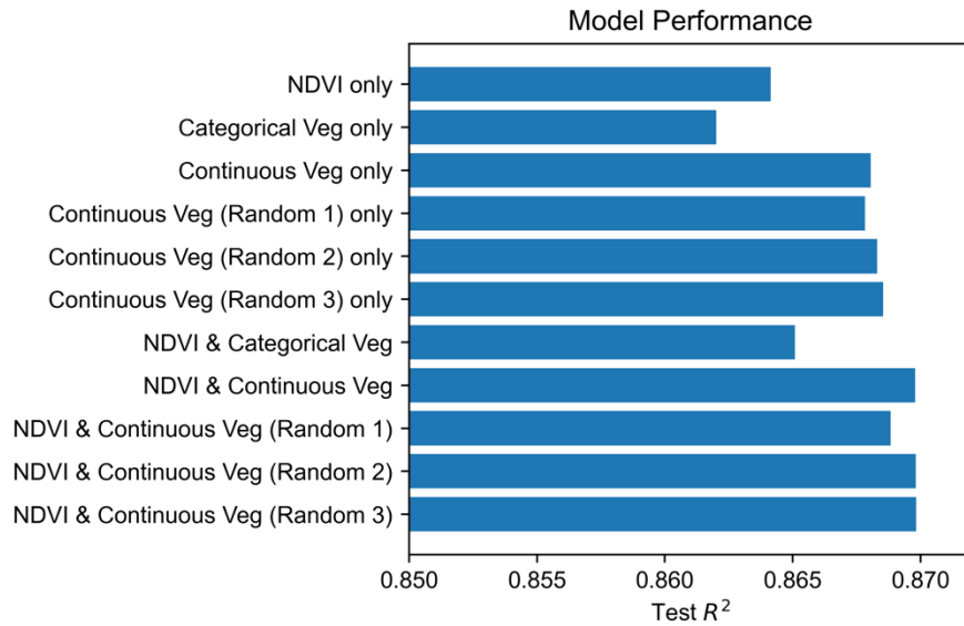
090 Figure A4. Random forest model performance for model runs using various combinations of vegetation features. The categorical vegetation uses the vegetation types shown in Figure 3. The continuous 095 vegetation is a ranking ordered by which vegetation type has higher SWE. The continuous vegetation 100 ranking is also randomized three different ways to determine if the ranking order is important. 105
