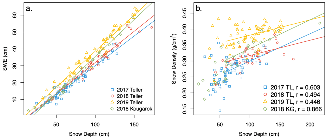
955 Figure 3. Scatter plots of (a.) snow depth vs SWE and (b.) snow depth vs snow density. The linear regressions in panel b. are for snow depth > 60 cm.
