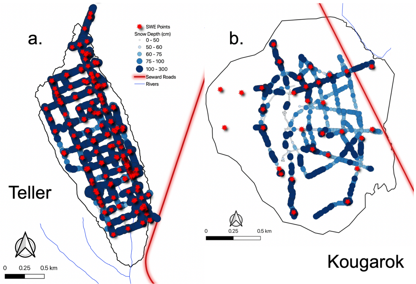
Figure 2. Measured snow depth (cm) and snow density (SWE Points) at a.) the Teller watershed (2017-2019) and b.) the Kougarok Hillslope (2018).
