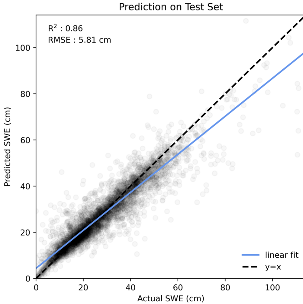
985 Figure 7. Random forest results of predicted SWE vs actual SWE for the test set when using all year and site datasets, with a test set of 20%. R^2 equal to 0.86 and the RMSE is equal to 5.81 cm. The solid blue line is a linear fit to the scatter points, and the dashed black line is a y=x line.
