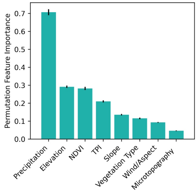
Figure 9. Random forest feature importance results (left, impurity and right, permutation) for the final model, with \pm 1 standard deviation shown by the black error bars.
