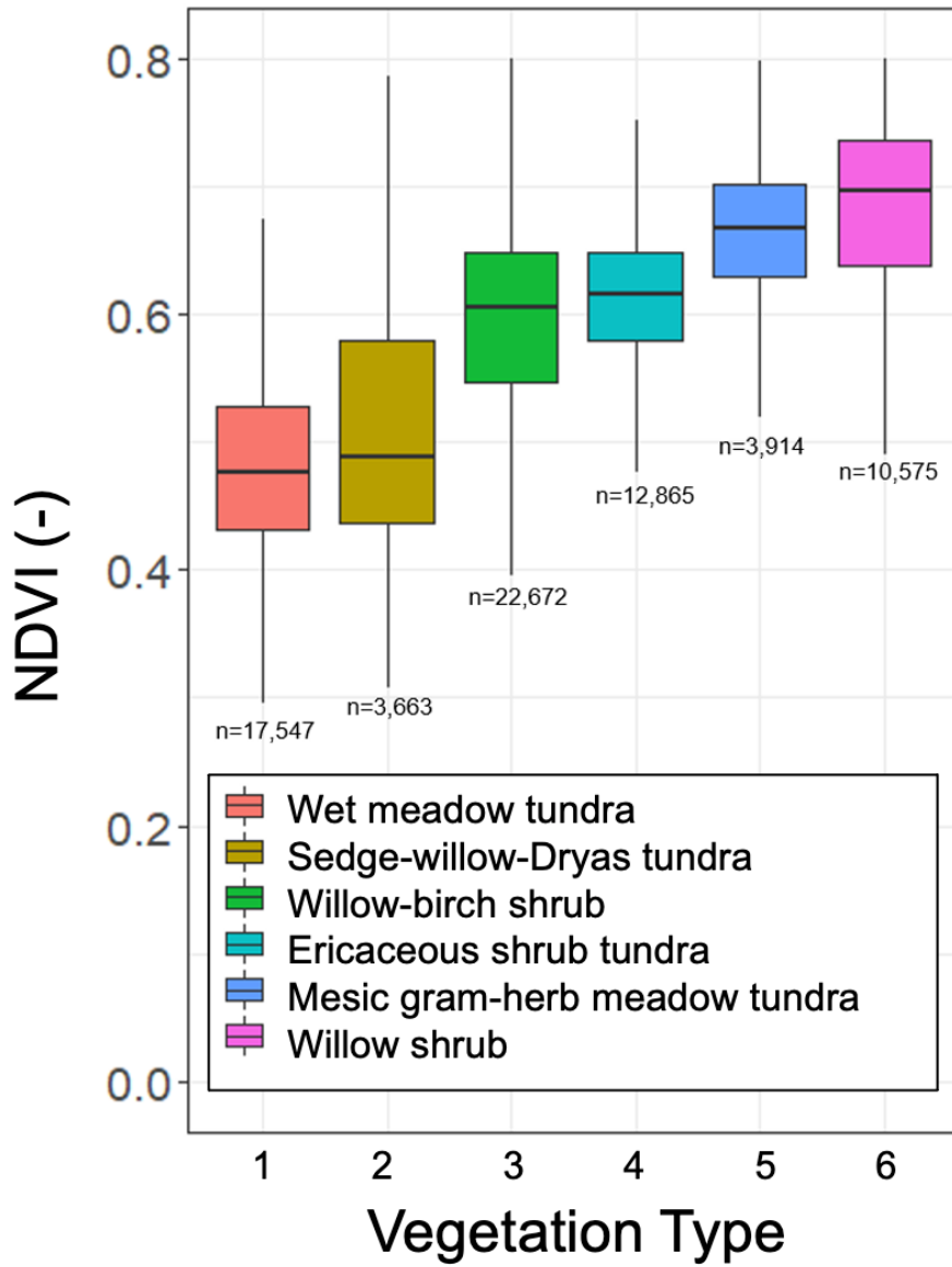
960 Figure 5. Teller watershed NDVI by major vegetation type. Mesic gram-herb is short for mesic graminoid-herbaceous tundra. Table A1 details each vegetation type.
