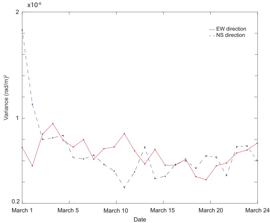
Figure 6. Daily evolution of the variance of measurement errors, estimated with the simulated annealing algorithm, as described in section 2.4.2. Variance in the EW (red) and NS (blue) directions. The variance in the EW direction remains stable, at around 0.5e-6 . That in the NS direction appears to show a slightly decreasing pattern, which appears to be the consequence of temporal variations of the ice properties in this direction.
