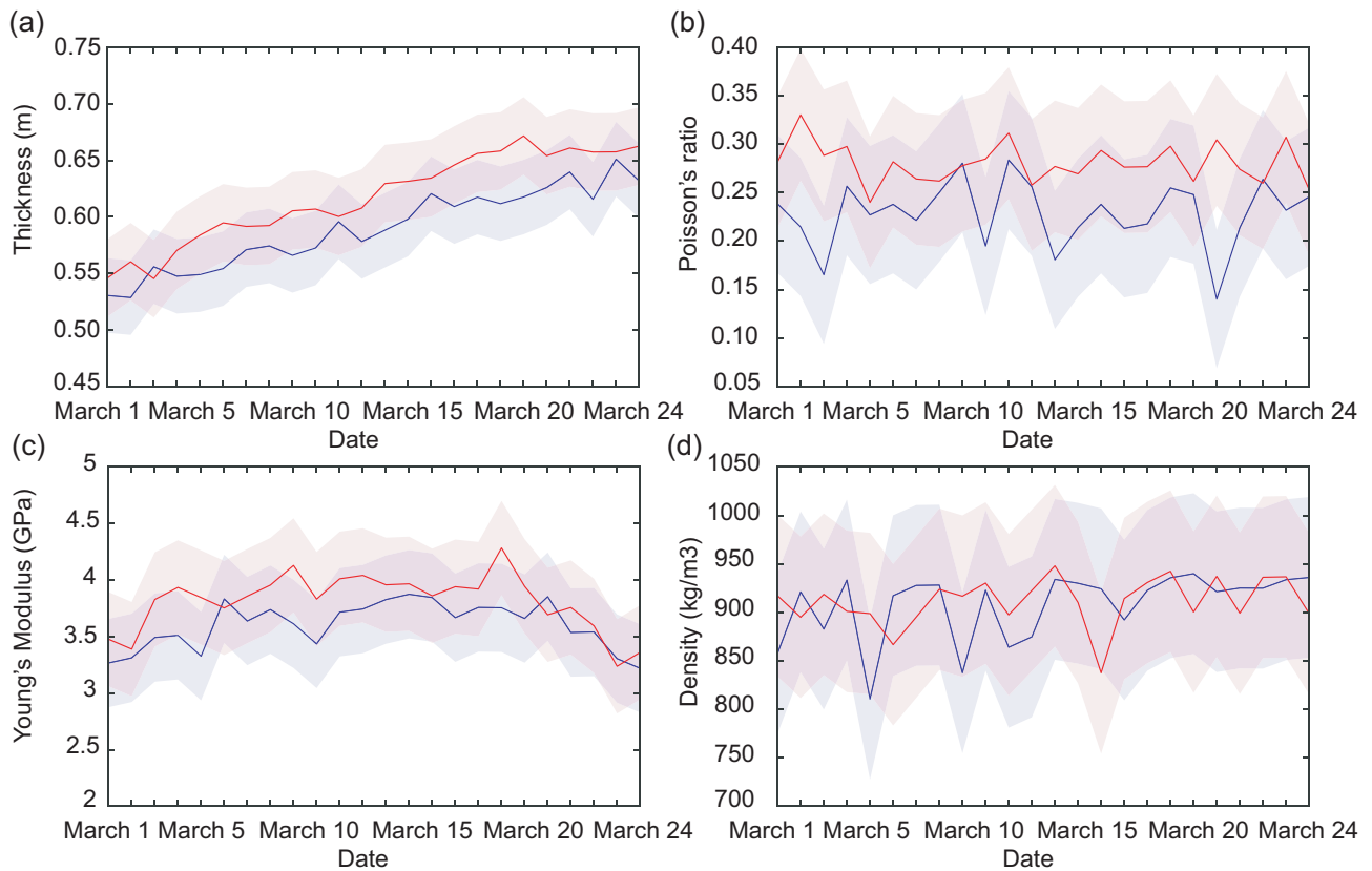
Figure 8. Daily evolution of the sea-ice parameters: (a) thickness, (b) Poisson's ratio, (c) Young's modulus, and (d) density, obtained for the lines of sensors in direction NS (blue) and EW (red). The coloured band represents the standard deviation associated with each of the curves. We observe an increase in the ice thickness in both directions, while the elastic parameters remain stable, around values that are consistent with the literature for first-year ice.
