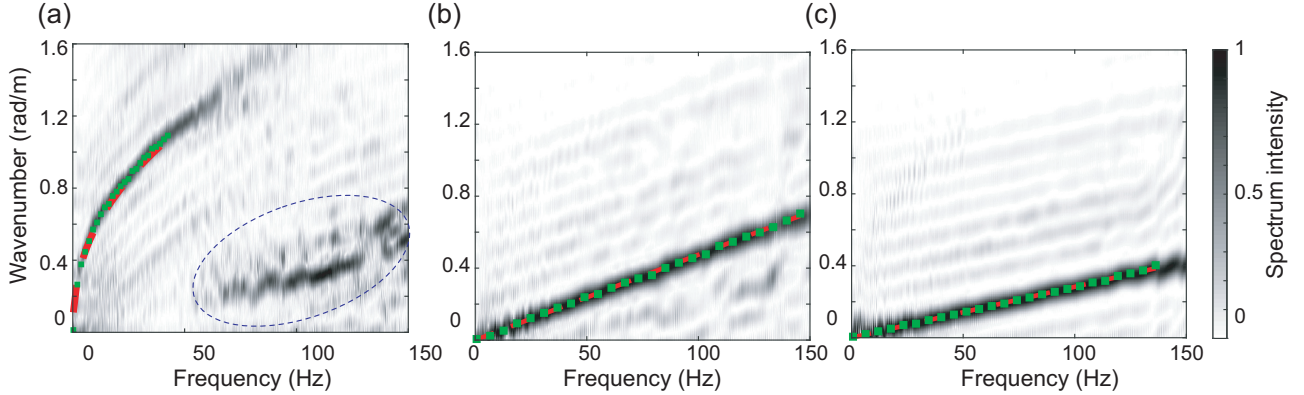
Figure 5. Frequency-wavenumber spectra obtained from the noise correlation function calculated on March 9, 2019, with the method described in section 2.2 and the processing of section 2.3, for recordings in the EW direction. (a) Spectrum from the vertical channel, dominated by the QS mode. The zone with a dotted contour highlights a seismic signature with slopes corresponding to a mix between the SH_0 and QS_0 modes. These modes appear on the vertical channel because the geophones were slightly tilted. (b) Spectrum from the radial channel, dominated by the QS_0 mode. (c) Spectrum from the transverse channel, dominated by the SH_0 mode. Green dots show the average of the dispersion curves extracted in the EW and WE directions. The red dotted lines show the dispersion curves obtained from Equations (1)-(3), with the sea-ice parameters inferred from Bayesian inference: E = 4.1 GPa, \nu = 0.28 , \rho = 917 kg/m 3 , and h = 0.60 m.
