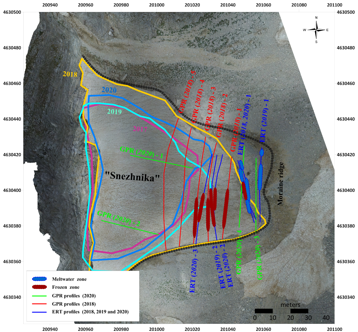
Figure 3. Location of the all GPR (red for 2018 and green for 2020) and ERT (blue) profiles in Snezhnika area. The size of the glacierret glacieret between 2017 and 2020 is given with lines in different colors. Bold red lines show the position of permafrost area, and bold blue lines show place of melt water (subsurface drainage system). The background picture, as well as moraine ridge outline (black line) , is made with the UAV in 2018 in the same day of measurements.
