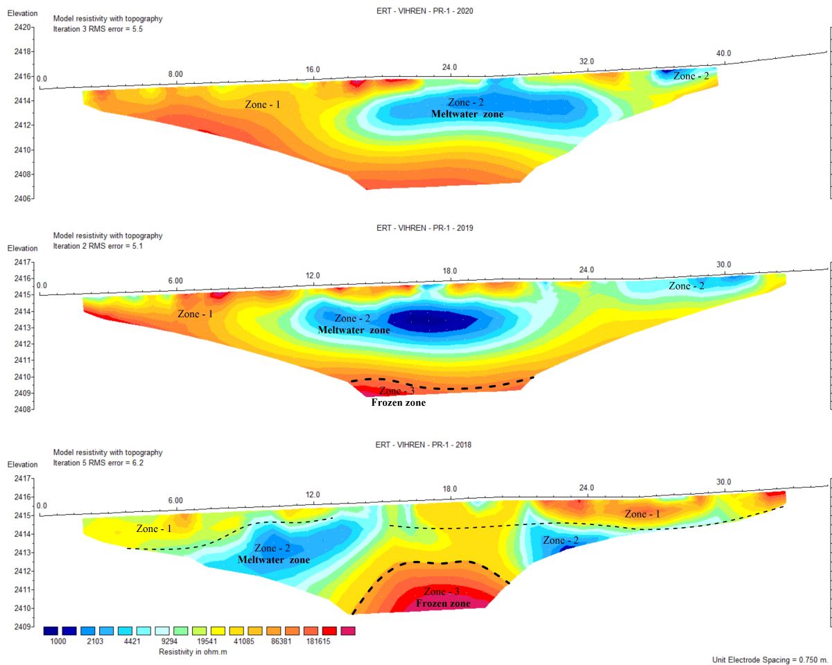
Figure 6. Electrical resistivity sections along ERT-1 obtained near Snezhnika microglacier in 2020 (a), 2019 (b) and 2018 (c). Blue color represents low resistivities and red color indicates areas with very high resistivities.
