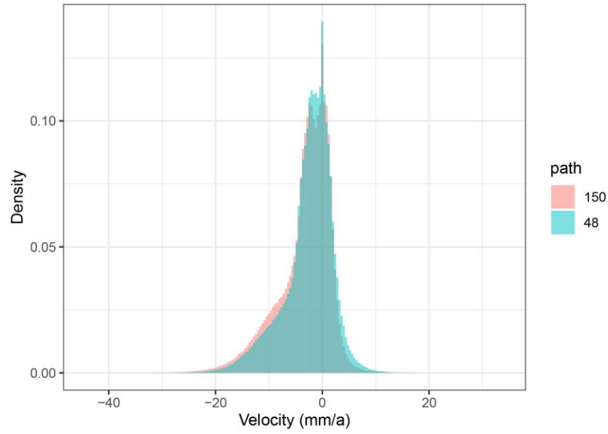
Fig. A4 The distribution of long-term velocity values in the satellite LOS direction from orbit 48 and orbit 150 in their overlapping area.
