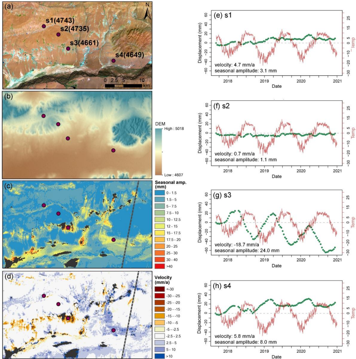
575 Figure 13 Deformation characters. This sector is marked with the red rectangle in Fig. 1 and 7-8. (a) Landsat 8 580 image (red: SWIR1, green: NIR, blue: red). (b) DEM overlapped on the hillshade, which is calculated using DEM with the Sentinel-1 incidence angle and azimuth angle. (c)(d) are seasonal deformation amplitude and long-term deformation velocity, respectively. The grey dashed line delineates the track boundary of orbit 150. (e)-(h) are deformation time series of marked sites. The elevation sites' elevation (m a.s.l.) of the sites are labeled in brackets in subfigure (a). Air temperature in red color is from ERA5-Land air temperature reanalysis data. Deformations are in the LOS direction.
