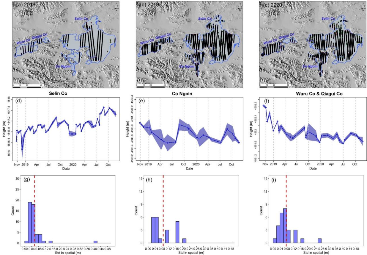
400 Figure 4 Water surface elevations of the three lakes. Subfigures (a)-(c) show tracks of the elevation measurements for each year. Subfigures (d)-(f) show the ICESat-2 derived elevations. The solid lines indicate the average values of all elevation measurements within the lake on a given date. The light-colored areas show the mean \pm one standard deviation. Subfigures (g)-(i) further show histograms of the standard deviations of the water surface elevation of the lake from all acquisition dates. The red dashed line indicates the mean value.
