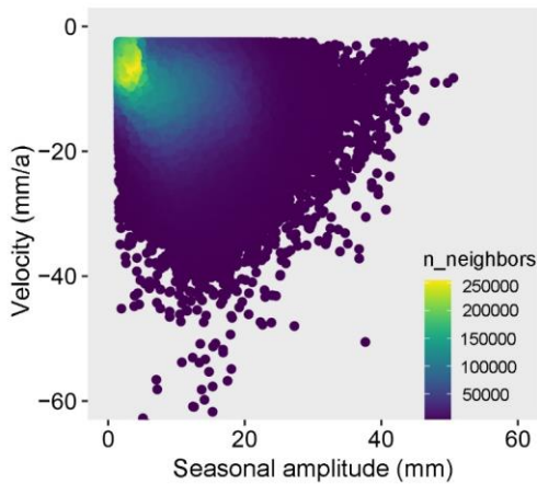
465 Figure 87 Distribution of the LOS seasonal amplitude versus the LOS deformation velocity within the Selin Co watershed, in all 6.57 \times 10^5 valid pixels.
