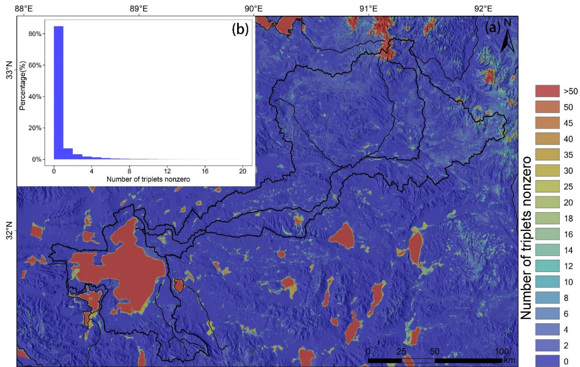
525 Figure 119 (a) Map of the number of interferogram triplets with nonzero integer ambiguity T_{int} (Eq(4)), (b) histogram illustrating the distribution of T_{int} values within the Selin Co watershed excluding glaciers and water bodies.
