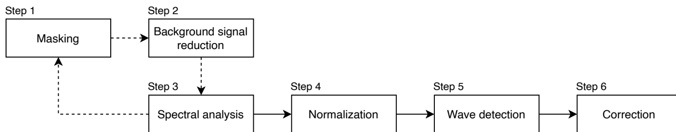
Figure 4. Steps of the wave detection algorithm TeRACWA (Terrestrial Radar Assessment of Calving Wave Activity). Steps linked by dashed and solid arrows are respectively applied to each TRI acquisition and to the resulting data set.
