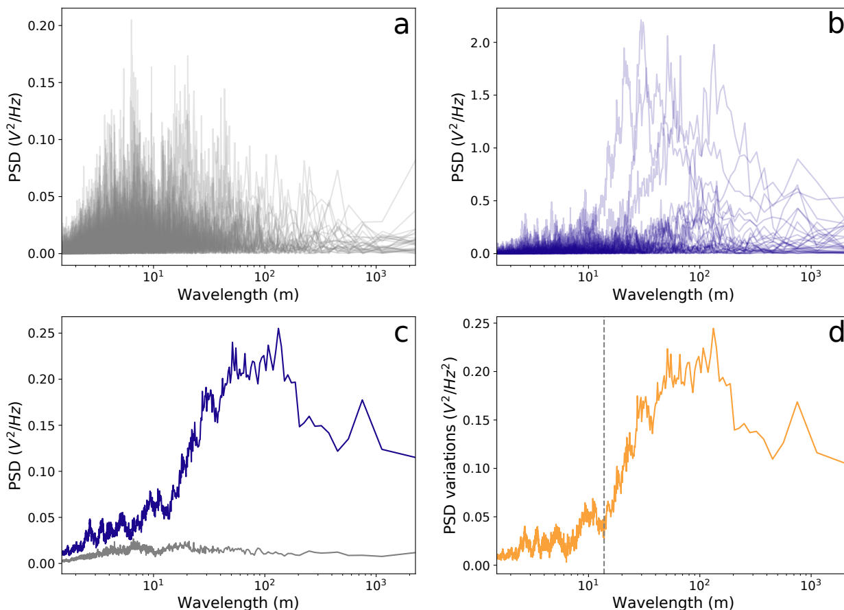
Figure 3. Determination of the frequency high-cutoff by analysing the power spectra of (a) 30 random background signals and (b) 30 wave signals. (c) Power spectral density (PSD) averages for the selected background (gray) and wave (blue) signals. (d) Difference between the two curves shown in (c). The gray dotted line indicates the cutoff wavelength (13.7 m).
