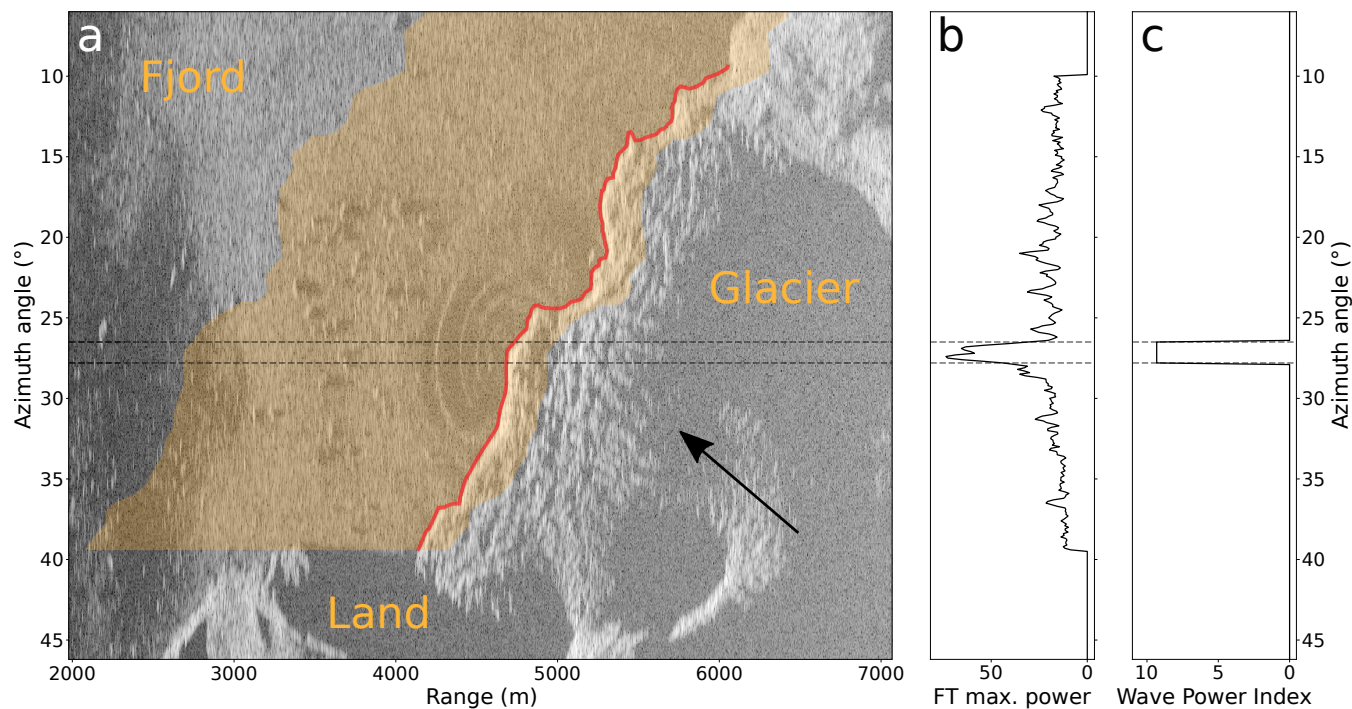
Figure 2. Example of calving wave detection. (a) Radar image of July 7, 2018 at 06:21:00 UTC represented as the logarithm of the signal strength. The black arrow indicates the ice flow direction, and the red line the outline of the glacier front. The translucent orange area shows the region of interest (ROI). (b) Maximum power of the Fourier transform by azimuth line obtained after the spectral analysis (step 3). (c) Wave power index (WPI) computed by TeRACWA (step 6). The two dashed lines indicate the boundaries of the wave detection on panels (a) and (b). The part of the calving front in between the lines corresponds to the wave source area.
