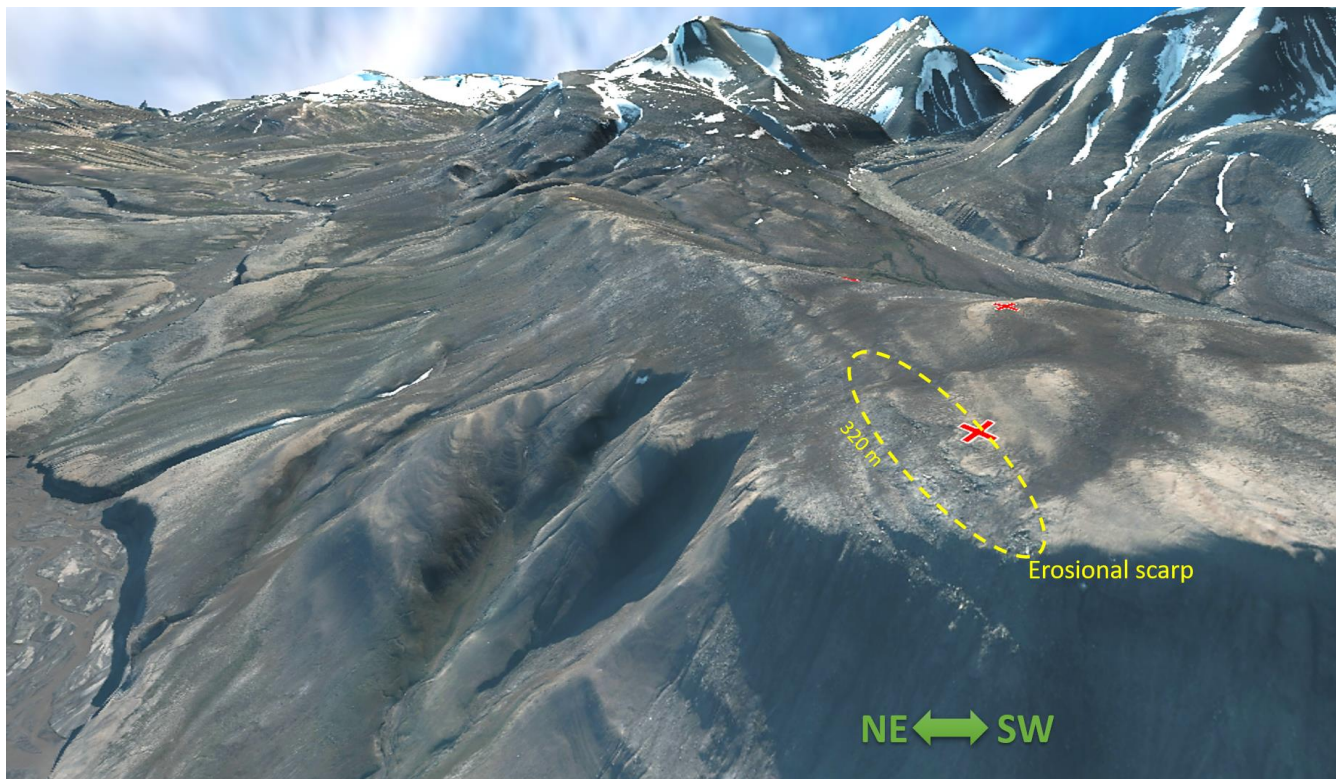
535 Figure A2 - 3D perspective view of the north-eastern flank of Janssonhaugen highlighting the third area associated with anomalous seismicity. The 3D model was constructed by draping an orthophoto on top of a 1.5x vertically exaggerated DEM. Red crosses mark locations of SPITS seismometer stations. Orthophoto/DEM © Norwegian Polar Institute (npolar.no).
