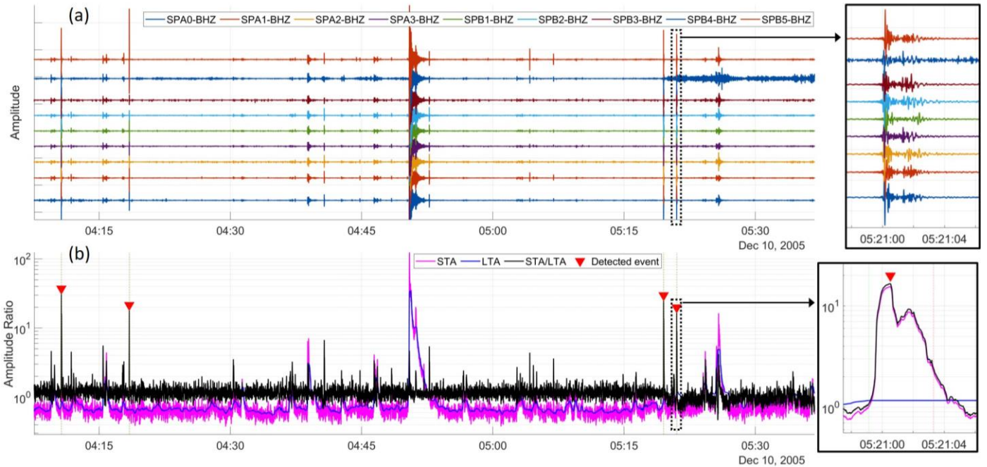
Figure 4 – Example of (a) timeseries of vertical component ground motion and (b) event detection using the STA/LTA detector. Short duration events with sufficient amplitude and array coherence are selected while longer events such as the high amplitude example at 04:50 are ignored. Inset boxes show detailed views for a specific detection.
