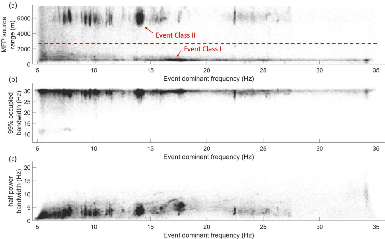
565 Figure C1 - Illustration of relationship between dominant frequency estimated by Thomson's multitaper spectral amplitude peak and (a) MFP estimated range to source, (b) bandwidth containing 99% of signal power estimated from periodogram power spectral density and (c) half-power bandwidth determined as the frequency range where power spectral density is within 3 dB of the maximum. The two event classes are most readily identified by the range to source, as annotated by the red dashed line.
