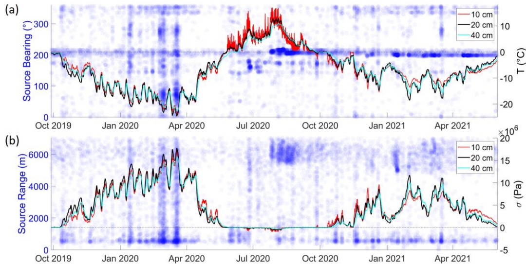
425 Figure 10 – (a) Ground temperature profiles (solid lines) and bearing (clockwise from North) to coherent MFP localised source positions from centre of SPITS array (blue circles). (b) modelled ground thermal stress from Eq. (12) (solid lines) and ranges to coherent MFP localised sources (blue circles). Source ranges and azimuths are transparent such that denser colours represent clusters of events.
