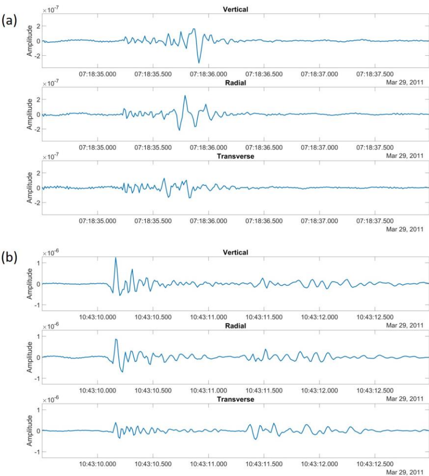
575 Figure C2 - Three-component seismograms from SPITS station SPA0 for (a) an example of event Class I (frost quake) and (b) an 580 example of event Class II (Gruve 7 mining activity). The signals are bandpass filtered to 2.5-35 Hz and the horizontal components of ground motion (measured in NS and EW orientations) were rotated to radial and transverse to the source bearings estimated by MFP (see Figure 5e and Figure 5f).
