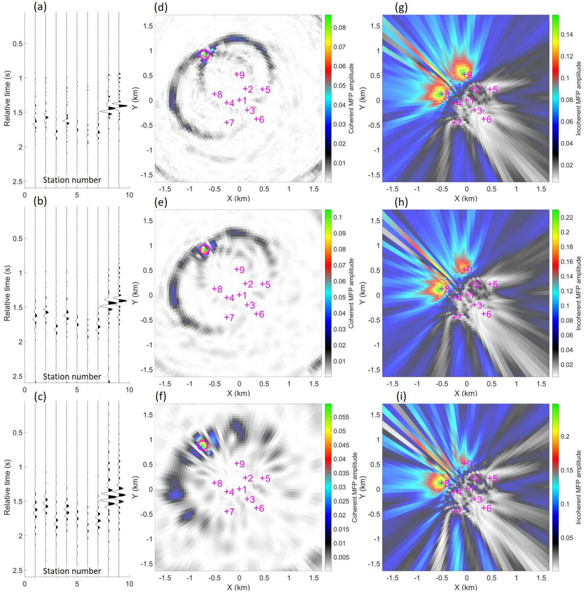
Figure D1 - Example of MFP source location for an event with dominant frequency of 10.2 Hz and half-power bandwidth of 6.7 Hz 590 (same event as shown in Figure 5b) filtered to passbands of (a) 5-35 Hz, (b) 5-15 Hz and (c) 7.5-12.5 Hz prior to MFP. (d), (e) & (f) show corresponding coherent MFP ambiguity surfaces while (g), (h) and (i) show incoherent MFP ambiguity surfaces.
