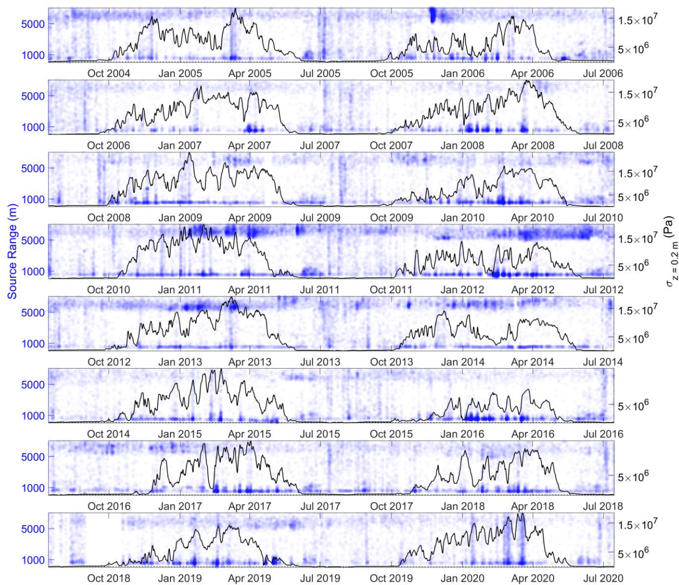
455 Figure 12 – Modelled thermal stress from Eq. (12) at 0.2 m depth (black lines) and ranges to coherent MFP localised sources (blue circles). Source ranges and azimuths are plotted as transparent points such that denser colours represent clusters of events. Event Class I & II are associated with small (<1500 m) and large (>5000 m) source ranges, respectively.
