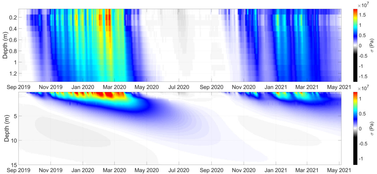
Figure 9 – Illustration of spatiotemporal thermal stress field modelled according to Eq. (12) and constrained by temperature measurements recorded by sensors installed at Janssonhaugen Vest (0.1 m) and in the P11 borehole (0.2-15 m). The temperature-depth profile used to calculate thermal stress was interpolated to regular 10 cm intervals using a spline interpolant. Sign convention is positive for tensional stress.
