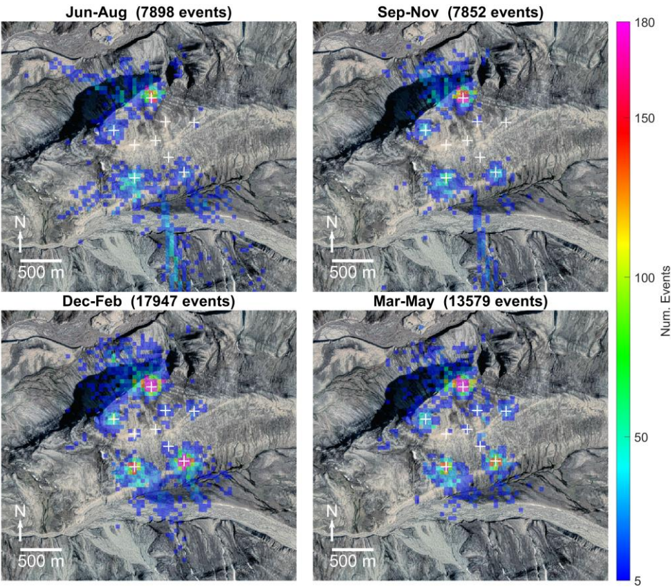
370 Figure 7 – Detail view of Janssonhaugen overlaid with spatially binned (50×50 m) distribution of coherent MFP inferred seismic source positions plotted by season for events recorded between August 2004 and July 2021. Positions of SPITS seismometers are indicated by white crosses. Orthophoto © Norwegian Polar Institute (npolar.no).
