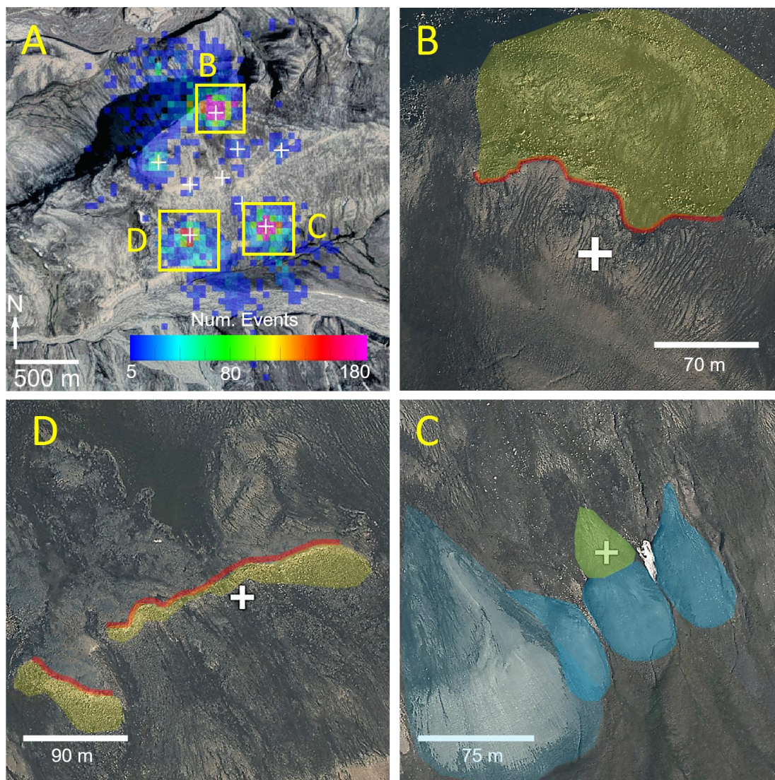
Figure 8 – (a) Dec-Feb events as plotted in Figure 7 with orthophotograph details illustrating the geomorphologic features associated with the most seismically active areas. Erosional scarps (b), (d) are annotated in red and associated boulder fields in yellow, and frozen debris/solifluction lobes (c) are annotated in blue. A faintly visible area of polygonal patterned ground is annotated in green in (c). Orthophoto © Norwegian Polar Institute (npolar.no).
