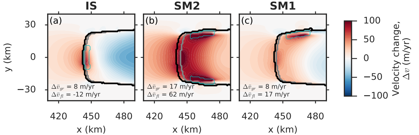
Figure 6. Change in ice speed \Delta v (colorbar) in the vicinity of the grounding line at the end of the 100-yr perturbation for the three different perturbation types and an applied melt-strip width of w = 4 km. In each panel the spatial mean of the grounded and floating speed changes (average over the displayed area), \Delta \bar{v}_{gr} and \Delta \bar{v}_{fl} , respectively, are given in the lower left corner. Thick contours represent the grounding-line position in the initial state (grey) and in the perturbed states (black). The thin cyan contour denotes the perturbation area. Note that the total melt rate P is 2 Gt/yr in the IS and SM2 cases and 1 Gt/yr in the SM1 case for a better comparability between the SM1 and SM2 cases. The pattern of changing ice-speed is shown for further time slices in Fig. S7.
