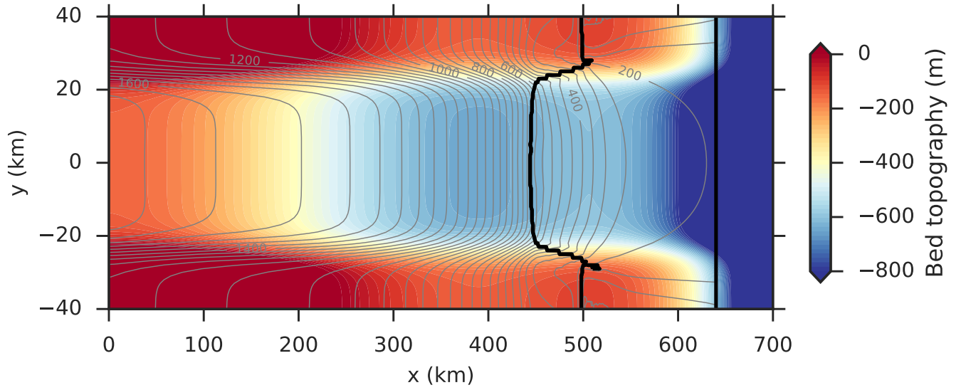
Figure 1. (a) Top view of channel-type bed topography (Asay-Davis et al., 2016; Cornford et al., 2020) used in this study. It is characterized by an overdeepening (retrograde bed section) in x -direction on which the spun-up grounding line stabilizes. (b) Centerline-profiles (along dotted line of panel (a)) of the spun-up ice-sheet-shelf system (grey) and has a stable steady-state position. Gray contours represent ice thickness in 50-m steps. The fixed calving front is shown by the underlying bed topography (straight black) contour at x = 640 km.
