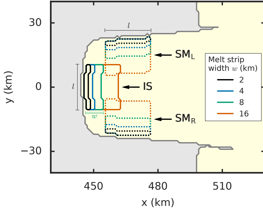
Figure 3. Region Ice-shelf regions IS, SM_L and spatial extent (colored contours) of SM_R in which the basal-melt basal melt perturbations are applied in the three types of experiments (zoom into grounding-line region). While all perturbation areas have the same length l along the grounding line, their width w is varied in the simulations (colored contours). The steady-state grounding line is represented by the dark grey contour, the ice sheet is colored light gray, the floating ice shelf is colored yellow. Continuous and dotted contours are used for better distinguishability between the central and lateral melt regions.
