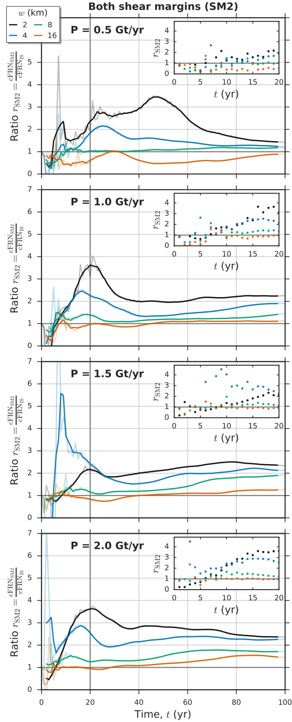
Figure 7. Time evolution of the cFRN ratios r_{SM2} and r_{SM1} for the two shear-margin-perturbation experiments (columns), respectively, the four perturbation strengths P (rows) and the four melt strip widths w (colors given in the legend). The curves show the 5-year running mean of the yearly data (light colors). For each panel the yearly data points for the first 20 model years are shown in the corresponding inset. A comparison to the qualitatively very similar curves of r_{SM1} is given in Fig. S8.
