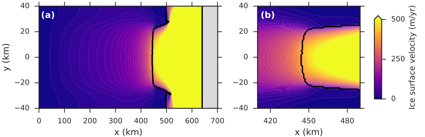
Figure 2. Steady-state ice surface speed (colorbar) for (a) the entire model domain and (b) the grounding-line region. Grounding line and calving front represented by black contours.
