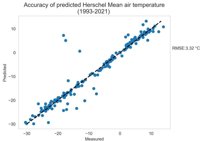
640 Figure A1: result from linear regression between air temperature measured on Herschel Island and predicted value using Burn and Zhang 2009 equation.
