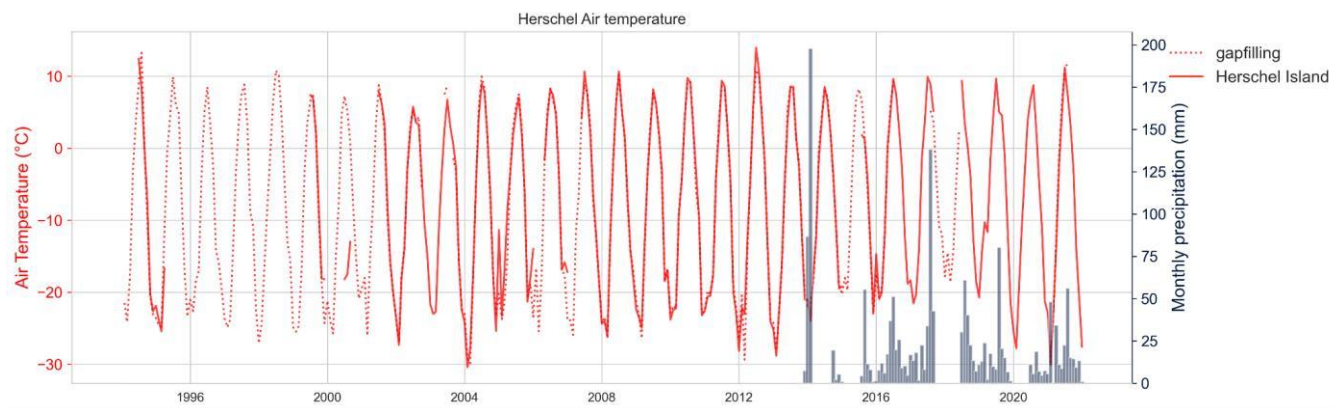
645 Figure A2: Comparison during 1994-2022 air temperature measured on Herschel Island and predicted value using Burn and Zhang 2009 equation.
