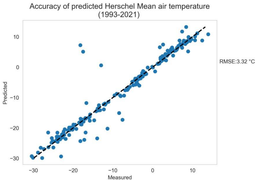
635 Figure A1: result from linear regression between air temperature measured on Herschel Island and predicted value using 640 Burn and Zhang 2009 equation.
