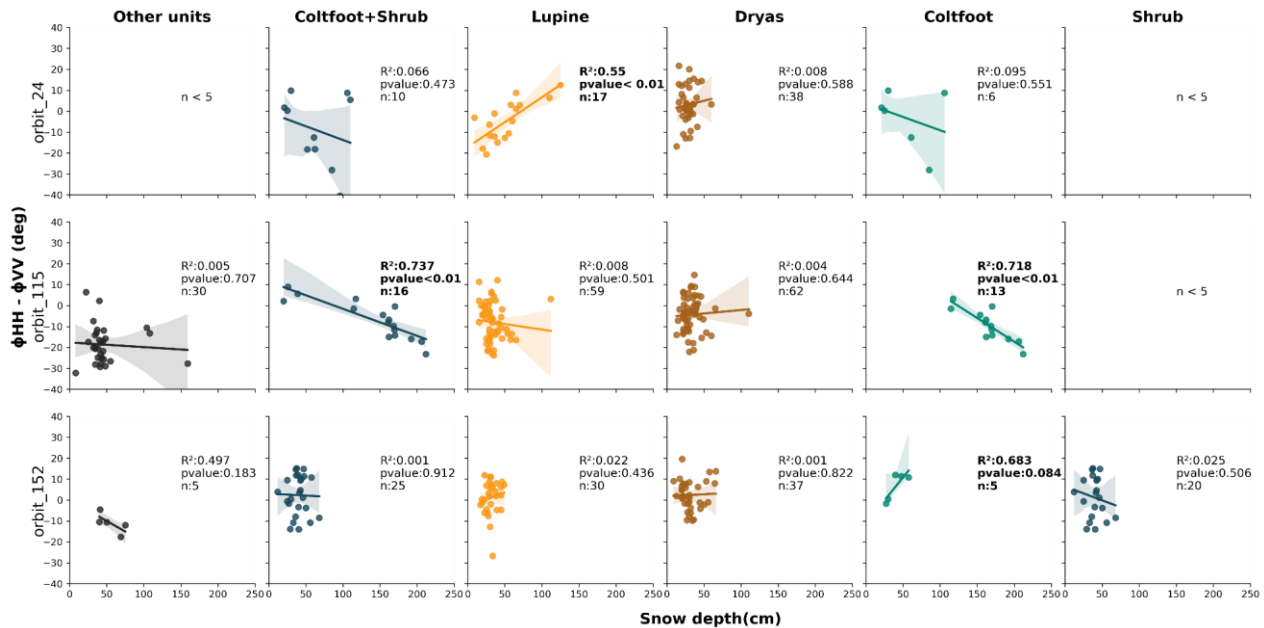
Figure 6. Correlation analysis between CPD and snow depth.
