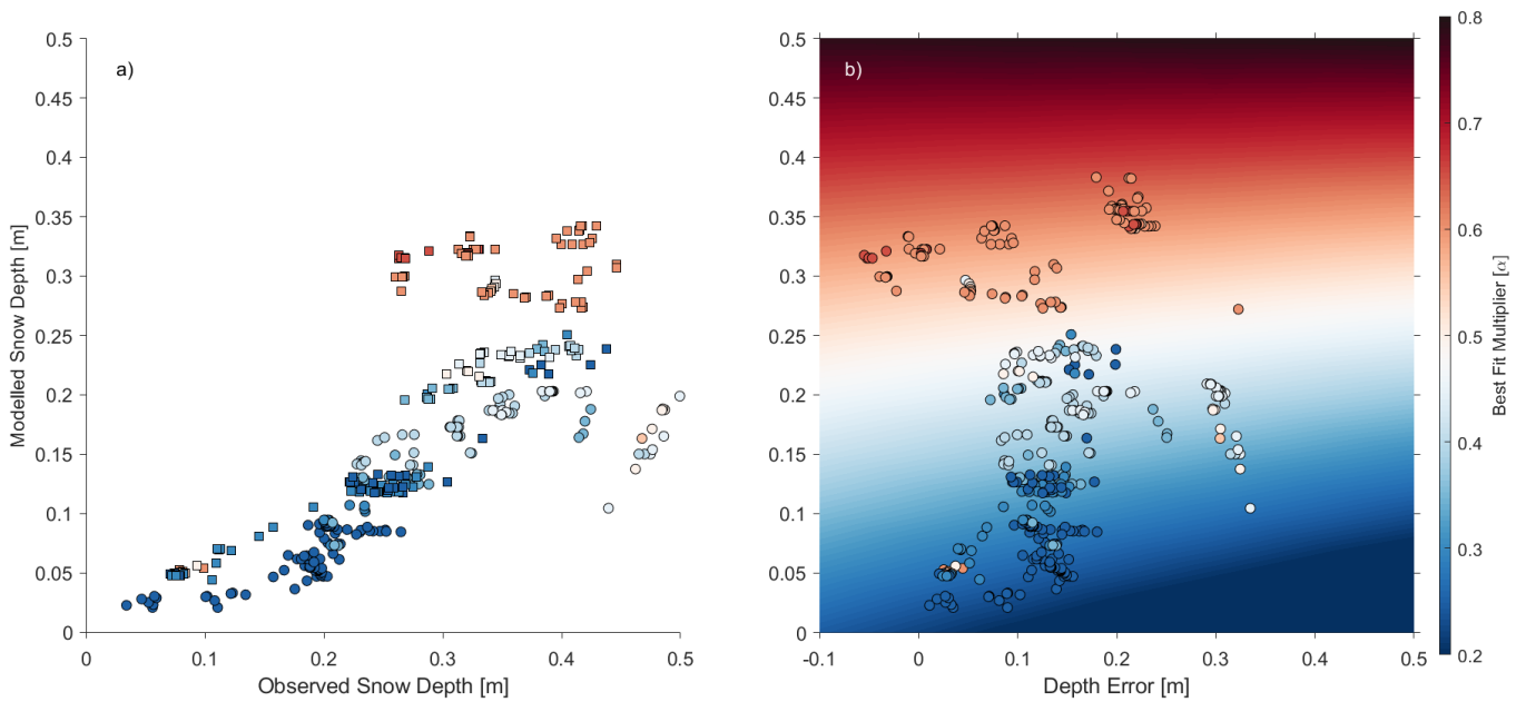
840 Figure 8: Influence of observed (x-axis; a) and modelled (y-axis; both) snow depth and snow depth error (x-axis; b) on the best fit correction (colour) at each timestep for both the 2017-18 (circles) and 2018-19 (squares) snow seasons.
