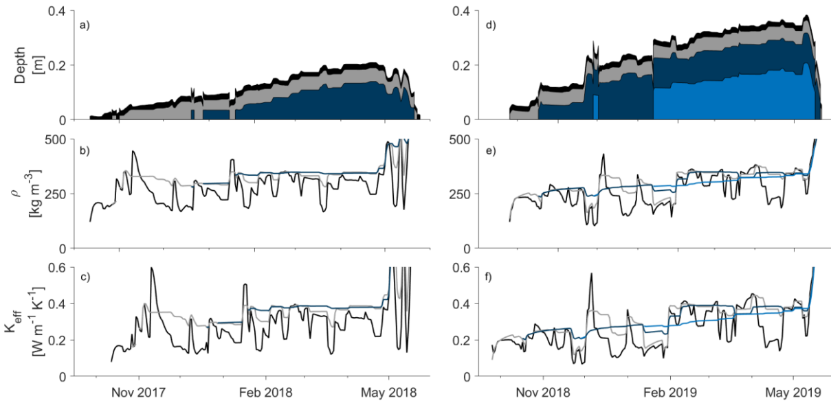
Figure 5: Simulated snow layers and their properties for winter 2017-18; a) simulated snow layer thicknesses, b) snow layer densities, c) snow layer thermal conductivities; d) to f) as before but for winter 2018-19. Each colour represents a different computational snow layer.
