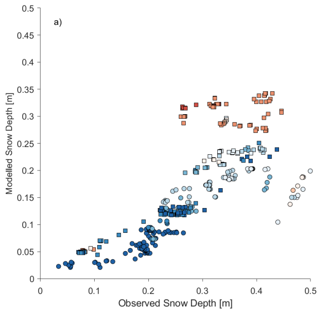
Figure 89: Influence of observed (x-axis; a) and modelled (y-axis; both) snow depth and snow depth error (x-axis; b) on the best fit correction (colour) at each timestep for both the 2017-18 (circles) and 2018-19 (squares) snow seasons.
