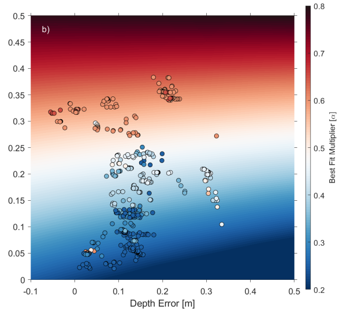
Figure 89: Influence of observed (x-axis; a) and modelled (y-axis; both) snow depth and snow depth error (x-axis; b) on the best fit correction (colour) at each timestep for both the 2017-18 (circles) and 2018-19 (squares) snow seasons.
