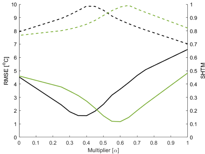
Figure 8: Changes to model performance when adjusting snow thermal conductivity, measured using RMSE of 10cm soil temperatures (solid lines) and the Snow Heat Transfer Metric (SHTM—dashed lines) for the 2017-18 (black) and 2018-19 (green) snow seasons.
