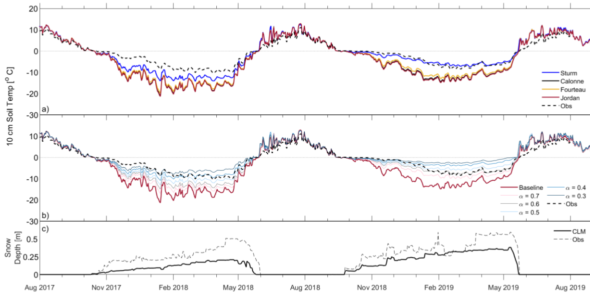
Figure 7: a) Timeseries of 10cm soil temperatures for K_{eff} sensitivity tests compared to field measurements, ab) Simulated 10cm soil temperature timeseries using the 4 different both Jordan (1991) and Sturm et al (1997) parameterisations of snow thermal conductivity compared to field measurements, b) Timeseries of 10cm soil temperatures when using different values of the correction factor \alpha compared to field measurements, -ec) Observed and simulated snow depths for the same time period.
