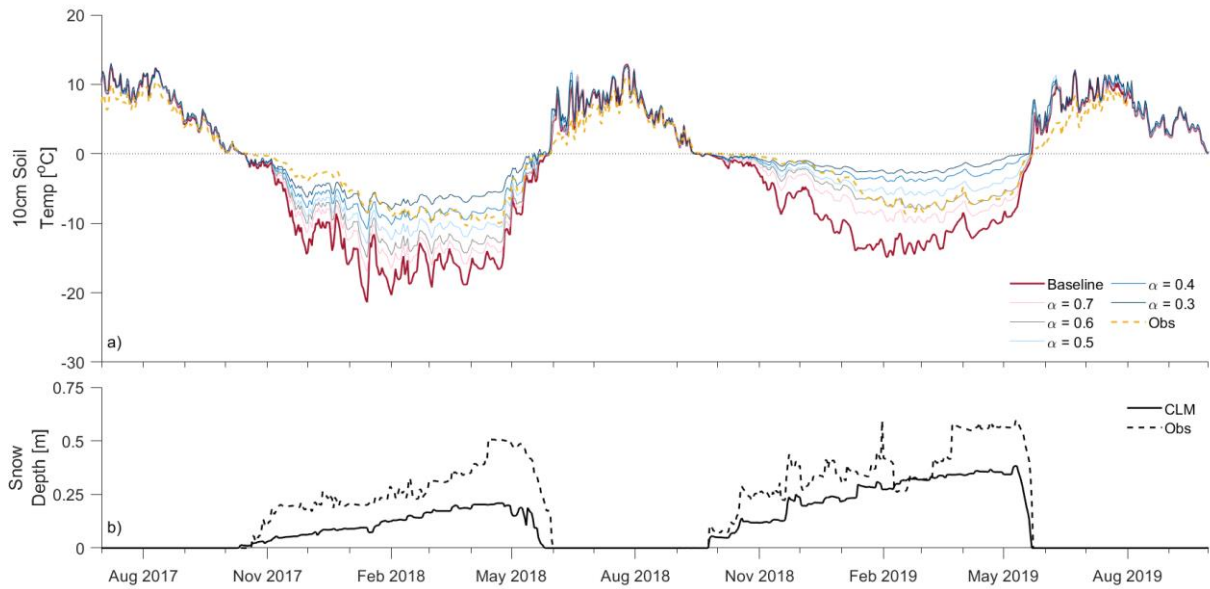
Figure 8: a) Timeseries of 10cm soil temperatures timeseries for K_{sat} sensitivity tests compared to field measurements, b) Observed and simulated snow depths for the same time period.
