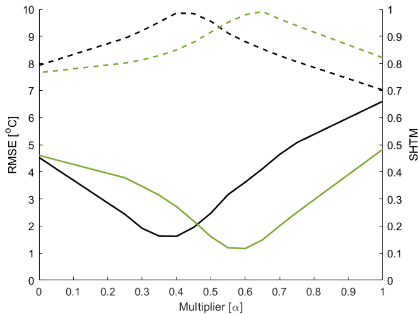
Figure 87: Changes to model performance when adjusting snow thermal conductivity, measured using RMSE of 10cm soil temperatures (solid lines) and the Snow Heat Transfer Metric (SHTM – dashed lines) for the 2017-18 (black) and 2018-19 (green) snow seasons.
