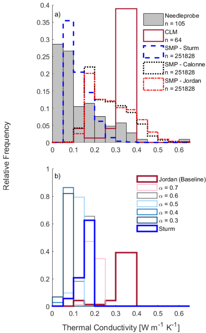
Figure 6: a) Histograms of measured and simulated thermal conductivity from March 2018 and 2019 sampling campaigns, b) Sensitivity testing of simulated thermal conductivities for the same time period using both the default CLM snow thermal conductivity parameterisation and the Sturm (1997) parameterisation. Note the different scales on the y-axes. a) Histograms of measured and simulated thermal conductivity from March 2018 and 2019 sampling campaigns, b) Sensitivity testing of simulated thermal conductivities for the same time period. Note the different scales on the y-axes.
