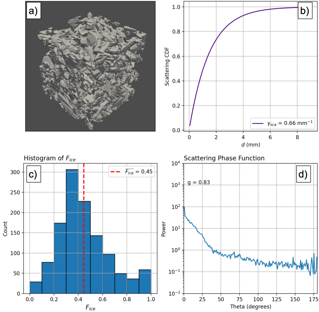
Figure 2. (a) 3D rendering of the snow sample used to generate the optical properties. (b) Cumulative distribution function of scattering as a function of distance (mm) and \gamma_{sca} . (c) Histogram of F_{ice} . The red dashed line indicates the mean value. (d) Scattering phase function. 1200 individual photon tracks were used to generate the optical properties shown in this figure. The asymmetry parameter ( g ) is the average of the geometric asymmetry parameter computed from the phase function as g_G = \frac{1}{2} \int p(\cos\Theta) \cos\Theta \sin\Theta d\Theta and the diffraction asymmetry parameter g_D \simeq 1 according to Kokhanovsky and Zege (2004) and Libois et al. (2013).
