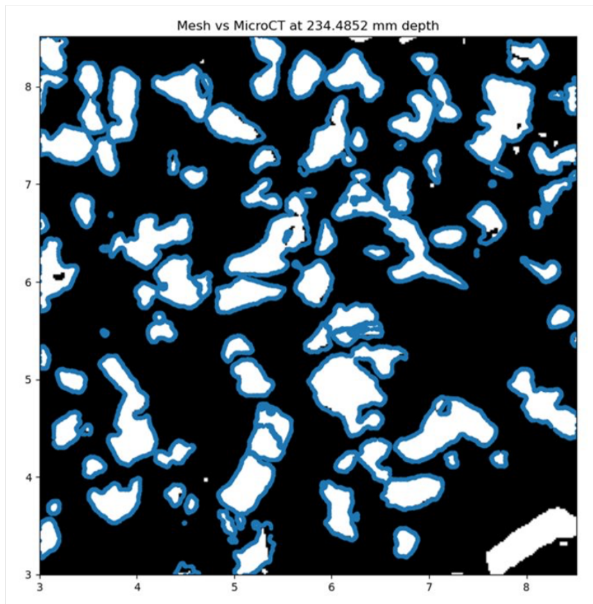
Figure 5. 2D Cross-sectional slice of a binarized \mu CT scan with corresponding mesh boundaries superimposed shown as the blue lines.
