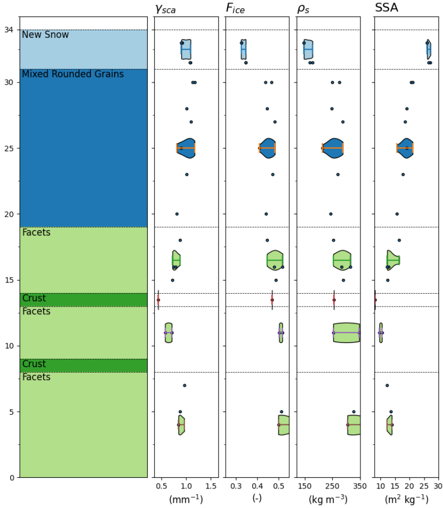
Figure 15. Snow pit stratigraphy (left) compared against \gamma_{sca} , F_{ice} , \rho_s , and SSA. Each dot represents a \mu CT sample at a specified depth. Violin plots show estimated probability distributions for each observer-identified snow layer according to the samples collected with the layer.
