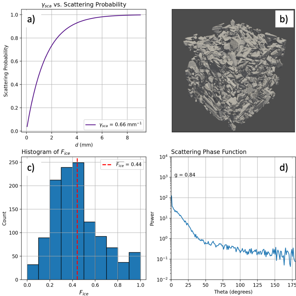
Figure 2. (a) Probability of scattering as a function of distance (mm) and \gamma_{sca} . (b) 3D rendering of the snow sample used to generate the optical properties. (c) Histogram of F_{ice} . The red dashed line indicates the mean value. (d) Scattering phase function. 1200 individual photon tracks were used to generate the optical properties shown in this figure. The asymmetry parameter ( g ) is the average of the geometric asymmetry parameter computed from the phase function as g_G = \frac{1}{2} \int \cos(\Theta) * \sin(\Theta) d\Theta and the diffraction asymmetry parameter g_D \simeq 1 according to Kokhanovsky and Zege (2004) and Libois et al. (2013).
