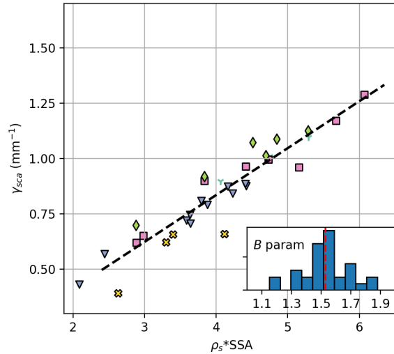
Figure 13. Optical properties for \lambda=1000 nm computed from \mu CT photon tracking compared against sample physical properties. a) F_{ice} vs. \rho_s and b) \gamma_{sca} vs. SSA \cdot \rho_s . Linear regression lines are shown in black dashed lines. Marker shapes and colors are indicative of the observed grain forms determined through visual assessment during snow pit analysis. Note that in panel (b) a histogram of the estimated B parameters for all of the \mu CT samples is shown, inset. B_{mean} = 1.53 is shown as the vertical red line.
