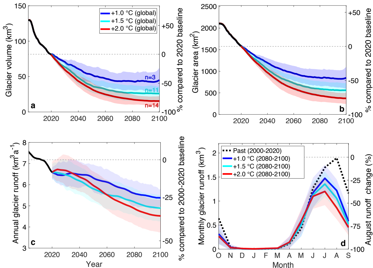
Figure 2. Modelled evolution of total glacier (a) volume, (b) area, (c) annual glacier runoff, and (d) monthly glacier runoff of the European Alps. Time series in c are smoothed with a 20-year running mean. In all panels, the thick line represents the mean and the transparent band corresponds to one standard deviation of the results obtained by forcing GloGEMflow with the selected GCM members. The numbers of GCM members is given ( n ).
