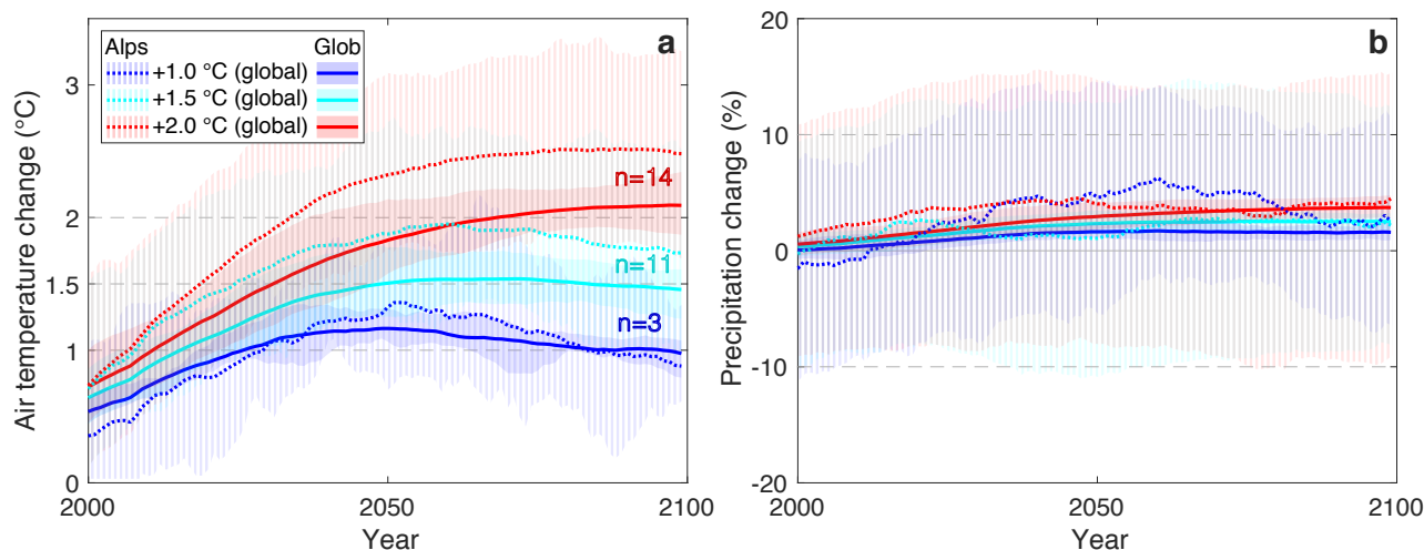
Figure 1. Evolution of annual global and Alpine (a) average air temperature and (b) precipitation total compared to the pre-industrial (1850-1900) baseline. Series are smoothed with a 30-year running mean. The coloured bands show the standard deviation of the projection given by individual GCM members. n is the considered numbers of GCM members.
