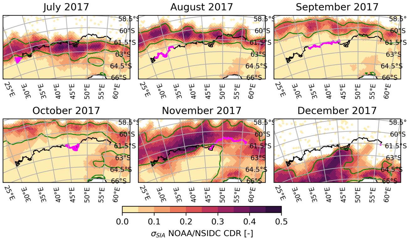
Figure 6. Trajectory of the ice-tethered, non-floating drifter studied by Womack et al. (2022) in winter 2017 (from 04-07-2017 to 01-12-2017, black line) overlain to the \sigma_{SIA} indicator field (shading) and the 0.15-0.80 SIC range (green contours) from the NOAA/NSIDC CDR. The magenta lines indicate the paths followed during each month.
