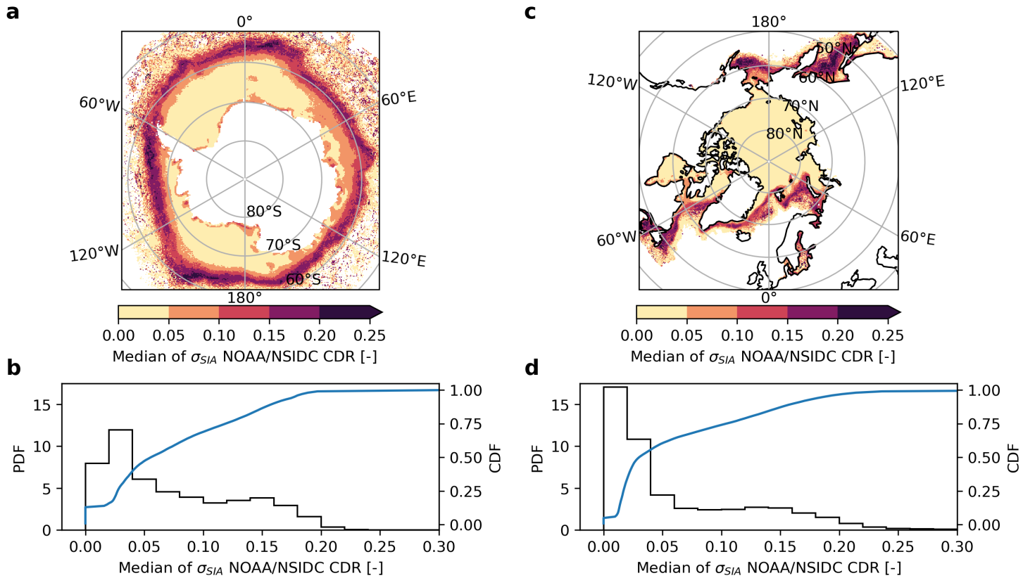
Figure 3. (a) Median of the \sigma_{SIA} indicator on a stereographic projection. The pixels with SIC=0 and \sigma_{SIA} = 0 have been excluded from the analysis. (b) Empirical probability and cumulative density functions of the median values from the map shown in panel a (PDF: black line and CDF: blue line). (c-d) same as (a-b) but for the Arctic. All data are from the NOAA/NSIDC CDR (1987-2019).
