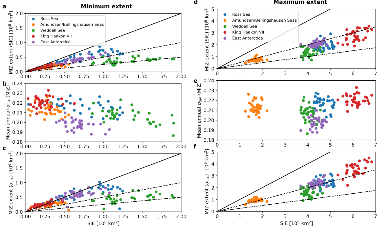
Figure 8. Relationship between the total minimum and maximum sea ice extent (SIE, x-axes) and three MIZ properties (y-axes) in the different sectors of the Southern Ocean for the years 1987-2019. a) minimum monthly MIZ extent computed using the 0.15-0.80 SIC mask criterion ; b) annual mean of \sigma_{SIA} , computed for the MIZ pixels where \sigma_{SIA}^m > 0.1 ; c) minimum monthly MIZ extent computed using the \sigma_{SIA}^m > 0.1 mask criterion. d-e-f) the same but for the maximum of each year. The lines represent the 100% (continuous), 50% (dashed) and 25% (dot-dash) MIZ fraction.
