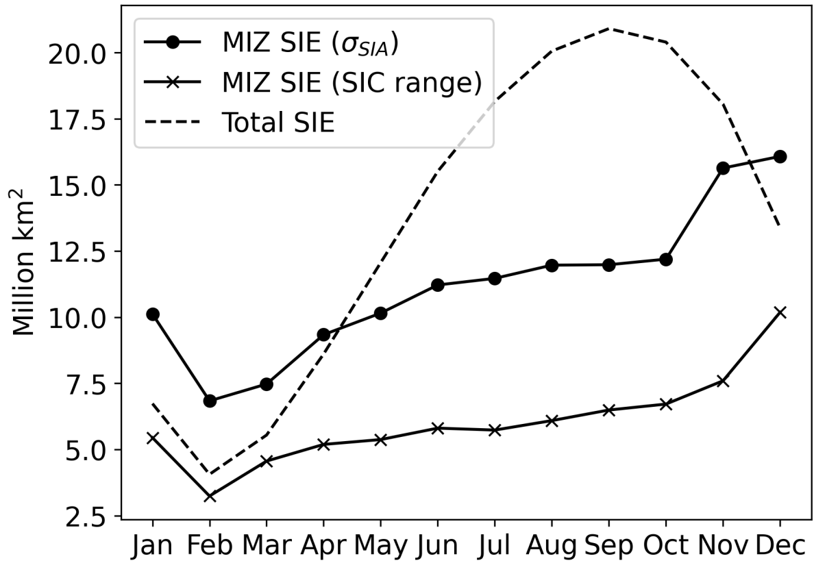
Figure 11. Estimated climatological extent of the MIZ and total sea ice extent computed from the monthly climatologies of NOAA/NSIDC CRD. The filled-circle line is obtained from the \bar{\sigma}_{SIA}^n indicator using the threshold 0.1, which also includes the coastal regions.
