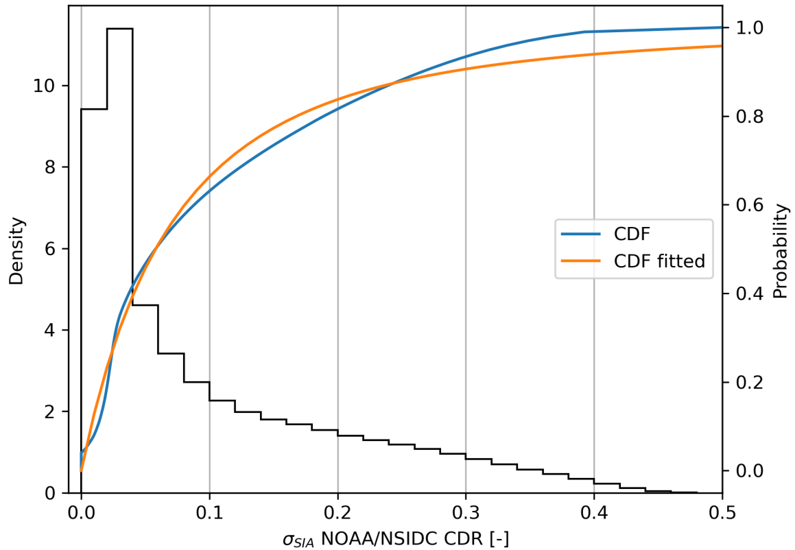
Figure 2. Empirical probability (black line) and cumulative (blue line) density functions of the \sigma_{SIA} indicator from the NOAA/NSIDC CDR data set. The orange curve is the fitted Pareto distribution.
