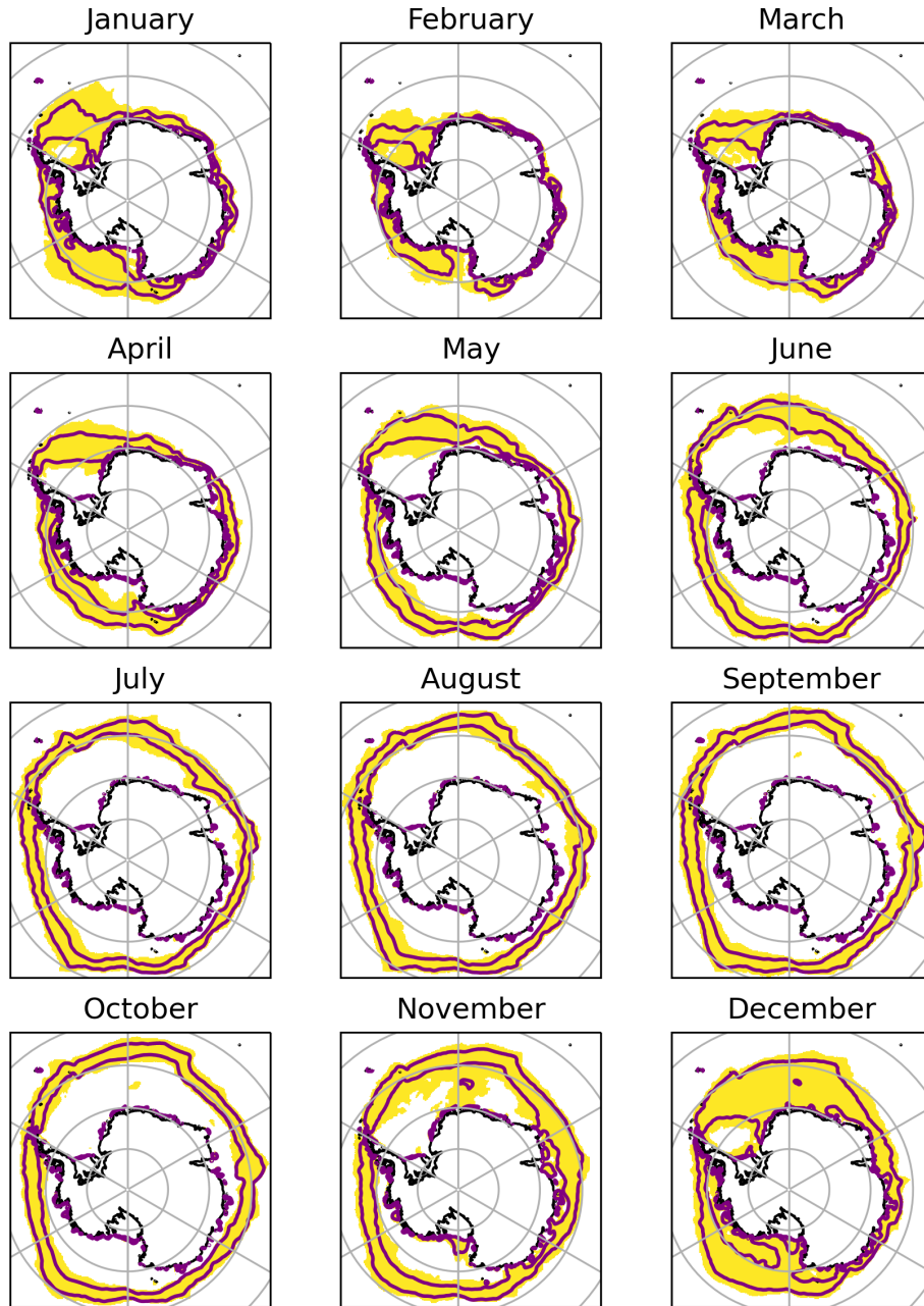
Figure 10. Climatological monthly mask of the MIZ obtained from the \bar{\sigma}_{SIA}^n indicator. The purple line indicates the MIZ extent computed using the SIC criterion.
