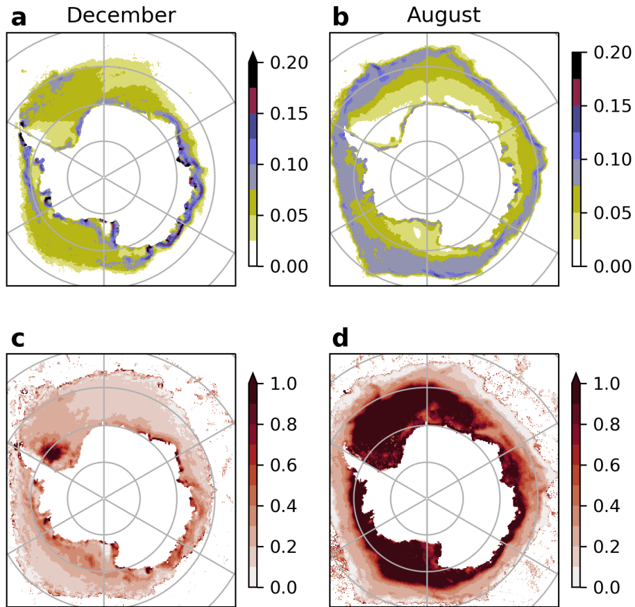
Figure 5. Comparison of the spatial and temporal variability for the NOAA/NSIDC CDR. a, b) climatological spatial standard deviation for the months of December and August; c, d) ratio between the spatial standard deviation shown in panels a and b and \bar{\sigma}_{SIA}^n for the same months of December and August. All the months are shown in Figure S4 of the supplementary material.
