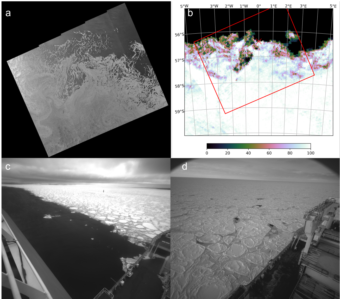
Figure 1. Example of sea ice conditions in the marginal ice zone at the edge with the ocean in austral spring and about 200 km into the pack ice in austral winter. (a) SAR image from the European Space Agency Sentinel 1B (GRD, acquired on 2019-10-21T19:21:53, obtained from http://www.seaice.dk at 300 m resolution, with credits to Roberto Saldo, dtu space and Technical University of Denmark). (b) Sea ice concentration from AMSR2 on the same day in stereographic polar projection (3.125 km resolution, processed by the University of Hamburg and obtained from ftp://ftp-projects.cen.uni-hamburg.de/seaice/AMSR2/3.125km ) showing the footprint of the SAR image and the location of the icebreaker SA Agulhas II in the morning of 2019-10-22. (c) Sea ice conditions before entering the MIZ at the location shown by the red cross in panel b. The sharp transition is the wake of the ship after reaching the sampling position. (d) Cemented pancake ice floes in austral winter (observed from the SA Agulhas II on 2019-07-27 at 0E, 57S).
