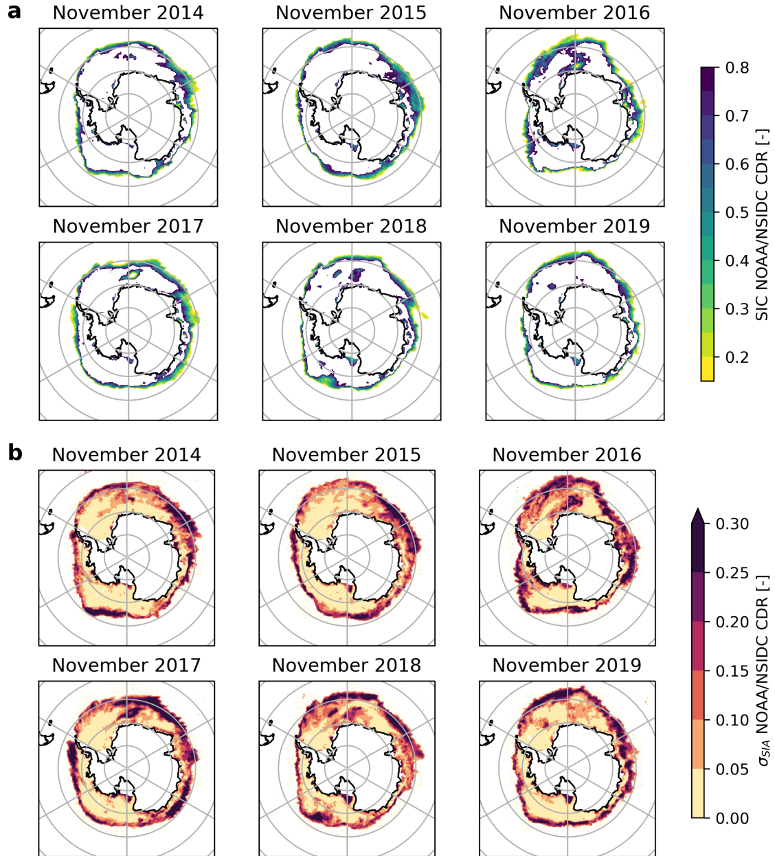
Figure 7. November maps of a) the mean SIC for the standard MIZ thresholds ( 0.15 \leq \text{SIC} < 0.80 ), and b) the \sigma_{SIA} indicator from the NOAA/NSIDC CDR for the years 2014-2019. Note the scale change with respect to Fig. 4. Years from 2008 to 2019 are shown in supplementary figures S5 and S6.
