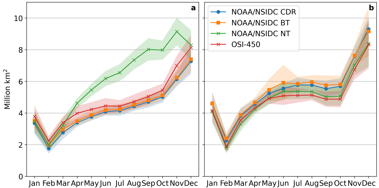
Figure 9. Seasonal cycle of the MIZ extent estimated from the a) SIC criterion ( 0.15 \leq \text{SIC} < 0.80 ) and b) the \sigma_{SIA} indicator ( \sigma_{SIA}^m > 0.1 ). The results are shown for all the products described in Sec. 2.1.
