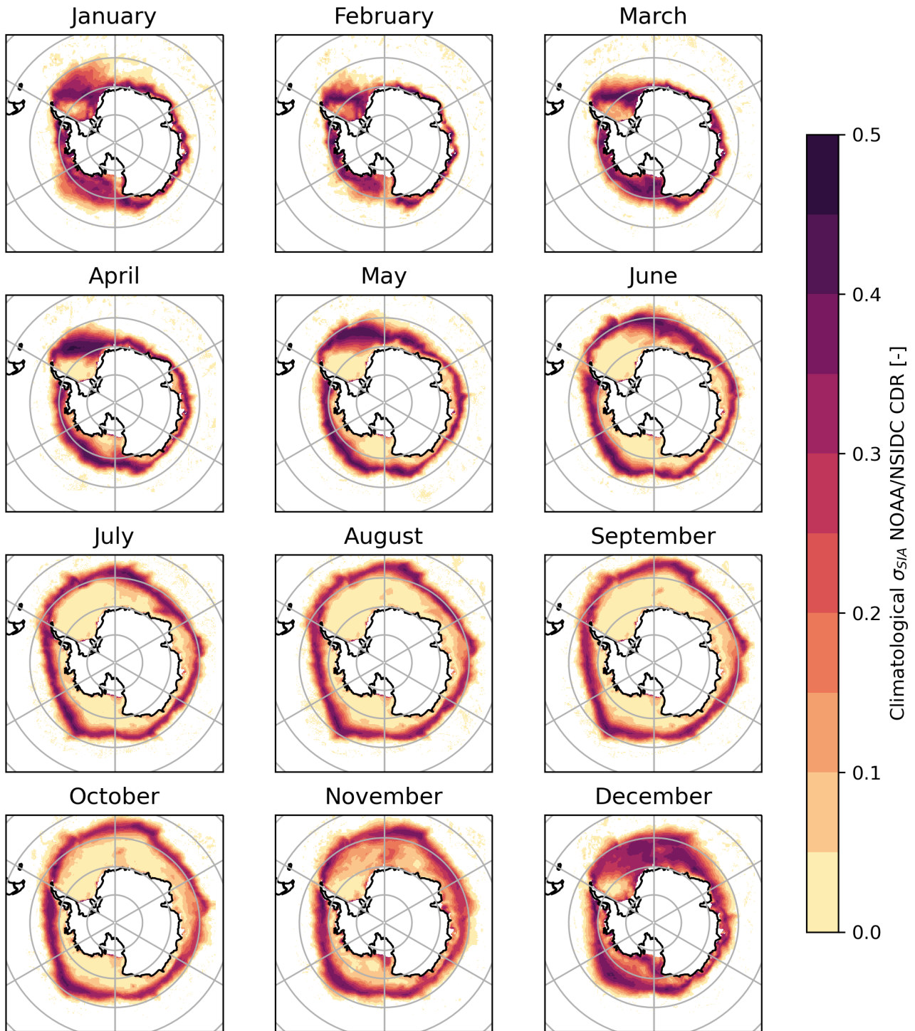
Figure 4. Climatological values of the indicator (\overline{\sigma}_{SIA}^n) , computed as the standard deviation of the daily anomalies for each month in the whole time series (see eq. 3).
