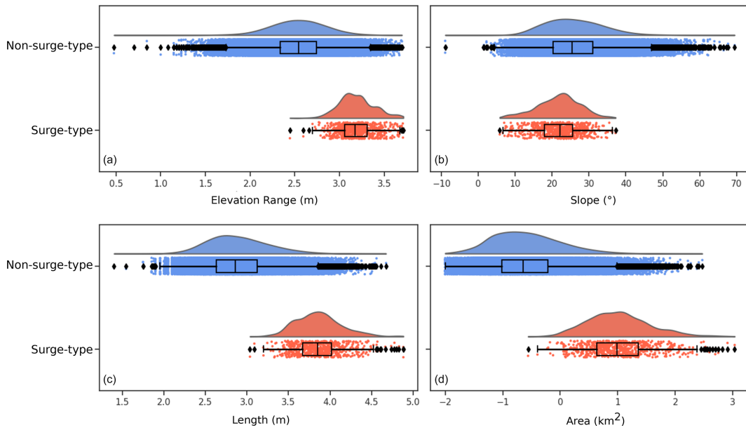
Figure 5. Distributions of geometrical attributes between non-surging and surge-type glaciers: (a) elevation range, (b) slope, (c) length and (d) area. Surge-type glaciers are represented in orange and non-surge-type glaciers in blue. L_{\max} is the length of the centreline of the longest glacier trunk of each RGI polygon. Area, length and altitude range are represented using common logarithms. Whiskers represent the 95th percentile of each distribution, while limits of the box represent 1 standard deviation.
