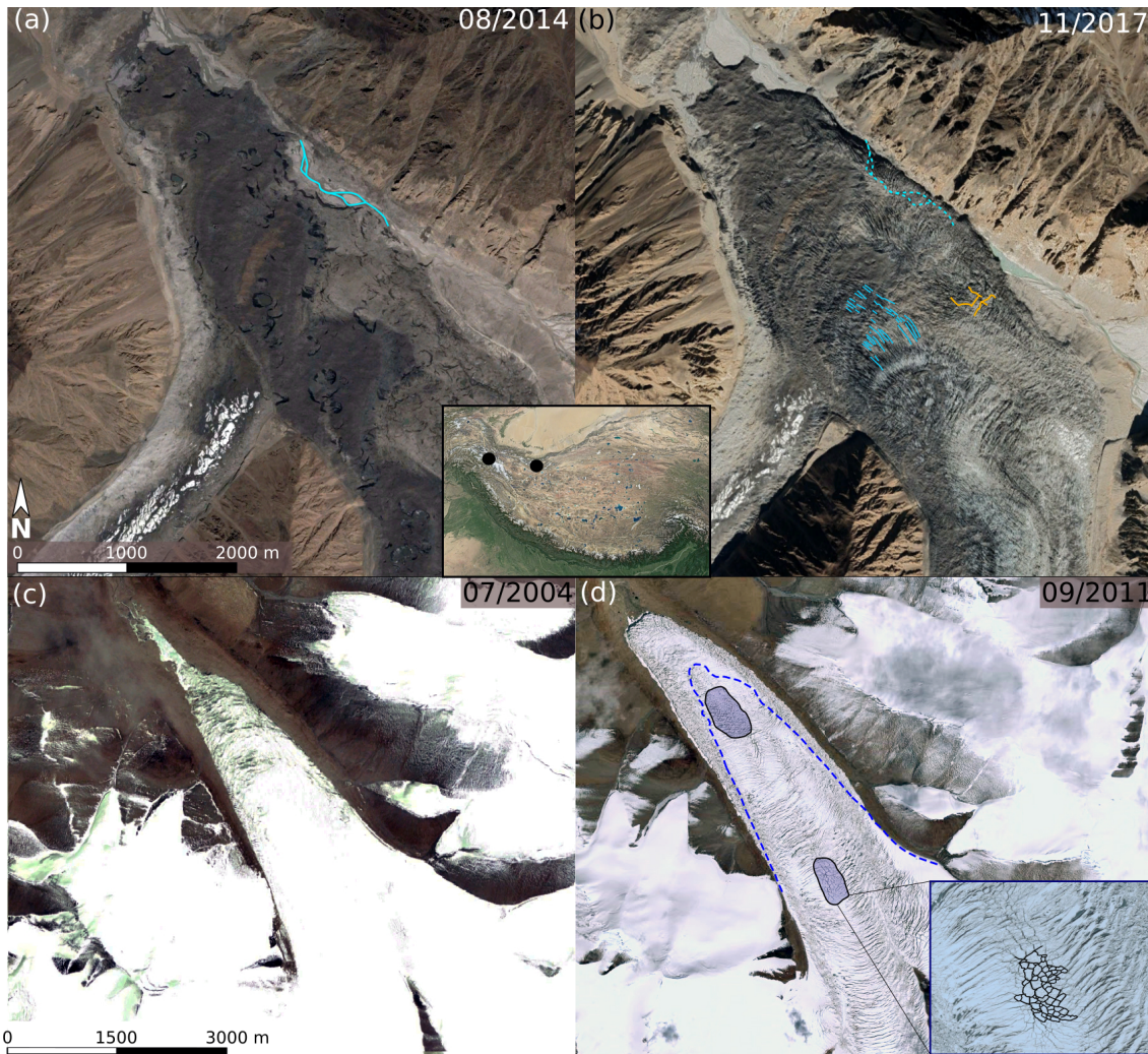
Figure 3. Google Earth imagery close-ups of surface features indicative of surges on debris-covered ( a, b : 2017 surge of Khurdopin Glacier, Hunza Basin, Karakoram) and clean ice glaciers ( c, d : 2008–2014 surge of N2 Glacier, West Kunlun Tibet, light blue CE3 ). ( a ) Khurdopin Glacier in August 2014 during the quiescent phase. Note the abundance of supraglacial ponds on the stagnant ice. Blue line: river bed. ( b ) Khurdopin Glacier in November 2017 during the active phase (peaking in May 2017) (Steiner et al., 2018). The surface is heavily crevassed with longitudinal (blue lines) and intersecting crevasses (yellow). The blue dashed line represents the location of the river bed in panel ( a ). ( c ) N2 glacier in a quiescent phase in 2004. ( d ) N2 Glacier in 2011 after active-phase peak (August 2009–November 2010) (Yasuda and Furuya, 2015). The blue dashed line represents the position of the glacier terminus in 2004. Note the substantial terminus advance and the two zones (blue polygons) of rhombic crevasse patterns, indicative of surge-type behaviour (Herzfeld and Zahner, 2001; Herzfeld et al., 2004). © Google Earth 2021 and © Microsoft.
