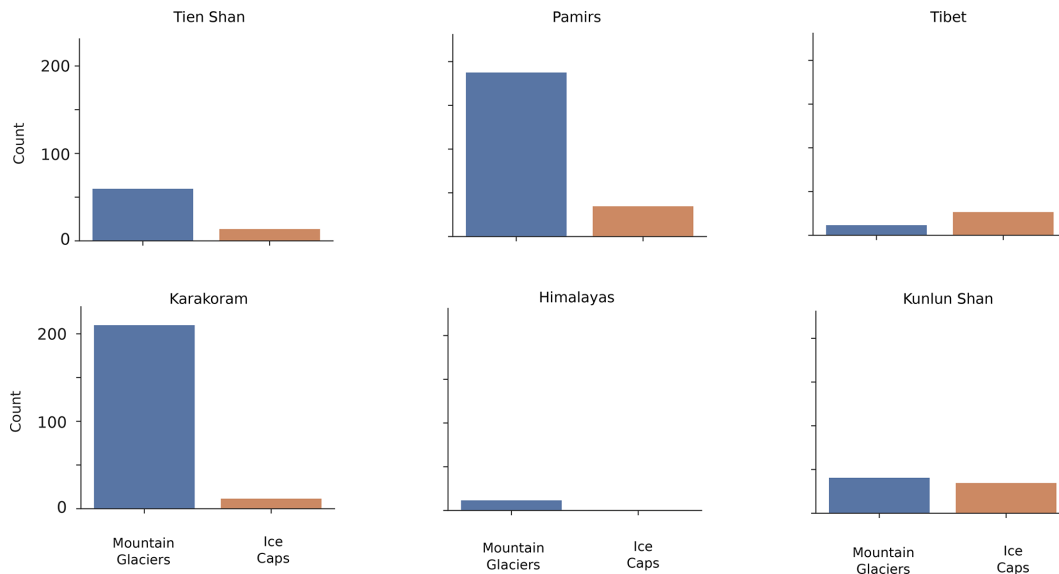
Figure 8. Distributions of surge-type glacier types for each of the greater HIMAP regions. Note that the Tibetan Mountains are the only region where ice cap outlet glaciers are more represented than mountain glaciers, with a ratio of 2.7.
