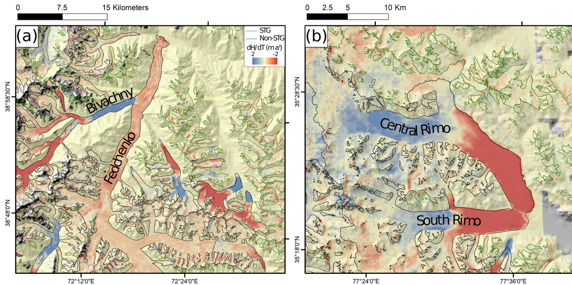
Figure 1. Examples of surface elevation change data used to identify surge-type glaciers. (a) Ice mass transfer associated with the surges of Bivachny Glacier, and other local glaciers, over the period 2010–2019 (data from Hugonnet et al., 2021). (b) Ice mass build-up in the reservoir zones of Central and South Rimo glaciers over the period 2000–2018 (data from Shean et al., 2020). Glacier outlines are from the Randolph Glacier Inventory V6.0 (RGI V6.0) (RGI Consortium, 2017).
