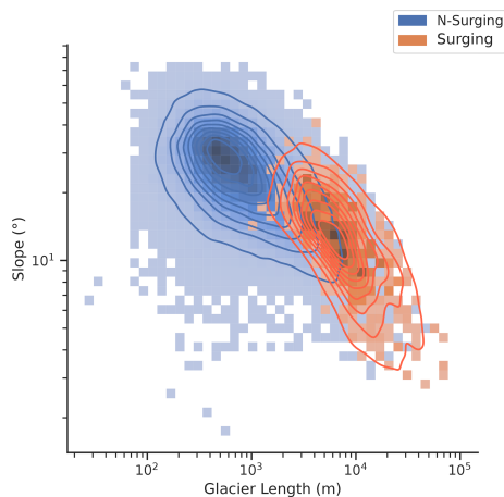
Figure 6. Length and mean slope for surging and non-surging glaciers in HMA. Due to the disparity in sample sizes between surge-type (666) and non-surging-type glaciers (more than 90 000), the length–mean-slope relationship is represented using a bi-variate histogram. Contour lines represent an estimate of the probability density, approximated using kernel density estimation.
