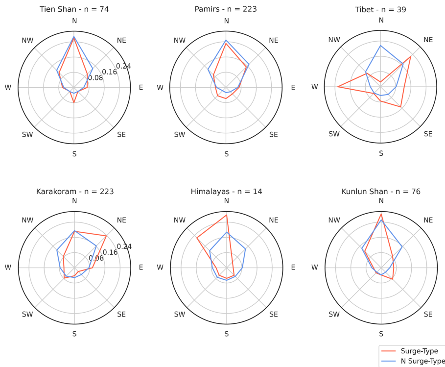
Figure 7. Aspect sector distribution for surging and non-surge-type glaciers for each greater study region per count. n refers to the number of surge-type glaciers per greater HIMAP region.
