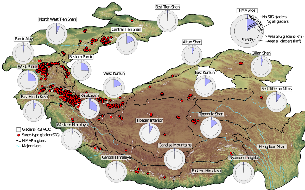
Figure 4. The distribution of surge-type glaciers (red dots) across HMA, identified by our multi-factor remote sensing approach. The number and area of surge-type glaciers within each HMAP region (Bolch et al., 2019), compared to the total glacier population, are also shown. Prominent but well-known clusters of surge-type glaciers are evident in the Pamirs and Karakoram, but our analysis has also confirmed and detected smaller clusters of surge-type glaciers across the Tibetan Plateau and Tien Shan CE4 .
