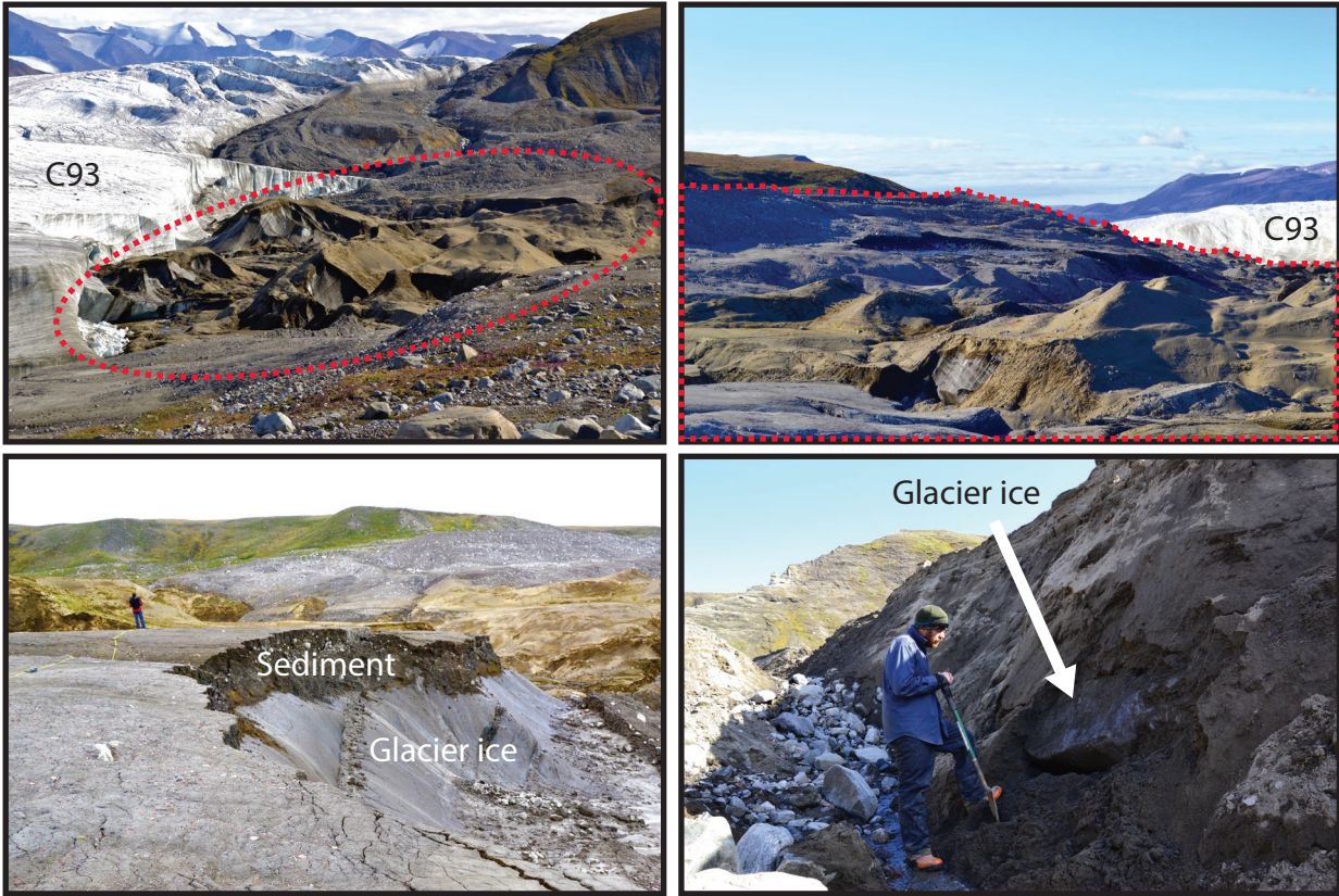
Figure S4: Burial of glacier ice at the margin of glacier C-93.
