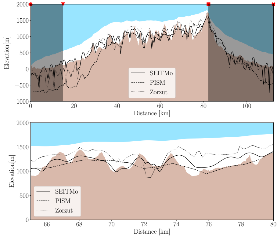
Figure 2. IOB cross section with the SIA inversion SEITMo, PISM, and Zorzut bedrocks, and red distance marks in the top as marked in Fig. 1. The outline of the ice cap is based on surface elevation from ArcticDEM and IOB ice thicknesses.
