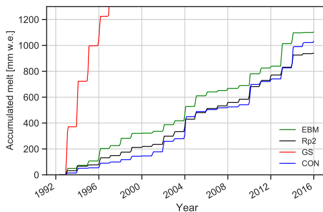
Figure 14. Cumulative melt in mm w.e. at Neumayer calculated by the energy balance model (EBM) of Jakobs et al. (2019) and Rp2, GS and CON.
