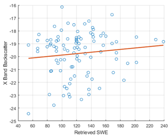
Figure 17: (a, left) 2D plot of sigma0 against the single variable of retrieved SWE at X band (b, right) 2D plot of sigma0 against the single variable of retrieved SWE at Ku band.
