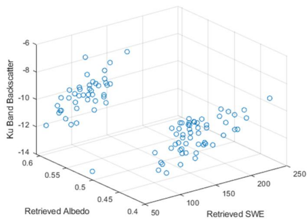
Figure 16: (a, left) 3-dimensional plot of the sigma0 when plotted against two variables at X band (b, right) 3-dimensional plot of the sigma0 when plotted against two variables at Ku band.
