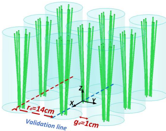
Figure 9: (a) Scattering from wheat plants are the radius of the circumscribing cylinder 6.5 cm, distance between the centres of 2 circumscribing cylinders is r_d = 14 cm, the closest distance between 2 circumscribing cylinders is g_d = 1 cm. Figure is adapted from Gu et al., 2021. (b) Transmission of microwave through wheat of different calculated using the hybrid method and the RTE vary with volume water content (VWC).
