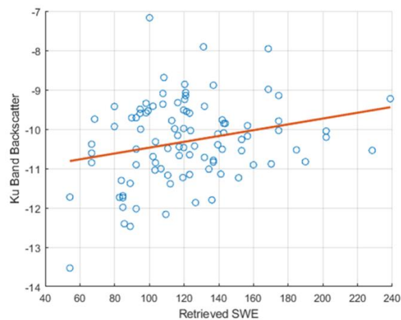
Figure 17: (a, left) 2D plot of sigma0 against the single variable of retrieved SWE at X band (b, right) 2D plot of sigma0 against the single variable of retrieved SWE at Ku band.
