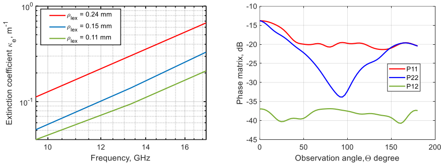
Figure 3: (a) Frequency dependence of the extinction coefficient from X- to Ku-band and (b) phase matrices at 13.3 GHz for different values of microstructure correlation length \rho_{\text{lex}} . Snow parameters are volume fraction f_v = 0.20 , aggregation parameter b = 1.2 , and correlation length 0.15 mm. P11 and P22 are co-polarized phase matrix elements and P12 is a cross-polarized phase matrix element.
