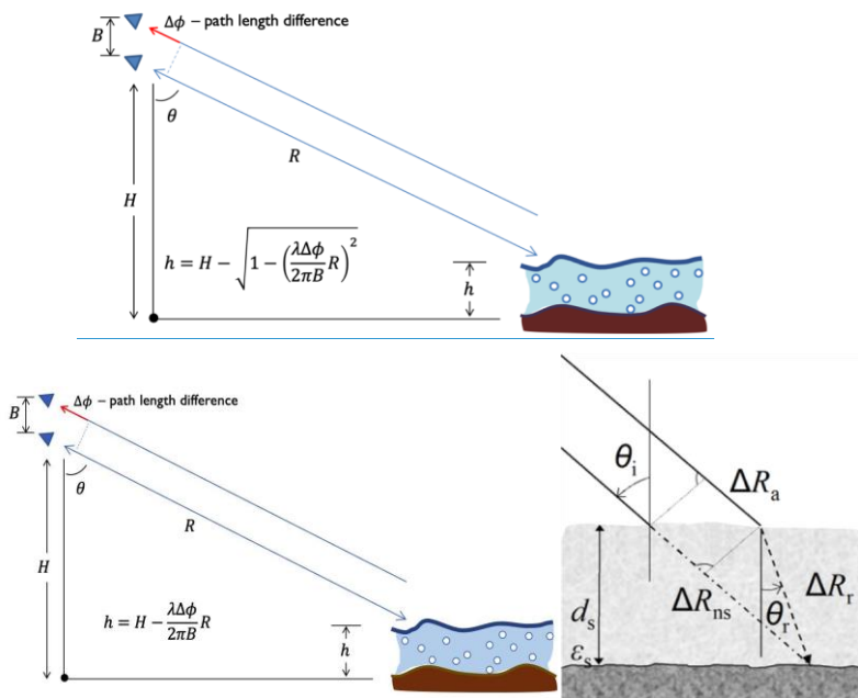
Figure 20: (A, left) Illustration of single-pass InSAR for mapping the snow surface. Using measured phase, \Delta\phi , simple trigonometric calculations are used to estimate the relative height, h , of the scattering phase center compared to the reference height, H . (B, right) When the phase center is below the snow surface, refraction in snow must also be taken into account. At low microwave frequencies (e.g. L-band) in dry snow, the phase center is often the snow-ground interface, and due to the slower electromagnetic velocity in snow, phase changes are related to changes in snow depth and density.
