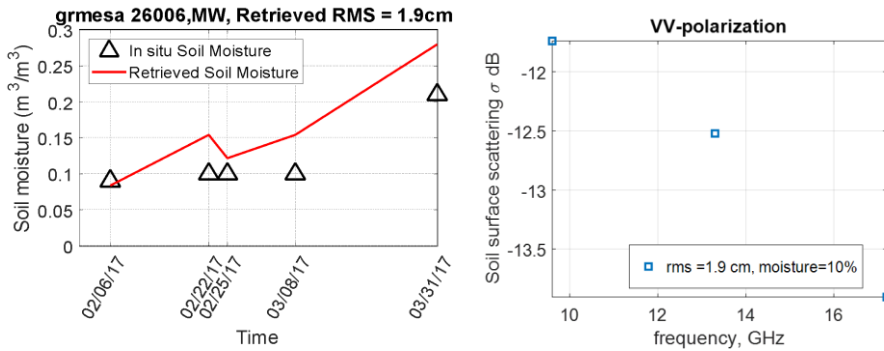
370 Figure 6 (a) Retrieval of soil moisture compared with in situ-measurements. The retrieved rms height is 1.9 cm. The retrieval is based on based on L-band UAVSAR data from SnowEx 2017 campaign. The measured soil moisture is from SnowEx 2017 campaign meteorological observations with a measured soil temperature of 0.6^\circ C . The location of the station is 39.03388^\circ N , 108.21399^\circ W with an elevation of 3033m. (b) Simulated surface scattering with snow attenuation from X- to Ku-band at VV polarization. Snow parameters are with depth of 54 cm, density of 183 kg m^{-3} , \langle \zeta \rangle = 1.2 mm , and b=1.2 . Blue marks are based on the SnowEx 2017 campaign data shown in (a). 375
