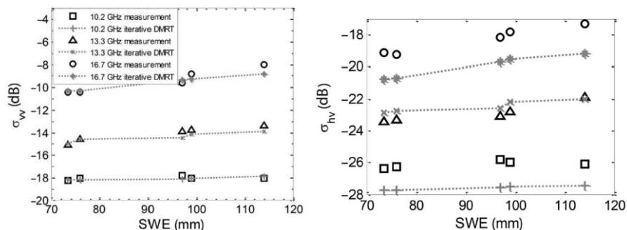
Figure 4: Comparison of the DMRT/bicontinuous media model using NoSREx 2010-2011 data backscatter against SWE for vertical co-pol (left) and cross-pol (right) at 10.2GHz, 13.3GHz, and 16.7GHz. Figures are adapted from Tan et al., 2015.
