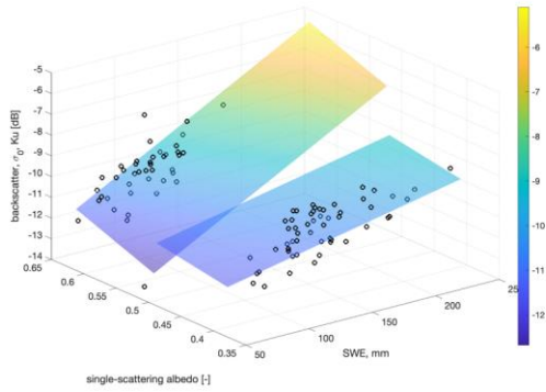
Figure 16: (a, left) 3-dimensional plot of the \sigma_0 when plotted against two variables at X-band (b, right) 3-dimensional plot of the \sigma_0 when plotted against two variables at Ku band (black circles) along with a linear least-squares fits of \sigma_0 to two variables SWE and single-scattering albedo (surfaces). The surface color indicates \sigma_0 value in dB.
