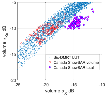
925 Figure 13: Canadian SnowSAR measurements compared with the Bic-DMRT LUT. Figure from Zhu et al. (2018).
