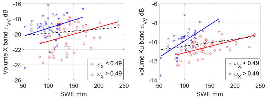
965 Figure 14: volume scattering of the Canada SnowSAR data as a function of SWE based on the retrieved scattering albedo \omega_X at (a, left) X-band and (b, right) Ku-band. Radar observations are from a single flight. A priori estimates are used to classify \omega_X into two classes. They are plotted by different coloured markers. The black dashed curve is the regression line of all Canada SnowSAR data. The blue and red solid curves are the regression lines for backscatter with \omega_X larger and smaller than 0.49, respectively. Figure from Zhu et al. (2018).
