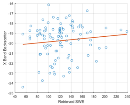
Figure 17: (a, left) 2D-dimensional plot of \sigma_0 against the single variable of retrieved SWE at X band (b, right) 2D-plot of \sigma_0 against the single variable of retrieved SWE at Ku band. The line represents a least squares linear fit between the two variables.
