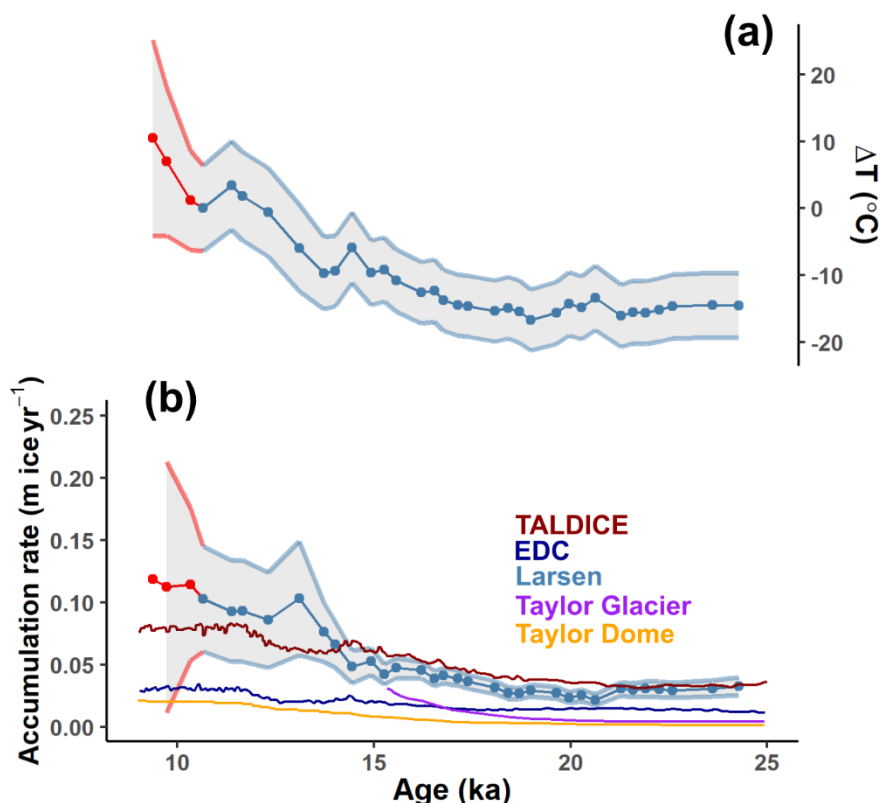
540 Figure 10. Reconstructed surface temperature and accumulation rate over the last glacial termination (Termination I). Accumulation rates of TALDICE and EDC are from Veres et al. (2013). Accumulation rates of Taylor Dome, and Taylor Glacier are from Baggenstos et al. (2018). The three youngest values of Larsen blue ice are rejected (red line) due to the large uncertainty in the \Delta age that translates into the possibility of negative accumulation rates and an unexpected 10.5 °C increase in ~1200 years. The \Delta T is a relative value to 10.6 ka BP; 10.6 ka BP is the youngest time period available. The uncertainty for the \Delta T and accumulation rate ( 1\sigma ) was estimated through error propagation.
