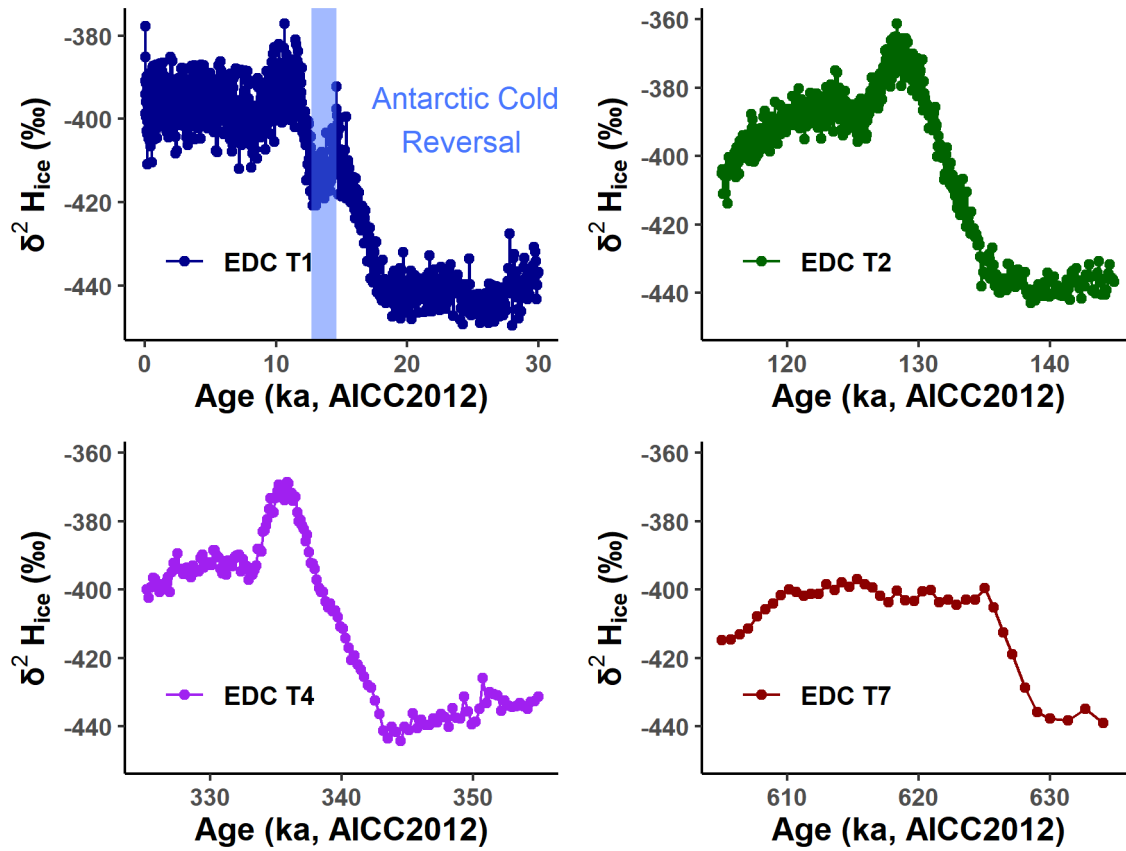
Figure A4. \delta^2\text{H}_{\text{ice}} records from EDC. \delta^2\text{H}_{\text{ice}} records for T1, T2, T4, and T7 on AICC2012 scale are from Bazin et al. (2013b). The blue vertical bar represents the time interval of the ACR (12.7–14.6 ka BP).
