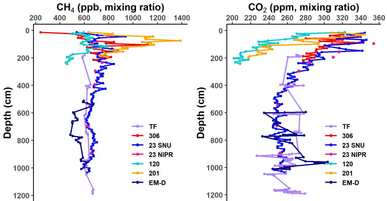
Figure A1. Vertical profiles of greenhouse gas concentrations at Larsen BIA ice cores. (a) \text{CH}_4 records. (b) \text{CO}_2 records. \text{CH}_4 was measured using wet extraction, while \text{CO}_2 was measured via both dry and wet extraction methods at SNU and NIPR, respectively. Results of TF core are from Jang et al. (2017).
