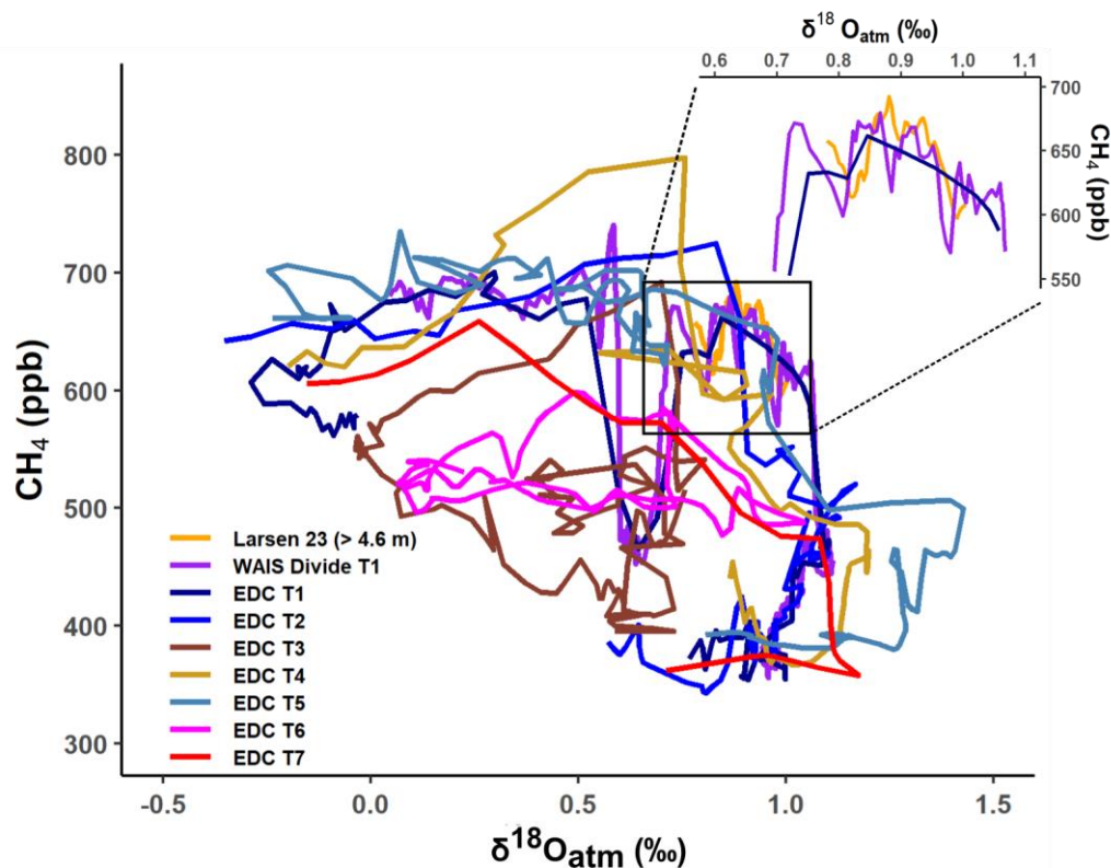
Figure 6. Comparison of \delta^{18}\text{O}_{\text{atm}} - \text{CH}_4 relationship in the Larsen ice core #23 with existing records over glacial Terminations. \delta^{18}\text{O}_{\text{atm}} and \text{CH}_4 data of WAIS Divide are from Severinghaus (2015) and Rhodes et al. (2017), respectively. \delta^{18}\text{O}_{\text{atm}} of EDC is from Landais et al. (2013) and Extier et al. (2018a). The \text{CH}_4 record of EDC is from Bazin et al. (2013d). The area within the black box is magnified to compare the Larsen #23 record with those from WAIS Divide T1 and EDC T1.
