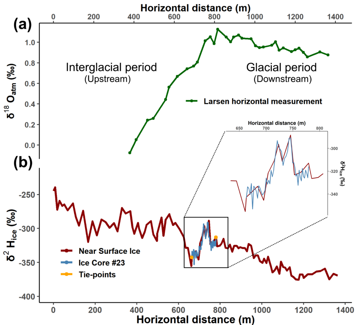
320 Figure 4. \delta^{18}\text{O}_{\text{atm}} and \delta^2\text{H}_{\text{ice}} records from Larsen BIA. (a) \delta^{18}\text{O}_{\text{atm}} from each ice core at a 1.95 m depth (horizontal measurement). The \delta^{18}\text{O}_{\text{atm}} of the horizontal measurement was gravity-corrected using Eq. (1). (b) \delta^2\text{H}_{\text{ice}} from near-surface ice (~5–10 cm depth surface ice samples and 10–30 cm depth ice core samples) and ice core #23. The surface ice record was matched with core #23 using two tie-points (orange dots), with a corresponding r^2 value of 0.86 ( p < 0.001 ).
