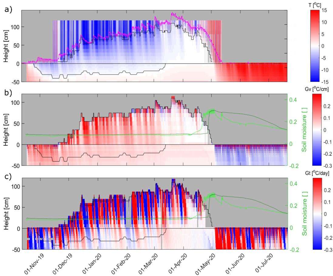
435 Figure 5: DTP systems deployed for snow and soil temperature measurements at a site in the East River (Colorado) watershed. The 440 DTP-inferred snow depth (above-ground black line) and soil frozen-layer thickness (below-ground black line) are overlaid on the DTP (a) temperature (T), (b) its vertical gradient (Gv) at each sampling time, and (c) the temporal change in temperature (Gt) after averaging the time series with a moving 24-hour time window. The pink line shows the snow depth from Butte SNOTEL station located 2 km away and at a 350 m higher elevation. The light and dark green lines indicate the soil moisture ( m^3/m^3 ) at 10 and 50 cm depth, respectively. Color scales have been cropped to the displayed minimum and maximum values in order to improve visualization.
