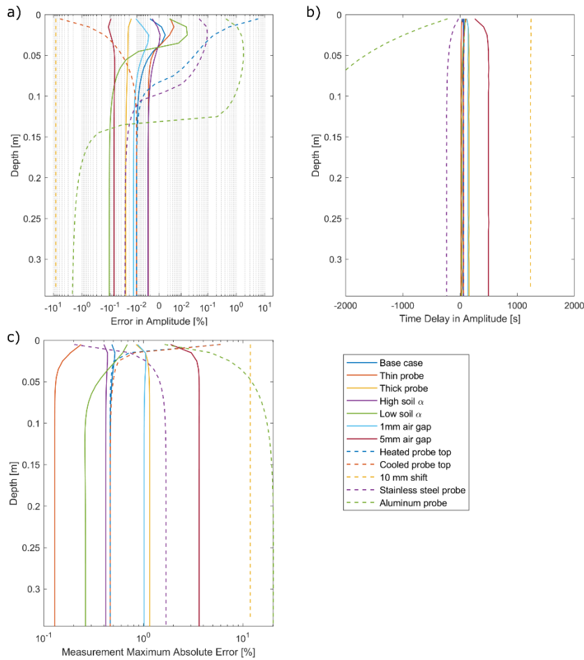
370 Figure 3: Influence of various probe characteristics and environmental factors on the accuracy of the DTP soil temperature measurements at various depth. (a) relative error in amplitude, (b) time delay in amplitude, and (c) measurement maximum percentage error relative to true amplitude at each depth.
