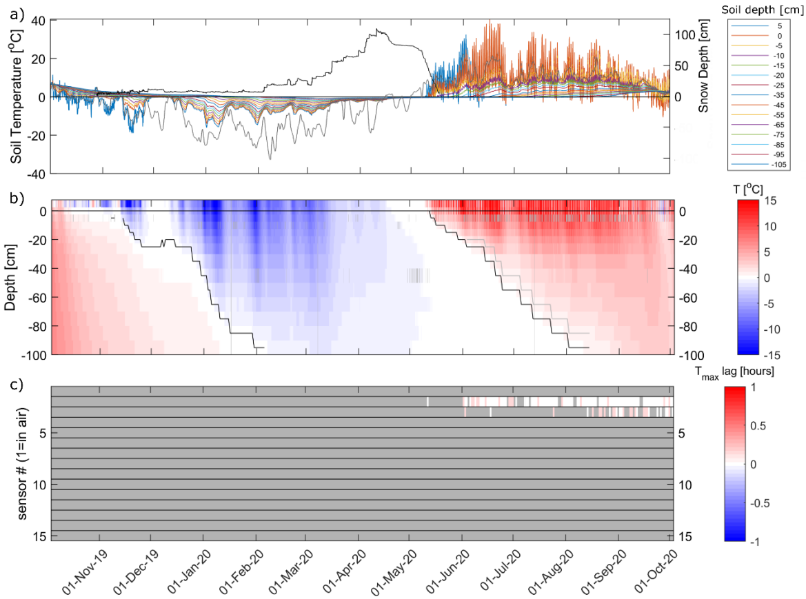
485 Figure 6: (a) soil temperature measurements from a DTP system in a discontinuous permafrost environment (Teller Road, mile 27, Nome, Alaska) with sensor from 5 cm above the surface to 105 cm depth, overlaid with the snow depth (black line) and daily average 490 air temperature (grey line) measured at a weather station located about 1 km away from the DTP system; (b) same DTP dataset with black lines indicating the inferred bottom and top of the frozen layer; (c) time delay smaller than 0.25 hour in daily minimum temperature between aboveground top sensor and each sensor along the probe, indicating the presence of an additional sensor positioned above the ground surface due to an upward displacement of the DTP system relative to ground surface. A ~2.5 cm displacement is flagged around June 3, and then August 20, which together led to a ~7.5 cm shift of the probe relative to the ground surface. This displacement is also qualitatively visible in (a) where the line representing above-ground temperature (initially at +5 cm) is successively overlapped by temperature data from the temperature sensors initially located at 0 and -5 cm depth. The grey line in (b) indicates the thaw layer thickness estimate after correction applied for the June 3 displacement.
