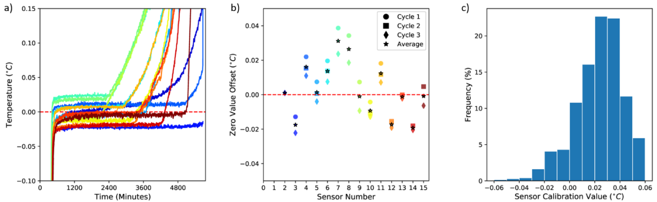
Figure 2: Sensor accuracy assessment. (a) 0°C curtain occurring during ice-to-water phase transition and observed by each sensor along the DTP probe, with offset related to sensor factory accuracy; (b) offset values observed by running the assessment approach three times with the same probe, indicating that the additional calibration improves the accuracy of the sensor to +/- 0.015°C (i.e., based on variations in three cycles), (c) distribution of the sensor factory offsets obtained from 846 sensors from 70 probes, with a mean of 0.02433°C and a standard deviation of 0.02095°C.
