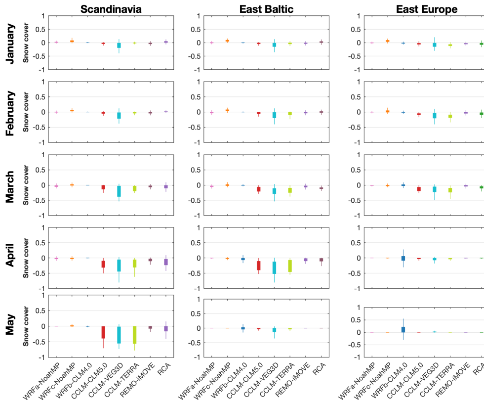
250 Figure 5: Impact of afforestation (FOREST-GRASS) on snow cover fraction simulated by the CORDEX FPS LUCAS models. The box plots indicate the spatial variability in the difference between the FOREST and GRASS experiments. Only differences that are statistically significant at the 95% confidence level are considered. Statistical significance was determined using the student t-test.
