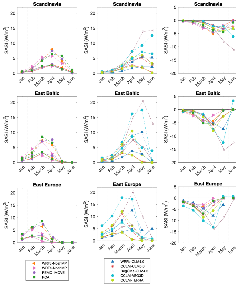
190 Figure 2: The first and second columns show the SASI values for GRASS (dashed lines) and FOREST (solid lines) experiments averaged over the three different regions shown in Figure 1. The nine simulations are divided into two different columns based on their values (high Vs low); the purpose of this separation is to ease interpretation of the results. The third column shows the impact of afforestation on SASI (FOREST – GRASS).
