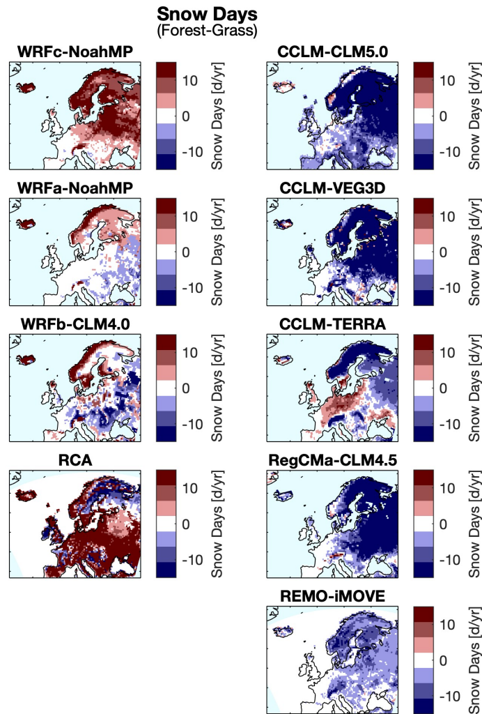
265 Figure 6: Impact of afforestation (FOREST-GRASS) on the number of snow days in the season, an indicator for the length of the snow season.
