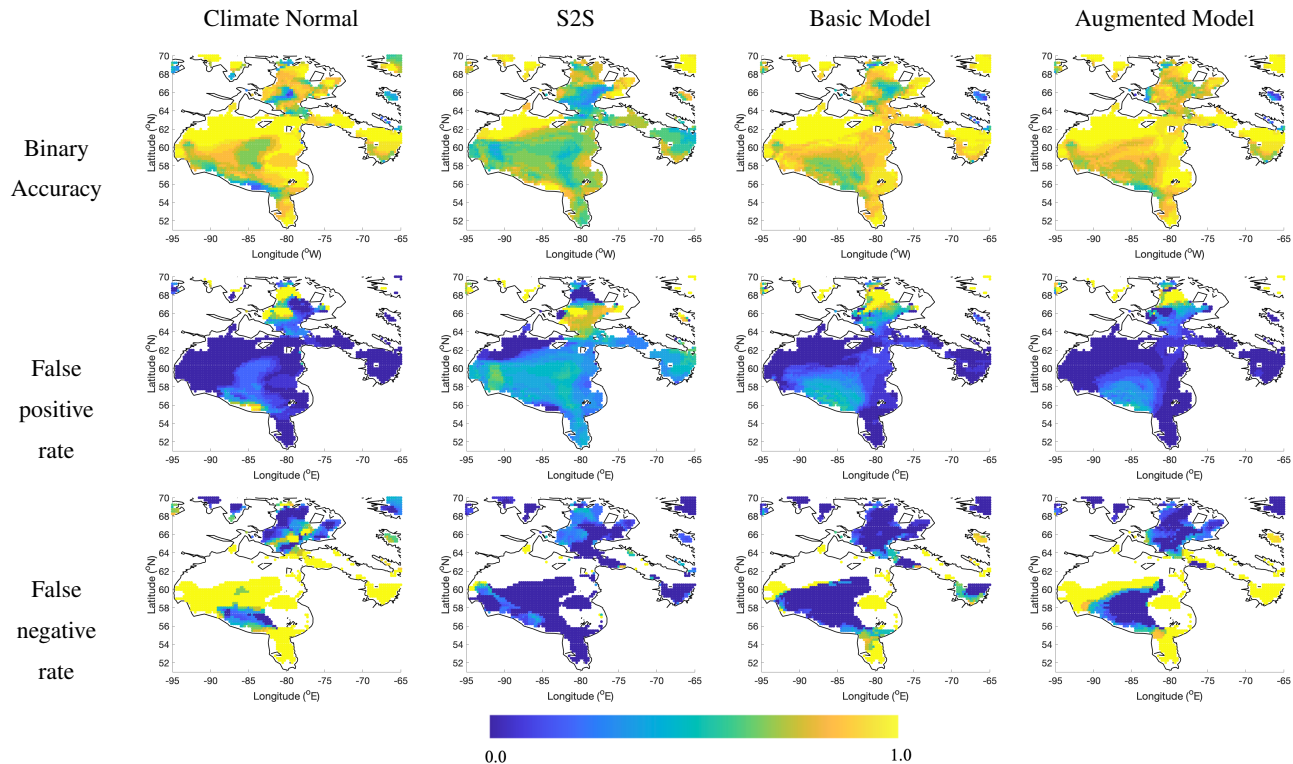
Figure 14. Binary accuracy, false positive rate and false negative rate calculated using data from forecasts launched between June 1-30, 2016 and June 1-30, 2017 at 30 lead days. These correspond to conditions from July 1-30, 2016 and July 1-30, 2017.
