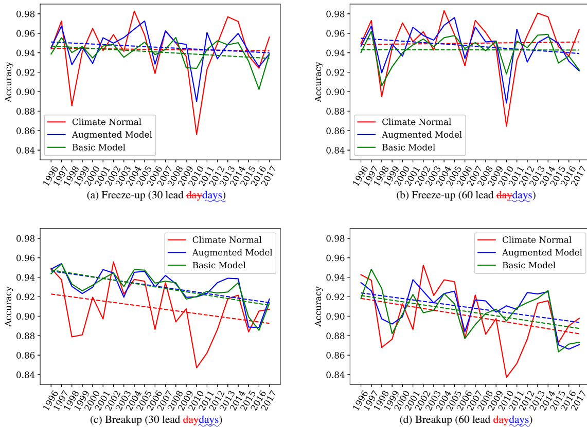
Figure 10. Accuracy of the Climate Normal, Basic model and Augmented model freeze-up and break-up predictions over the years at 30 and 60 lead daydays . Dashed lines show the trend.
