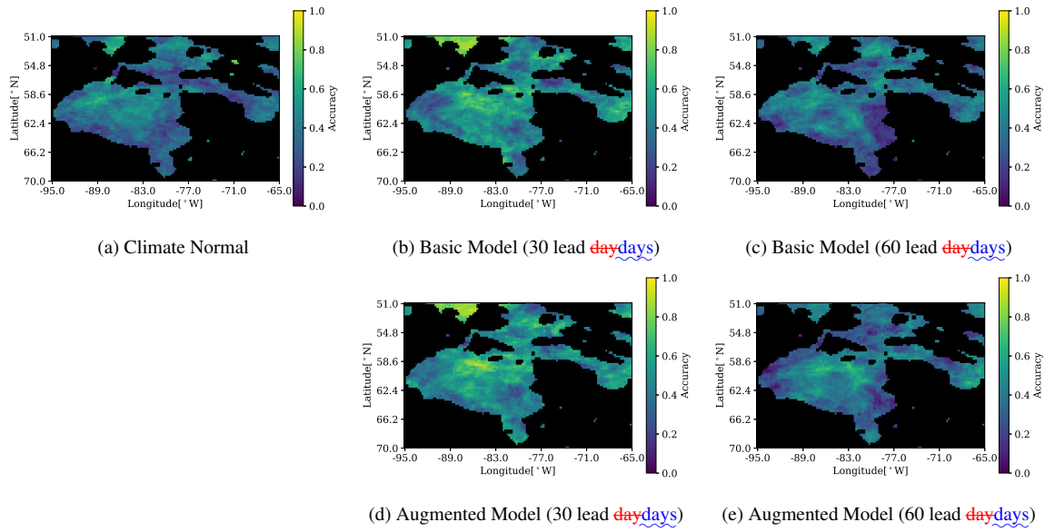
Figure 9. Accuracy of predicted break-up date within 7 days. Break-up dates are checked from May 1st to July 31st. The 7-day window is chosen to match to definition used by the Canadian Ice Service.
