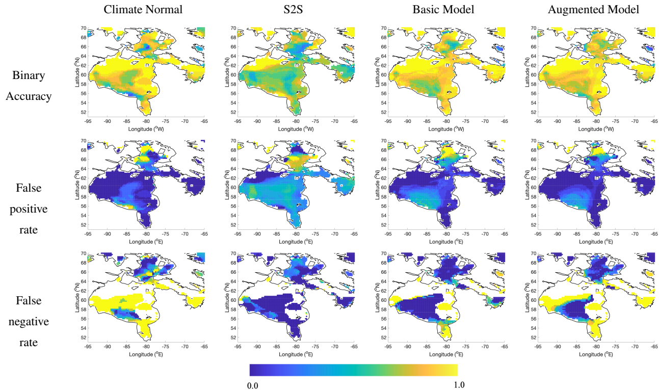
Figure 14. Comparison of forecasting approaches for Binary accuracy, false positive rate and false negative rate calculated using data from forecasts launched between June 1-30, 2016 and June 1-30, 2017 at 30 lead days. These correspond to conditions from July 1-30, 2016 and July 1-30, 2017.
