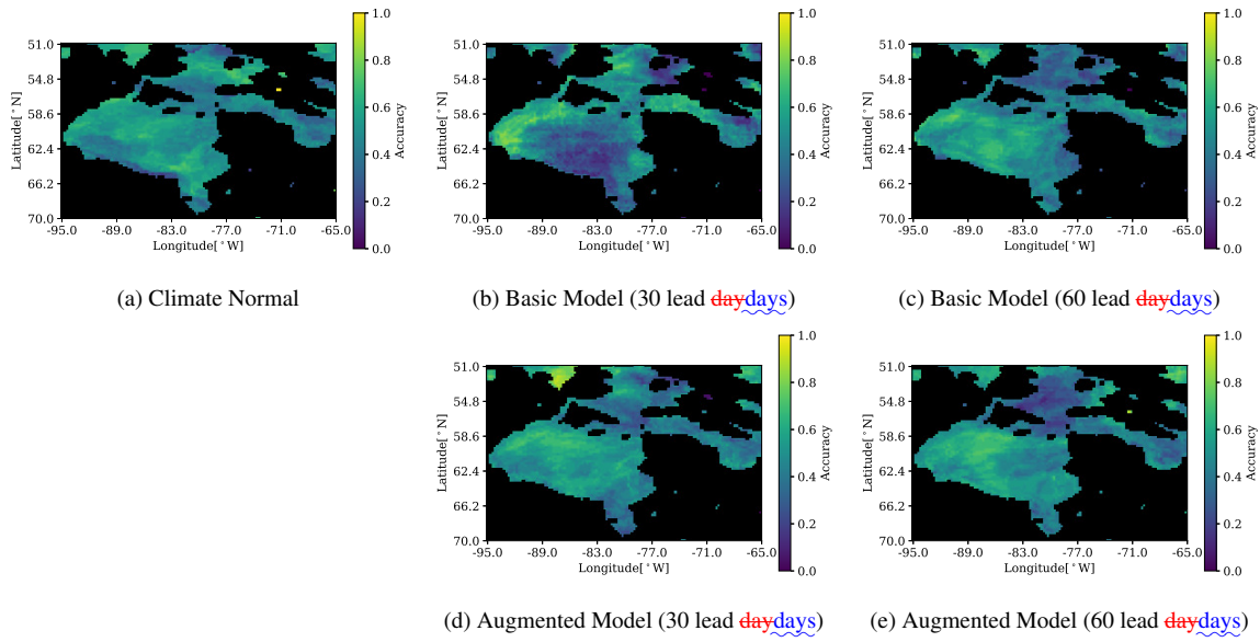
Figure 8. Accuracy of predicted freeze-up date within 7 days. Freeze-up dates are checked from October 1st to January 31st. The 7-day window is chosen to match to definition used by the Canadian Ice Service.
