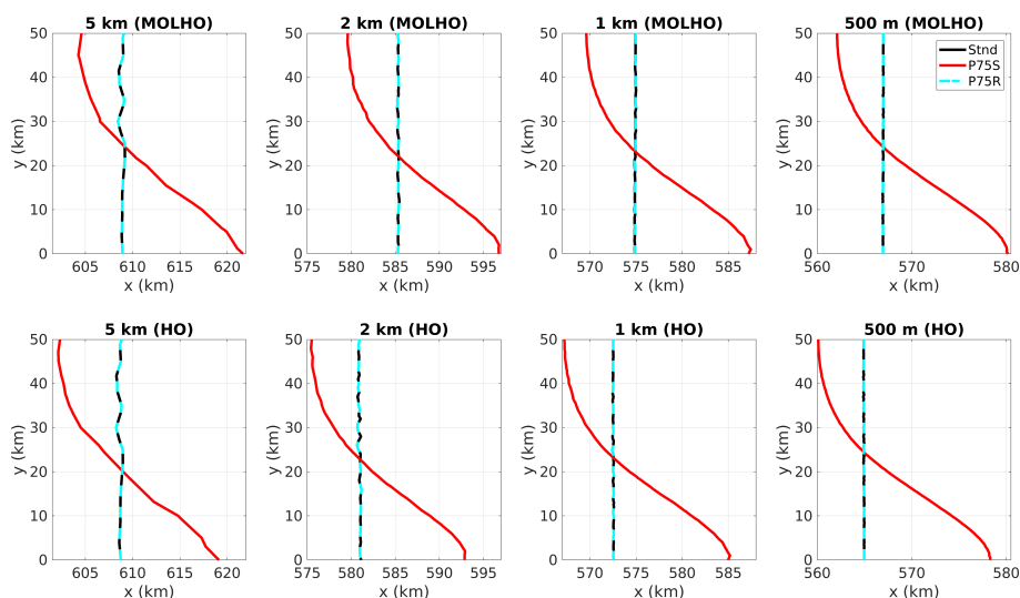
Figure 5. Grounding line positions of the MISIMP3D experiments obtained with different mesh resolutions. Black lines are the steady state grounding line positions (Stnd). Red lines are the positions obtained after 100 years of basal friction perturbation (P75S). Dashed blue lines are the new steady state grounding line positions obtained after resetting the friction coefficient to its original value (P75R).
