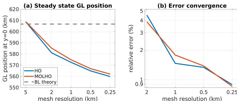
Figure 4. MISIMP3D experiment: steady state positions (a) and estimated error convergence (b) of the grounding line (GL) at y = 0 obtained with different mesh resolutions using HO and MOLHO. The error convergence is estimated using Eq. 24. For comparison, the steady state grounding line position predicted by the Boundary Layer (BL) theory that is based on SSA model is also shown.
