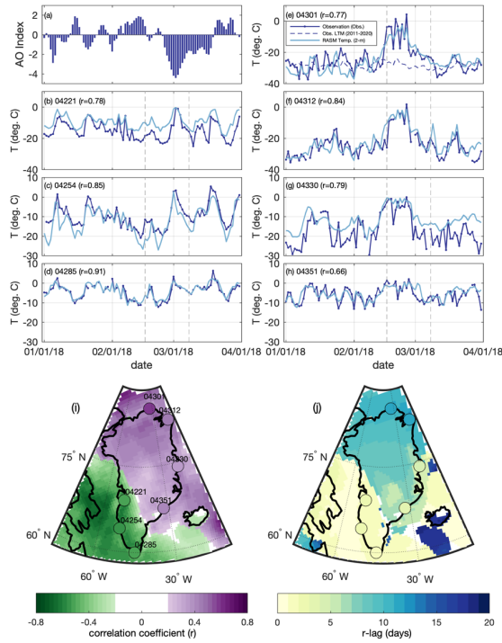
Figure 3. (a) The observed daily AO index and (b)-(h) the daily mean near-surface air temperature ( T , °C; blue ) during January-March 2018 from the selected weather stations around Greenland as shown in (i) and (j) as circle markers. The RASM daily 2-m air temperature ( light blue ) is from the nearest grid cell and the observed long-term daily mean (LTM, 2011-2020; blue-dashed ) is only at Station 04301. The correlation coefficient ( r ) is statistically significant ( p < 0.05 ) between the observed and the simulated air temperature is shown in the upper-left. The vertical dashed lines indicate the start and end dates of the 2018 winter polynya period. The spatial maps show (i) the maximum correlation coefficients and (j) their lagged time-scales (days) between the AO index and the RASM air temperature. Note that grid cells not statically significant ( p > 0.05 ) are indicated as white. The color-scale of the markers quantifies the relationship between the AO index and the observed air temperature at each weather station.
