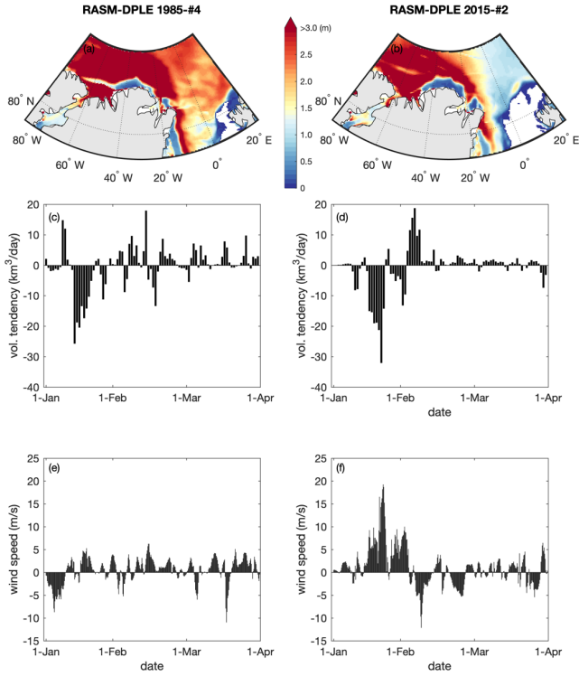
Figure 10. Sea ice thickness (SIT, m), sea ice dynamic volume tendency (DVT, \text{km}^3/\text{day} ) for the northern Greenland region (see Fig. 4a), and north(positive)-south(negative) wind component (m/s) during winter months from the ensemble member #4 in the 1985-initialized run and the ensemble member #2 in the 2015-initialized run: SIT on (a) 22 January 1988 and (b) 14 January 2024, daily DVT in January-March of (c) 1988 and (d) 2024, and six-hourly north-south wind in January-March of (e) 1988 and (f) 2024.
