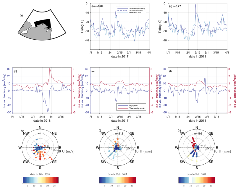
Figure 4. The observed daily near-surface air temperature ( T , °C; blue) from Station 04301 (Cape Morris Jesup as ●) in (a) and the RASM daily 2-m air temperature (light blue) from the nearest grid cell during January-March of (b) 2017 and (c) 2011; the observed long-term daily mean (LTM, 2011-2020; blue-dashed). The correlation coefficient ( r ) between the observed and the simulated air temperature is shown in the upper-left. Time rate of change of the RASM daily sea ice volume ( \text{km}^3/\text{day} ) due to thermodynamic (red) and dynamic (blue) tendency during January-March of (d) 2018, (e) 2017, and (f) 2011, spatially integrated for the black-shaded area in (a). Wind rose plots of 3-hourly wind data at Station 04312 (Station Nord as ▲) during February of (g) 2018, (h) 2017, and (i) 2011: wind speed ( U , m/s) and direction. The missing data are indicted as white in each color bar.
