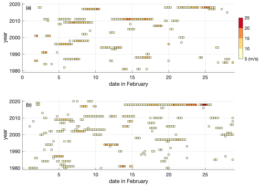
035 Figure 8. The northward wind component greater than 5 m/s from the RASM hindcast simulation during February of 1980-2020 at the nearest grid to (a) Station 04312 (Station Nord) and (b) Station 04301 (Cape Morris Jesup). Each square represents the six-hourly surface wind and its color indicates a magnitude of wind speed.
