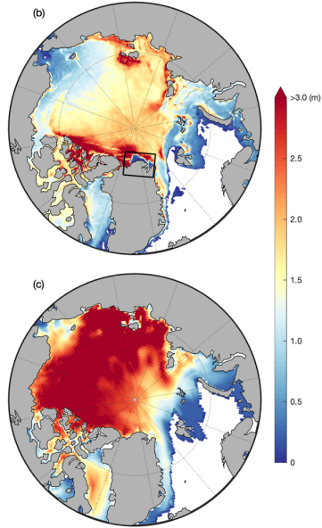
Figure 1: (a) The Visible Infrared Imaging Radiometer Suite (VIIRS) Nighttime Imagery (Day/Night Band, Enhanced Near Constant Contrast) over the northern Greenland on 25 February 2018 (adapted from NASA Worldview at https://worldview.earthdata.nasa.gov ) and sea ice thickness from (b) the RASM hindcast simulation as well as (c) CFS version 2 reanalysis over the Arctic on 25 February 2018. The rectangular box indicates the polynya area.
