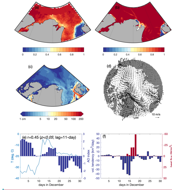
040 Figure 9. Mean sea ice concentration (NASA Team algorithm) on 15 December 1986 over the northern Greenland region from (a) the Nimbus-7 SMMR and (b) the RASM hindcast simulation. (c) Monthly integrated sea ice melt (top, lateral, and basal) for December 1986 and (d) near-surface (at 10 m) wind fields on 12 December 1986 from the RASM hindcast simulation. (e) RASM daily near-surface air temperature (light blue) from the nearest grid cell to Station 04301 (Cape Morris Jesup) and daily AO index (blue) in December 1986. The correlation coefficient ( r ) between the AO index and the simulated air temperature is shown in the upper-left. (f) Time rate of change of the RASM daily sea ice volume ( \text{km}^3/\text{day} ; blue) due to dynamic tendency during December 1986, spatially integrated for the region shown in Fig. 4a. Daily mean net turbulent (sensible and latent) heat flux ( \text{W}/\text{m}^2 ; red) is also shown over the same region where sea ice thickness is less than 10 cm from the RASM hindcast simulations. The negative values indicate loss from the region.
