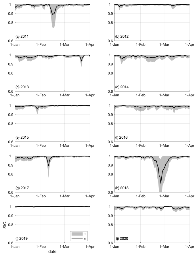
030 Figure 7. (a)-(j) Satellite-derived (NASA team algorithm) daily mean sea ice concentration (SIC, \mu ; black) for the northern Greenland region (see Fig. 4a) during January-March from 2011 to 2020. The grey shading depicts one standard deviation ( \sigma ; gray) from the mean.
