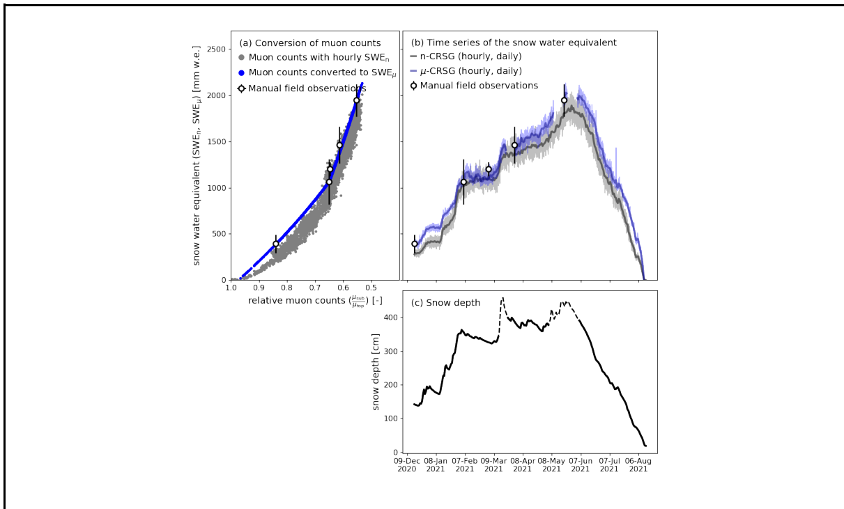
Fig. 3 From muon count rates to SWE. Panel (a) shows the relative muon count rates plotted against SWE that is measured by the n-CRSG (grey dots) and measured manually (white dots). Blue dots represent the SWE that is directly inferred from the relative muon count rate with the conversion function given in Eq.6. Panel (b) shows the time series of SWE inferred from neutron counts (grey) and muon counts (blue) at a daily resolution. Light grey and light blue represent hourly observations of the n-CRSG and \mu -CRSG, respectively. Panel (c) shows snow depth measured at the site (solid line) with data gaps that were complemented from a nearby high-altitude station (dashed line).
