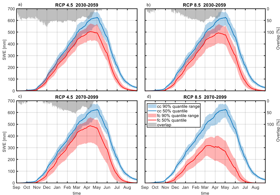
330 Figure 7. Areal mean seasonal SWE development under current (cc) and future climate (fc) for different emission scenarios and time horizons. Plotted are the 5, 50, 95 percentiles of climate period mean values stemming from 50 (current climate) and 500 climate periods (future climate with 50 realizations of 10 climate models). The overlap indicates how much of the current climate natural variability is overlaid by the future climate uncertainty range.
