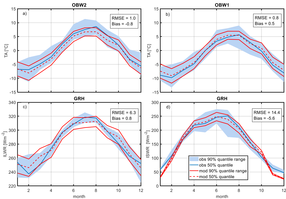
Figure 3. Monthly mean values for (a) air temperature (TA) at the stations OBW2 and (b) OBW1, (c) incoming longwave radiation (ILWR) and (d) incoming shortwave radiation (ISWR) at station GRH. Plotted are 5, 50 and 95th percentiles of observations in blue of 8 years (GRH) and 20 years (OBW1, 2), and modelled data in red of 1500 years. RMSE and Bias are calculated for 50 th percentiles.
