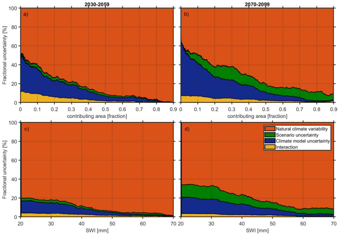
525 Figure 12. Same as Fig. 11c and d for the exceedance probability of the variables ‘contributing area’ and contributing-area averaged SWI using criterion 3 (cp. Figs. 8 and 11).
