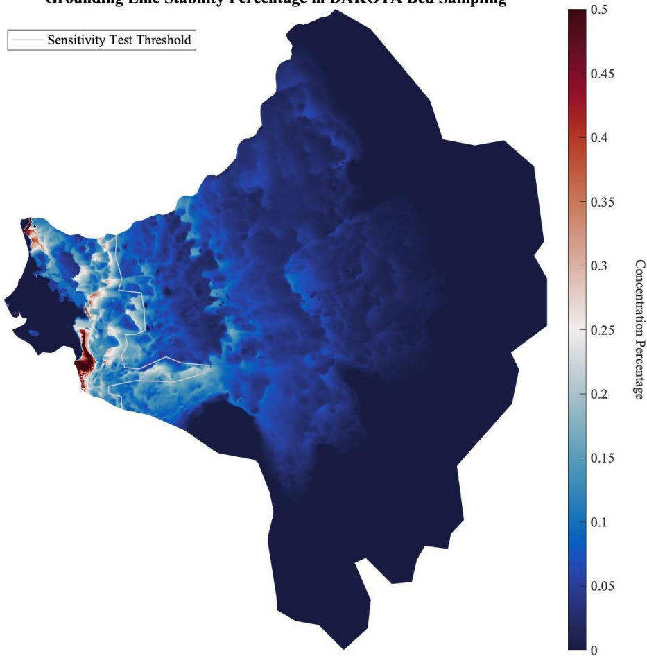
Fig. S4: The probability of the grounding line's location lying on an element during a 200-year projection forced with extreme (1.8 times present day) ice shelf basal melting rates, as determined from random sampling of bedrock topography within a prescribed 3% error (described in Sect. 5.1 and portrayed in Fig. 5, blue line). Grounding line positions are calculated every 10 years for all of the 300 forward simulations in the ensemble, resulting in 6000 different grounding line configurations. Plotted is the concentration of all 6000 grounding line positions as a percentage of the amount of times the grounding line is located in an individual location. A threshold line (gray) is drawn to segregate the percentages at or above 20%. This figure is the determining factor for analyzing and testing relevant regions in our sensitivity test (Sect. 5.2).
