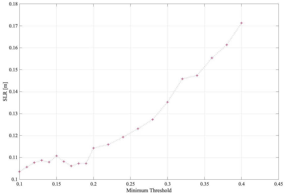
Fig. S5: SLR contribution as a function of positive perturbations in bedrock topography. Perturbations are only made at points that fall above a minimum threshold of grounding line concentration probability derived from the bedrock sampling \times 1.8 melt ensemble (Fig. S4). We use this figure to determine what grounding line concentrations we should set our limits to when deciding what regions of bedrock topography in Fig. S4 are most relevant to investigate as significant pinning points. In this case, we determine that 20% is an appropriate threshold.
