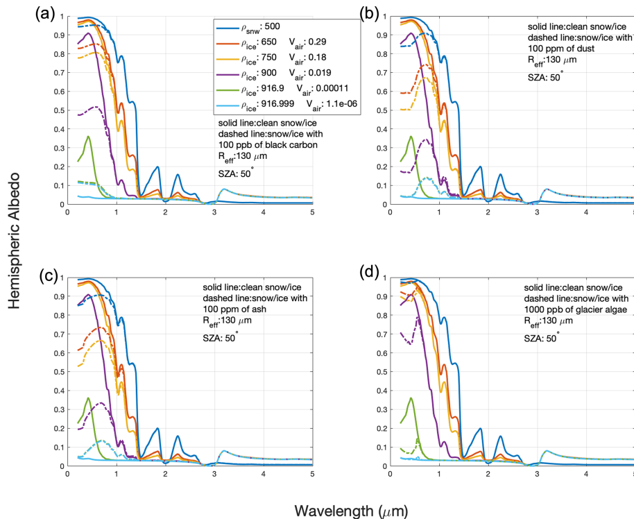
Figure 7. Model spectral albedo of various snow and ice surfaces with LACs. The model configuration of LAC-free surfaces (solid lines) is outlined in Fig. 3 (FS3), and spectral curves are for a snow grain/air bubble radius of 130\ \mu\text{m} . Dashed lines are the same with the addition of LACs. (a) Spectral albedo of various snow and ice media with and without 100 ppb of uncoated black carbon. (b) As in panel (a) but with and without 100 ppm of volcanic ash with a radius of 1.25\text{--}2.5\ \mu\text{m} . (c) As in panel (a) but with and without 100 ppm of GrIS dust species with a radius of 1.25\text{--}2.5\ \mu\text{m} . (d) As in panel (a) but with and without 1000 ppb of dry glacier algae with a length of 40 and width of 4\ \mu\text{m} (Cook et al., 2020).
