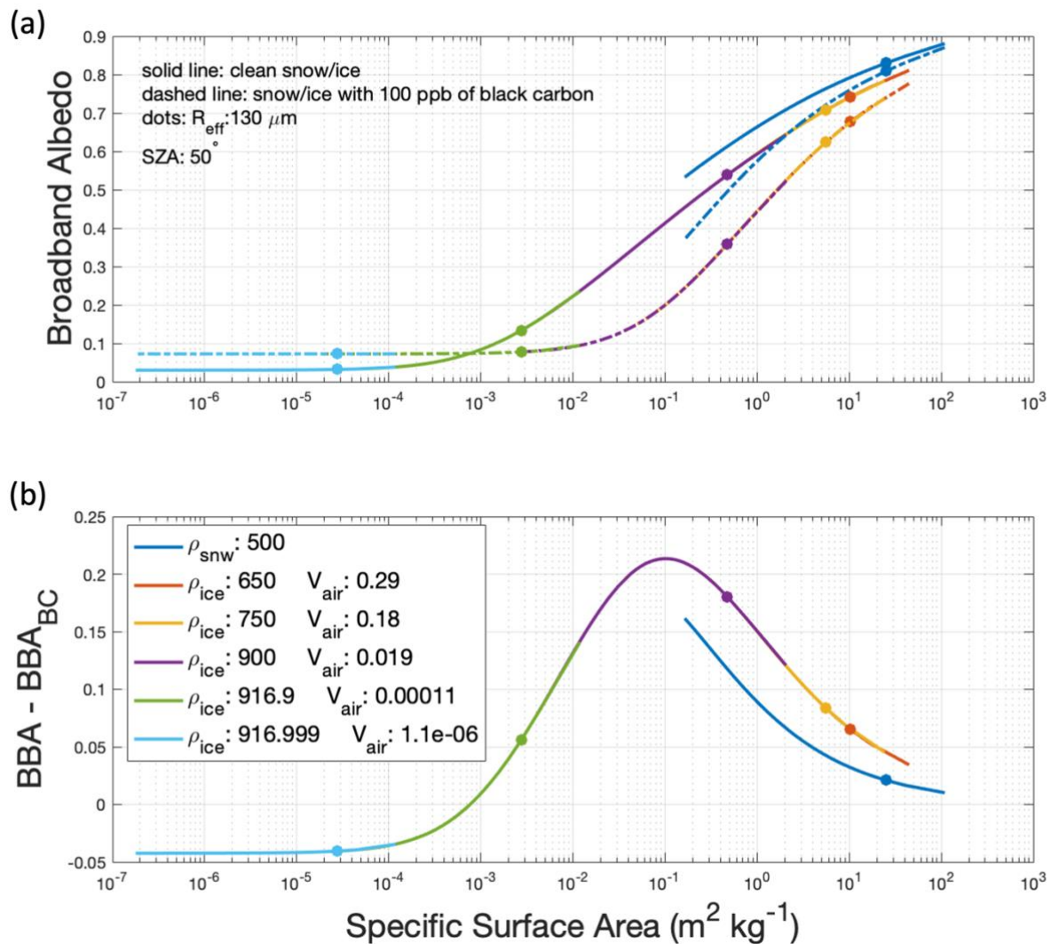
725 Figure 8: The impact of black carbon on snow and ice BBA as a function of SSA. Model configuration is the same as Figure 7a. Dots indicate where the radius of the snow grain and air bubbles is 130 \mu\text{m} . A) Broadband albedo as a function of specific surface area, solid lines indicate clean snow / ice and dashed lines indicate snow / ice with 100 ppb of black carbon. B) The broadband albedo impact of black carbon shown as the difference between the sold and dashed lines in A.
