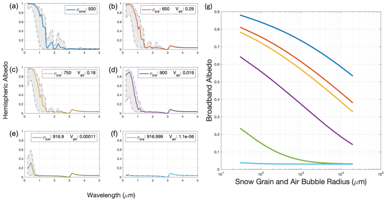
695 Figure 3: A-F Spectral albedo as a function of wavelength, snow or ice density, and the ice volume fraction of air. Shading indicates the full range of clean snow or ice albedo as a function of snow grain or air bubble radius, and the spectral albedo for an ice grain/air bubble with an effective radius of 180 \mu\text{m} is indicated by the colored line. Panel a is a snow layer, all the other panels are ice layers. The radius ranges from 30 \mu\text{m} (the highest albedo curves) to 20,000 \mu\text{m} (the lowest albedo curve). The model parameters are included in Table A1. G ) Broadband albedo (BBA) as a function of grain size (log scale). Each BBA and SSA corresponds to a spectral curve in A with a particular snow grain or air bubble radius.
