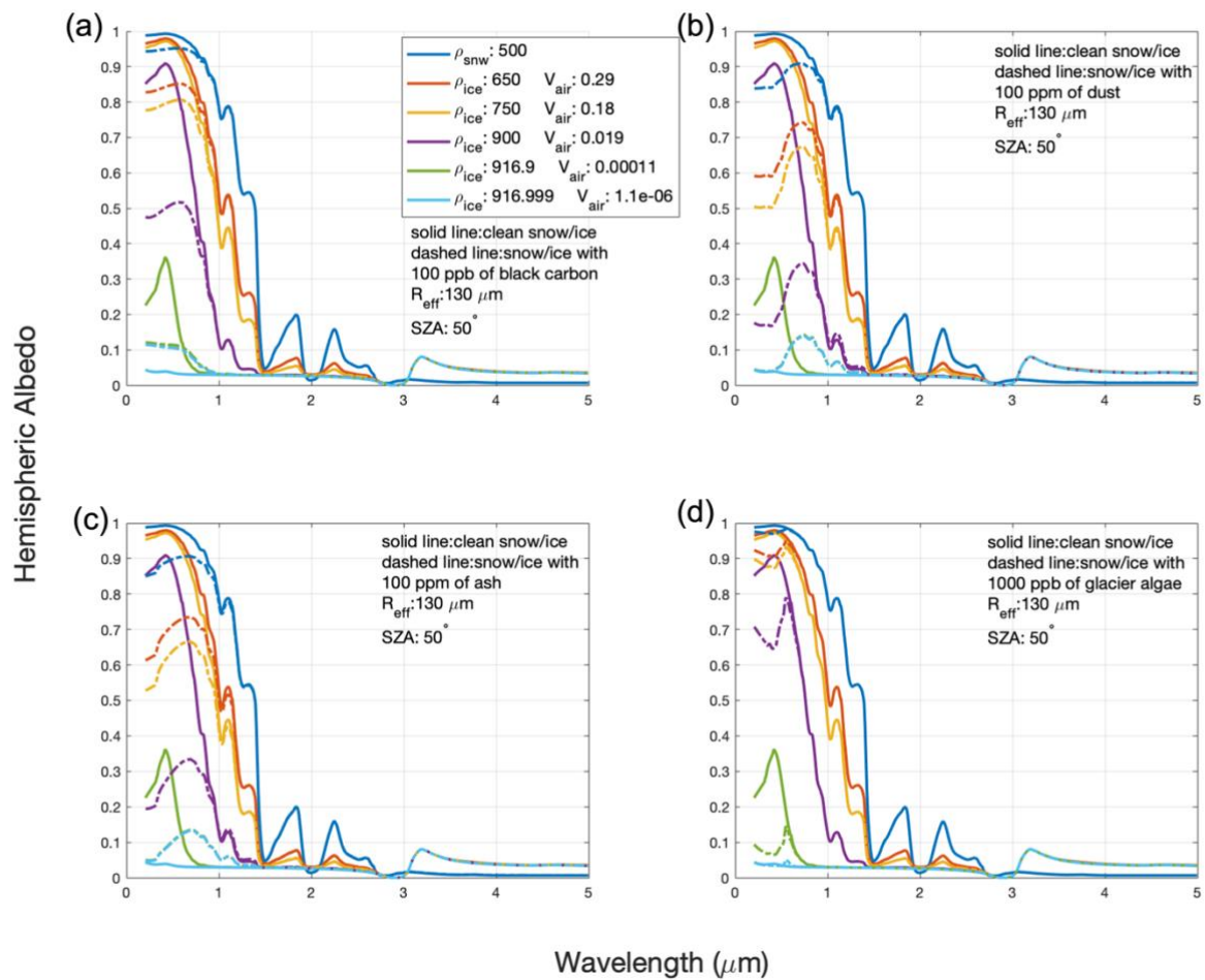
720 Figure 7: Model spectral albedo of various snow and ice surfaces with LAC. Model configuration of LAC-free surfaces (solid lines) is outlined in Figure 2 and spectral curves are for a snow grain/air bubble radius of 130 \mu\text{m} . Dashed lines are the same with the addition of LAC. A) Spectral albedo of various snow and ice media with and without 100 ppb of uncoated black carbon. B) As in (A), but with and without 100 ppm of volcanic ash with a radius of 1.25 - 2.5 \mu\text{m} . C) As in (A), but with and without 100 ppm of GrIS dust species with a radius of 1.25 - 2.5 \mu\text{m} . D) As in (A), but with and without 1,000 ppb of dry glacier algae with a length of 40 \mu\text{m} and width of 4 \mu\text{m} (Cook et al., 2020).
