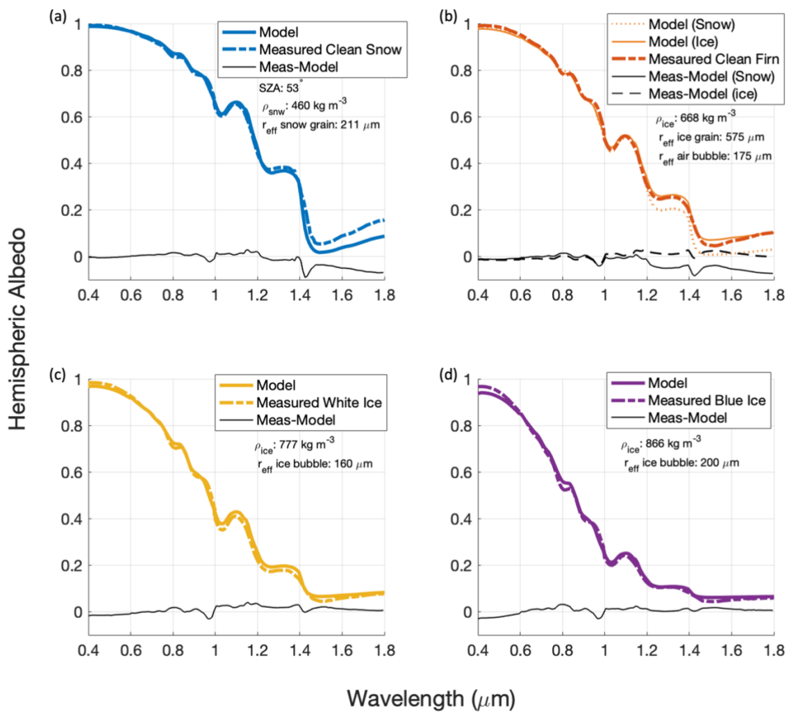
740 Figure 11: Spectral albedo measured by Dadic et al. (2013) compared to SNICAR-ADv4 modeled spectral albedo. The model parameters are tightly constrained with quantitative measurements made by Dadic et al. (2013).
