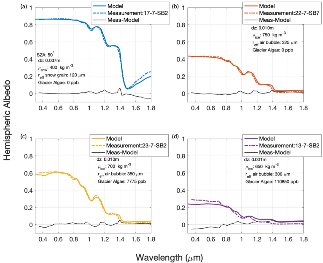
735 Figure 10: Spectral albedo measured by Cook et al. (2020) compared to SNICAR-ADv4 modeled spectral albedo. Model parameters are loosely based on qualitative snow and ice properties and quantitative algal cell measurements.
