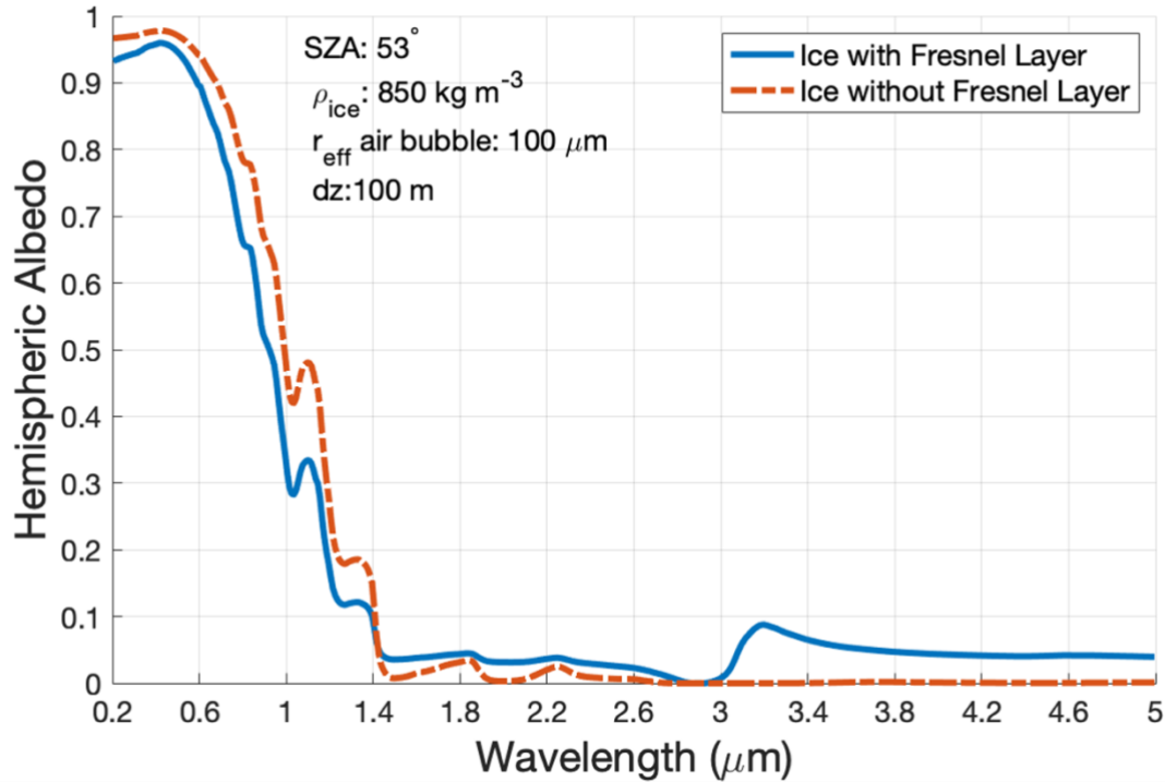
710 Figure 5: Ice spectral albedo with and without the refractive boundary between air and ice.
