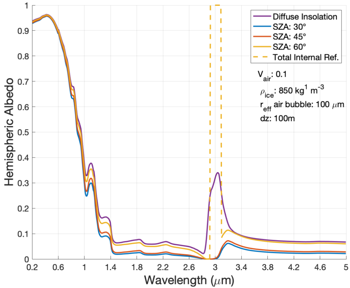
690 Figure 2: Spectral albedo with varying SZA. Each line indicates the spectral albedo simulated by SNICAR-ADv4 with a different SZA. The purple line shows the spectral albedo for the ice layer under diffuse light conditions and the dashed line indicates where total internal reflection occurs on the smooth ice surface.
