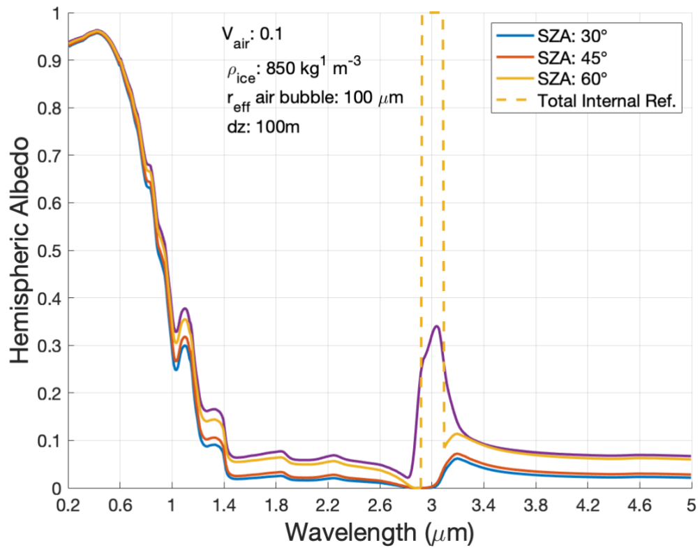
Figure 2: Spectral albedo with varying SZA
