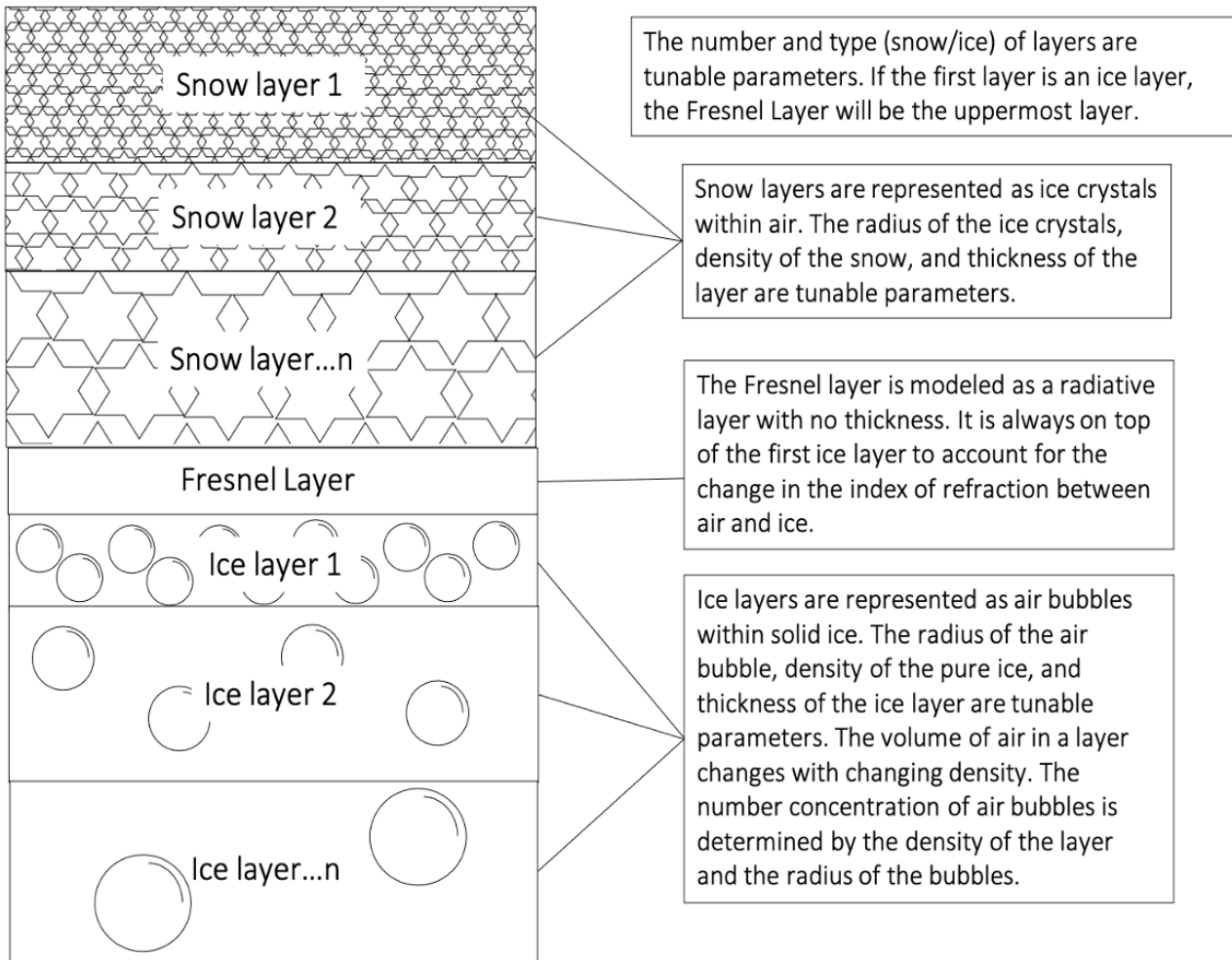
685 Figure 1: Model schematic of an example column of snow and ice.
