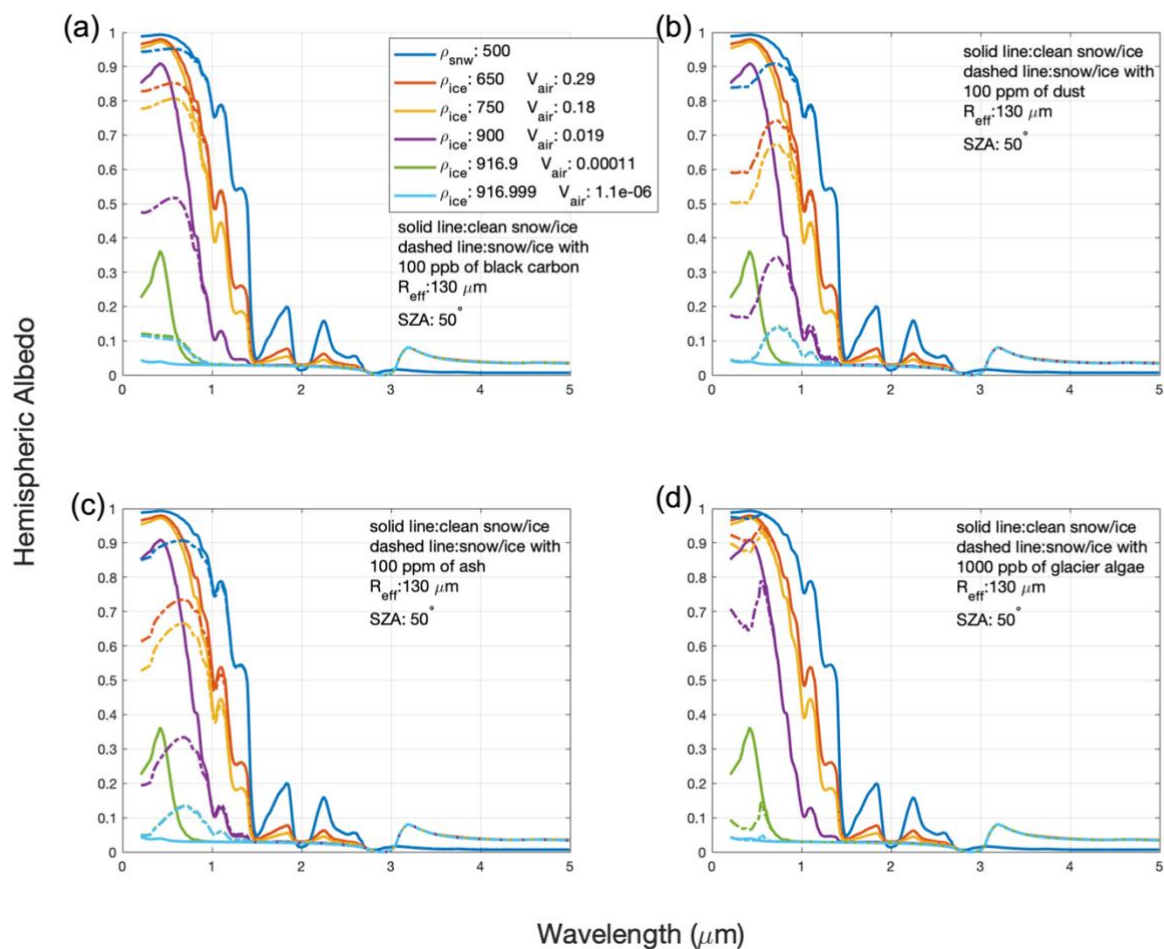
715 Figure 7: Model spectral albedo of various snow and ice surfaces with LAC. Model configuration of LAC-free surfaces (solid lines) is outlined in Figure 2 and spectral curves are for a snow grain/air bubble radius of 130 \mu\text{m} . Dashed lines are the same with the addition of LAC. A) Spectral albedo of various snow and ice media with and without 100 ppb of uncoated black carbon. B) As in (A), but with and without 100 ppm of volcanic ash with a radius of 1.25 - 2.5 \mu\text{m} . C) As in (A), but with and without 100 ppm of GrIS dust species with a radius of 1.25 - 2.5 \mu\text{m} . D) As in (A), but with and without 1,000 ppb of dry glacier algae with a length of 40 \mu\text{m} and width of 4 \mu\text{m} (Cook et al., 2020).
